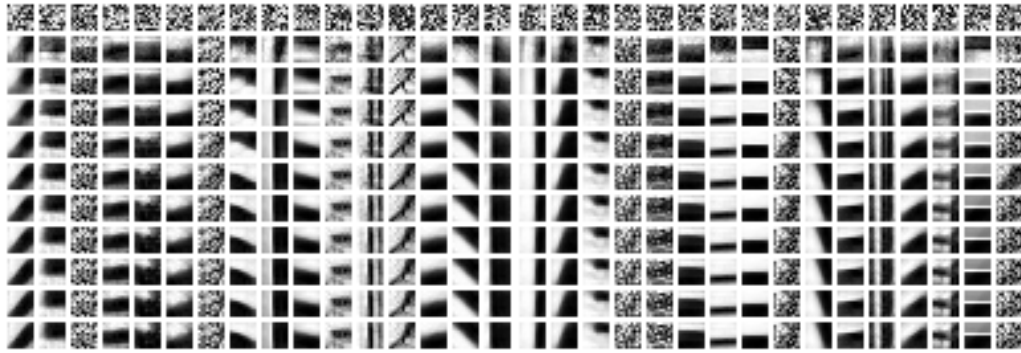
Figure 4.20: The evolution of the 32 templates during 20 runs of the EM algorithm under the improved background model, where the first row shows the random initialization of the templates.
