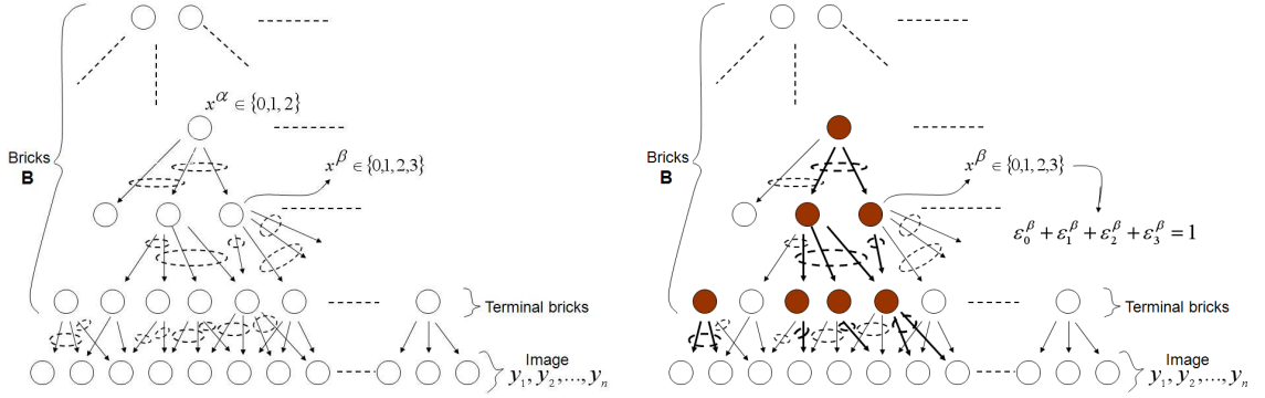
Figure 1.3: Architecture. Left. A hierarchy of “bricks,” each representing a disjunction of conjunctions. Bottom row is the image (pixel) data and the row above it is the set of terminal bricks. The state of a brick signals a chosen set of children. Right. An “interpretation,” which is an assignment of states such that the chosen children of any “on” brick are also on. There can be multiple roots and shared subtrees. Filled circles represent on bricks (non-zero states), and highlighted edges represent chosen children.
