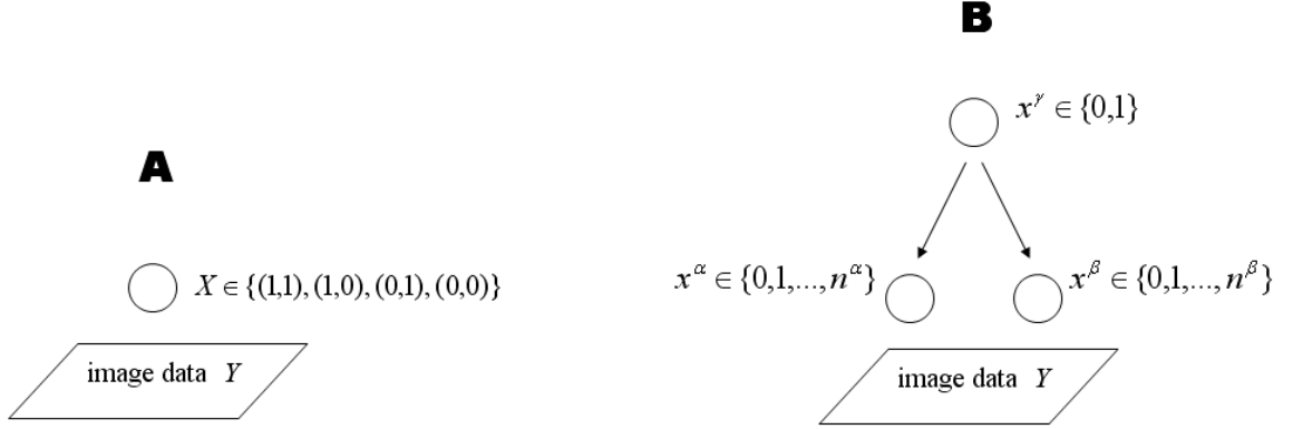
Figure 2.2: Graphical model. Panel “A” is a graphical representation for the non-hierarchical setting in Section 2.3. Panel “B” is a graphical representation for the hierarchical settings in Section 2.4.
