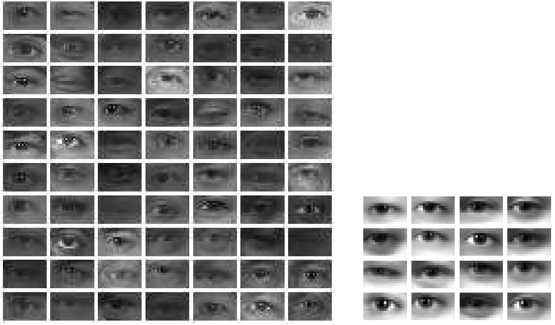
Figure 4.5: The left panel shows 70 training left eye images, each with size 15 \times 23 ). The right panel shows the 16 learned templates, each with size 12 \times 19 , under the model with mixtures over multiple templates and spatial shifts.
