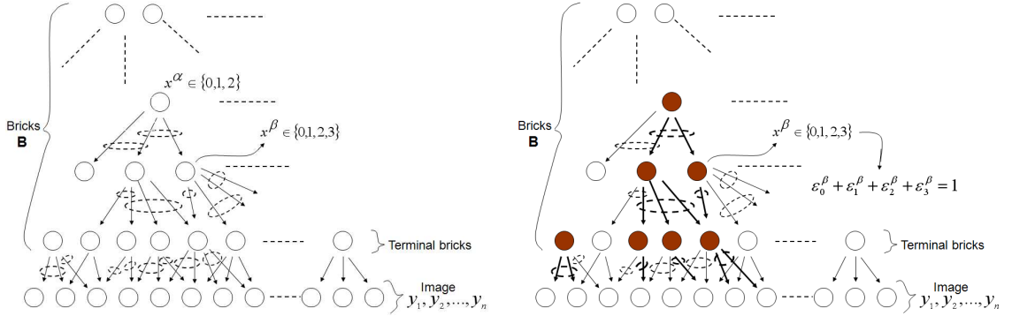
Figure 3.1: Architecture. Left. A hierarchy of “bricks,” each representing a disjunction of conjunctions. Bottom row is the image (pixel) data and the row above it is the set of terminal bricks. The state of a brick signals a chosen set of children. Right. An “interpretation,” which is an assignment of states such that the chosen children of any “on” brick are also on. There can be multiple roots and shared subtrees. Filled circles represent on bricks (non-zero states), and highlighted edges represent chosen children.
