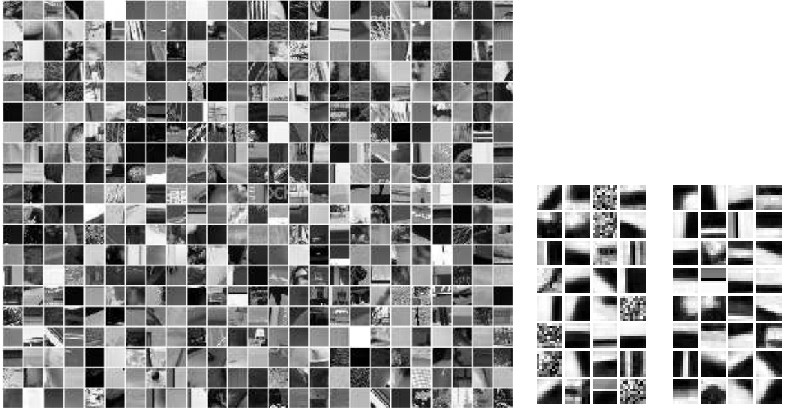
Figure 4.19: The left panel shows 500 randomly selected training image patches ( 15 \times 15 ). The middle panel shows the 32 learned templates from the improved background model, each with size 10 \times 10 . The right panel shows the 32 learned templates from the basic background model, each with size 10 \times 10 .
