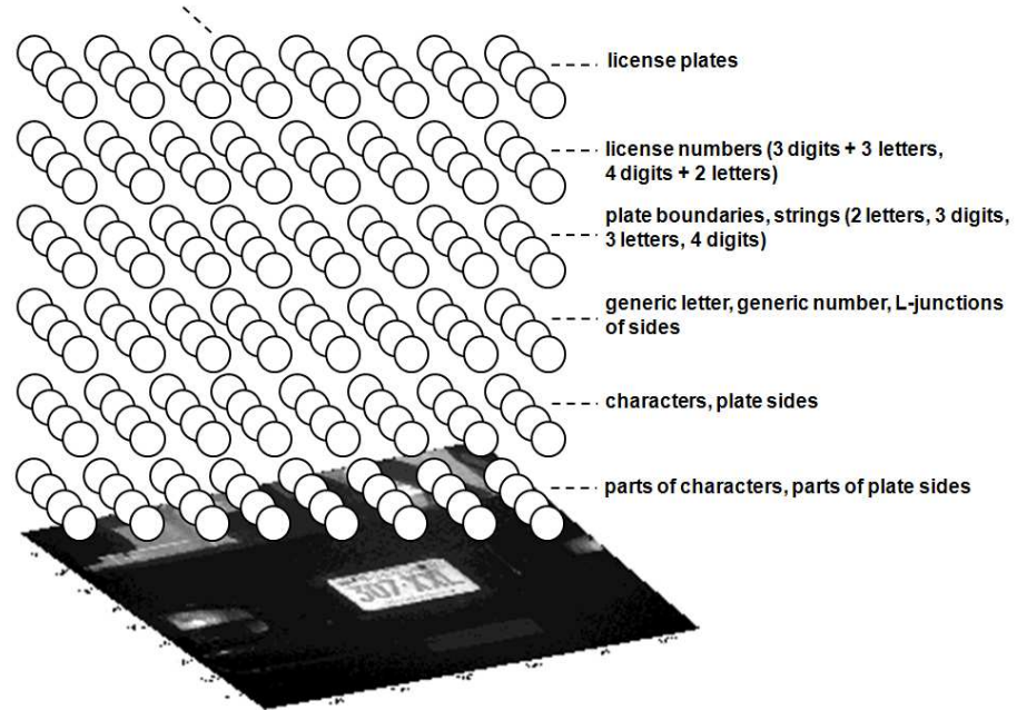
Figure 1.2: Semantic hierarchy for plate-reading application
