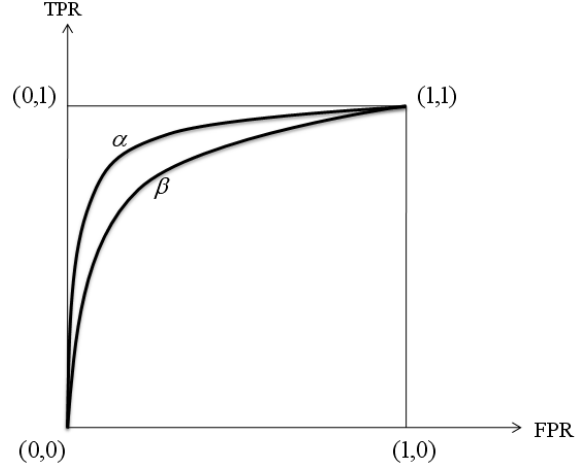
Figure 2.1: An example of two ROC curves. The ROC curve \alpha is always strictly higher on the Y axis than the ROC curve \beta . Hence the decision rule associated with \alpha is strictly better than the one associated with \beta .
