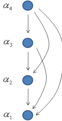
Figure 3.2: The special hierarchy structure in Step 1 and Step 2, when N=4 .
