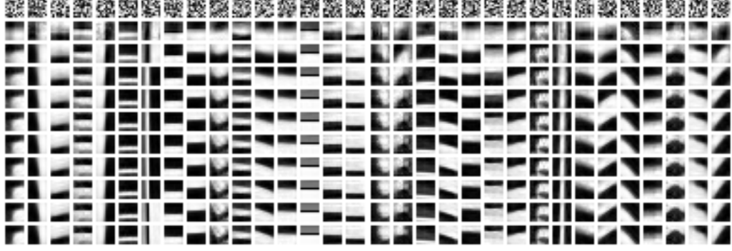
Figure 4.18: The evolution of the 32 templates during 20 runs of the EM algorithm, under the basic background model, where the first row shows the random initialization of the templates.
