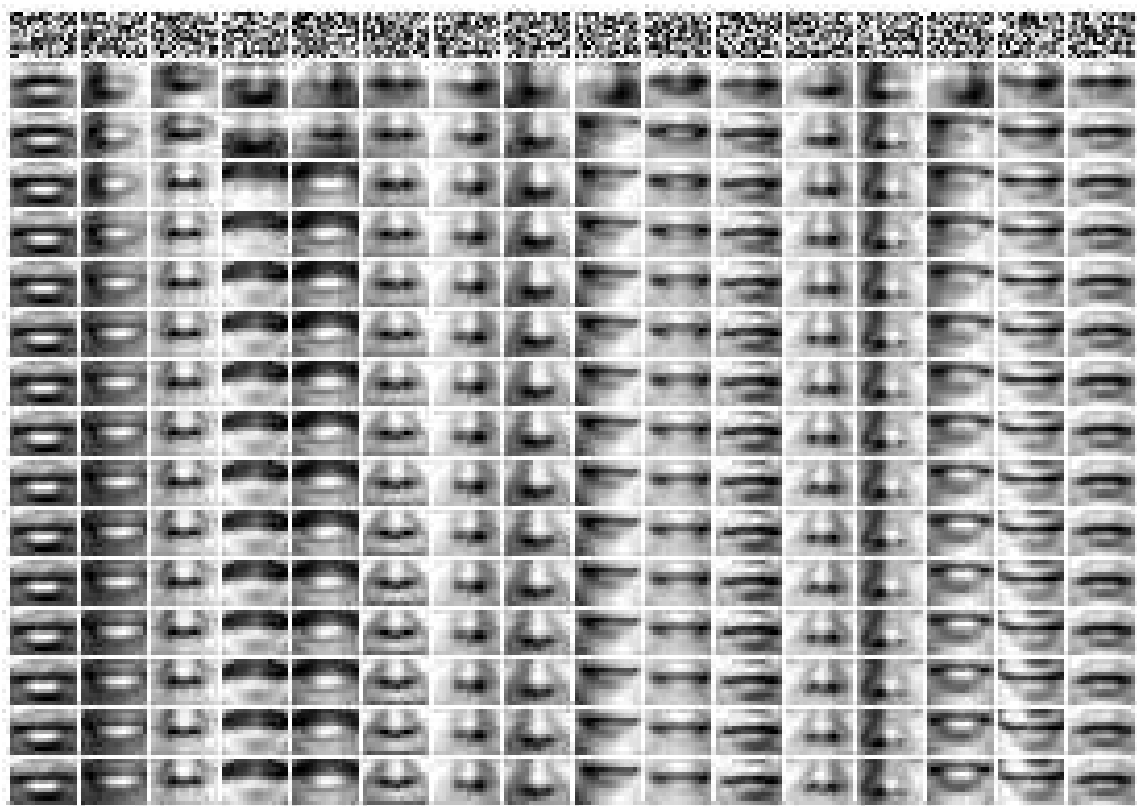
Figure 4.12: The evolution of the first 16 templates as the EM algorithm ran, starting from a random initialization.
