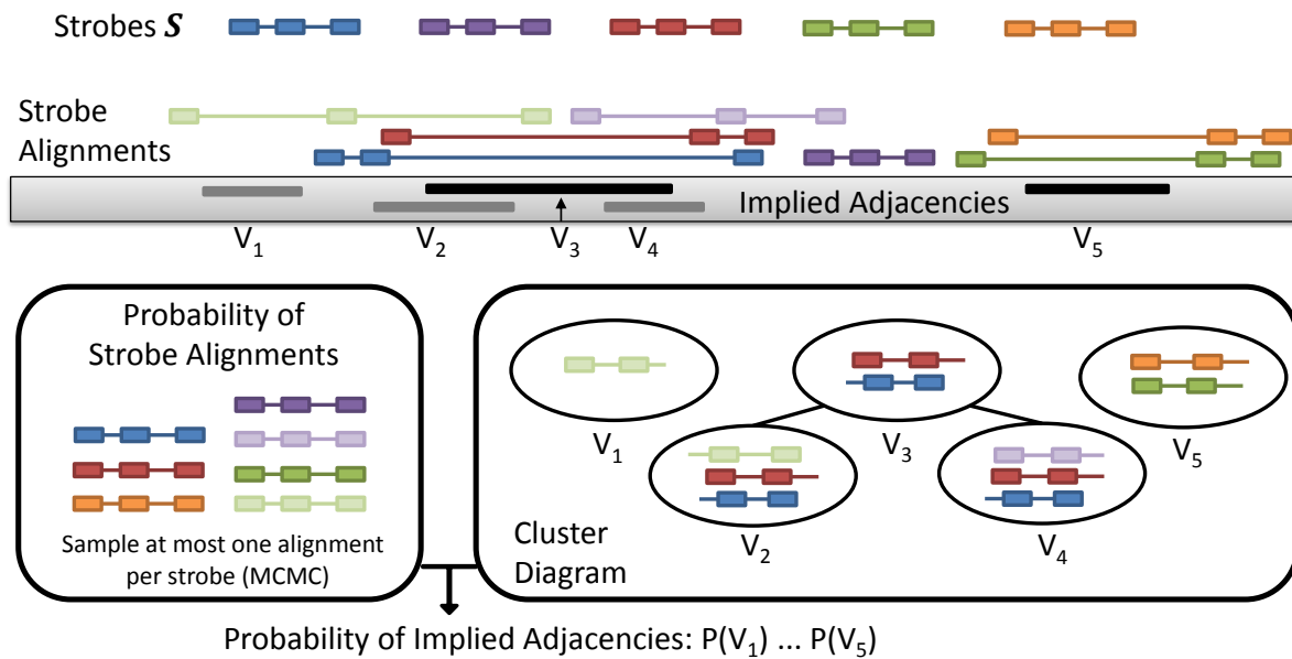
Figure 4.1: Overview of the probabilistic model for SV prediction from strobe sequencing data. In this example there are five strobos; three have a unique strobe alignment to the reference (blue, red, and orange), and two have two strobe alignments to the reference (green and purple). There are five adjacencies that are implied by different selections of strobe alignments; suppose that two of them ( V_3 and V_5 ) are correct. The implied adjacencies are represented as a cluster diagram G , where the nodes are the adjacencies and the edges denote interval overlaps. Using an MCMC method, we compute the probability of each strobe alignment in the space by sampling at most one alignment for each strobe with probability proportional to the posterior of the mappings. Finally, these probabilities are used to assign a probability of each implied adjacency (i.e. each node in G ).
