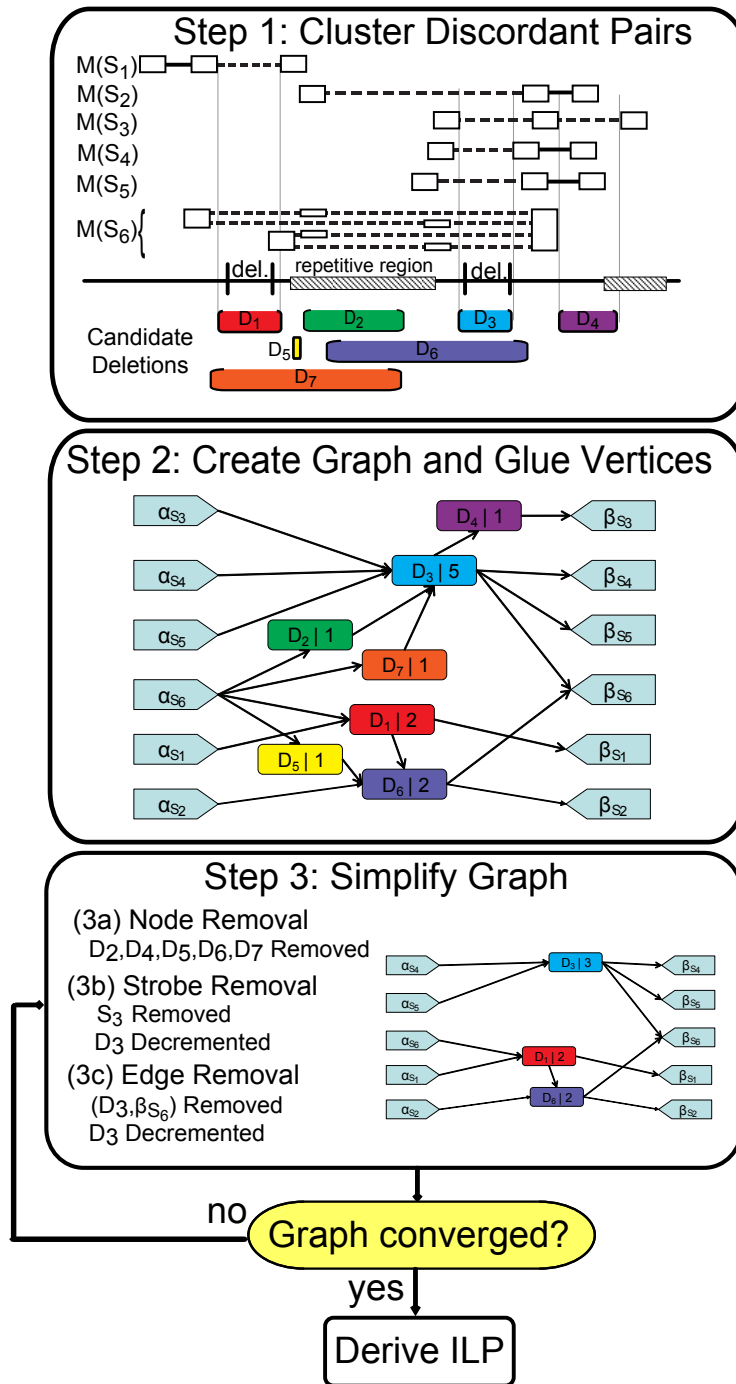
Figure 3.3: Construction of graph for 3-strobes S_1, \dots, S_6 . In step 1, the discordant pairs (dotted lines) representing a particular breakpoint type (deletions) are clustered, producing 7 candidate deletions. In step 2, a graph is created with a source vertex \alpha and a sink vertex \beta for each strobe and one vertex for each cluster. The number on each vertex indicates the number of strobes with a discordant pair consistent with the deletion. In step 3, the graph is simplified using heuristics described in § 3.3.4. Step 3 is repeated until the graph has converged, upon which it is used as input to the ILP.
