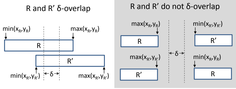
Figure 5.2: \delta -Overlapping vs. non- \delta -overlapping strobes in a strobe layout. Here, the subread orientations are ignored as the minimum or maximum value for each coordinate is selected. If subreads R and R' \delta -overlap, then both (\max(x_R, y_R) - \min(x_{R'}, y_{R'}) + 1) and (\max(x_{R'}, y_{R'}) - \min(x_R, y_R) + 1) are greater than or equal to \delta . If they do not \delta -overlap, then either (\max(x_R, y_R) - \min(x_{R'}, y_{R'}) + 1) or (\max(x_{R'}, y_{R'}) - \min(x_R, y_R) + 1) is less than \delta .
