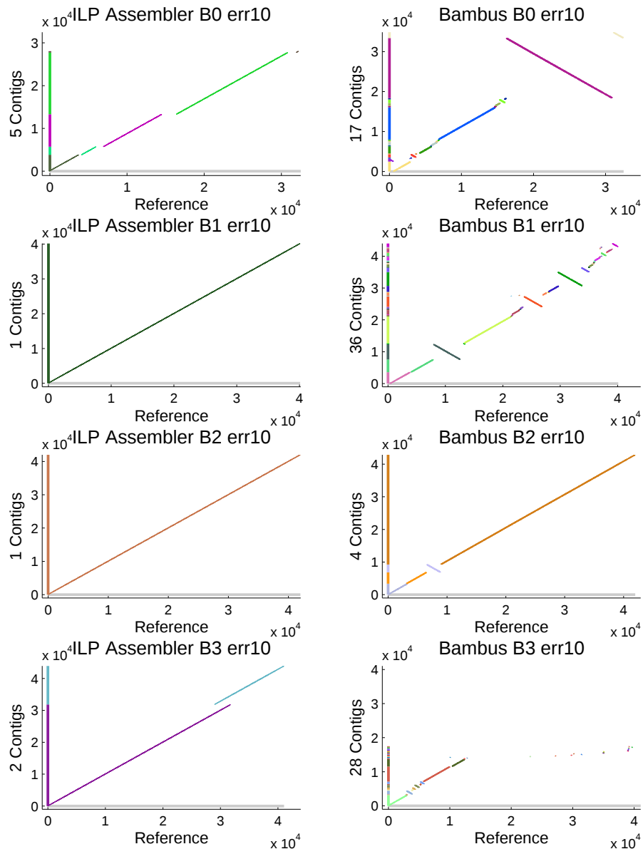
Figure 5.8: Comparison of Assemblies of BACs with 10% Error. Each “dot plot” aligns the contigs produced by the assembler to the reference, each colored a different color. Assemblies from the ILP assembler (Left) are more complete (less fragmented) than the assemblies from the Minimus/Bambus Assembler with Smith-Waterman alignments (Right).
