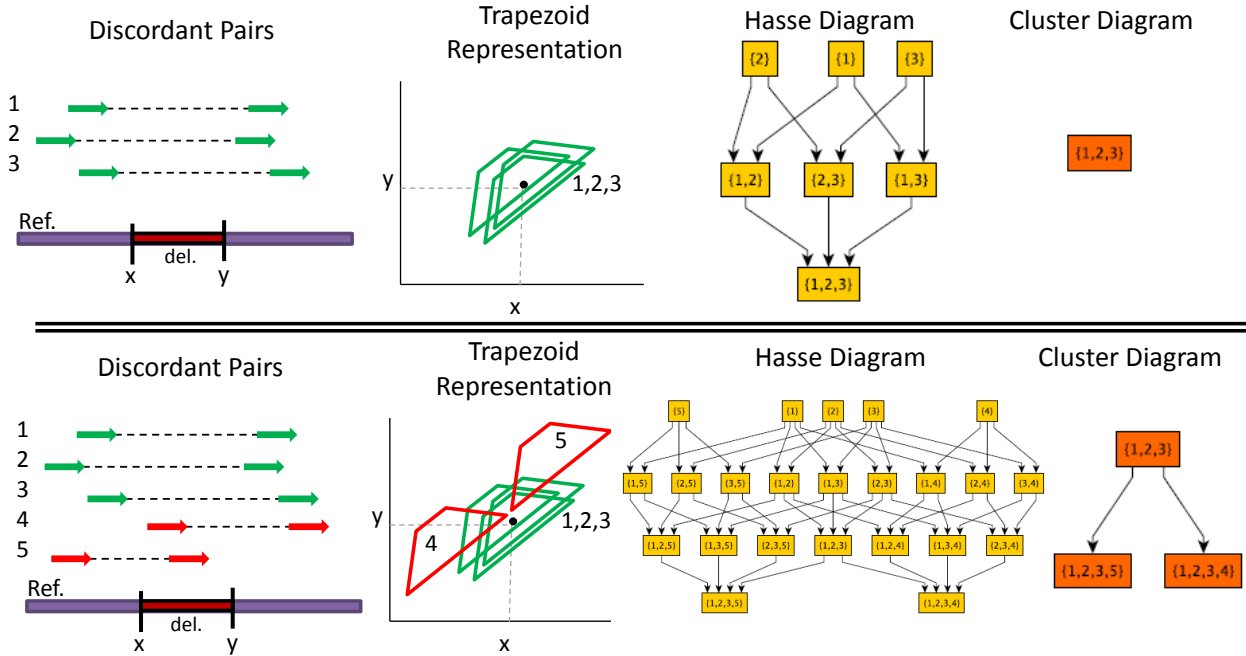
Figure 4.2: Cluster Diagram Construction. Cluster Diagrams for (Top) discordant pairs with a common area of intersection and (Bottom) discordant pairs with no common area of intersection. Each discordant pair can be represented as a trapezoid in \mathbb{R}^2 , and the set of all transitively-reduced intersections is a Hasse diagram (a partially ordered set on the pairs with the subset operator). After successively contracting nodes with a single outgoing edge and removing transitive edges, we get a cluster diagram. For sets of pairs with a common intersection, the cluster diagram is simply a single node.
