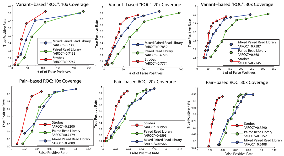
Figure 3.5: ROC curves for the Venter simulation. The top row is a variant-based “ROC” curve for 124 deletions \geq 120 basepairs, which computes the number of real deletions out of 124 that appear in the solution. The bottom row is a pair-based ROC curve for the same 124 deletions, which counts the number of discordant pairs that support the real deletions. The reported “AROC” is the area under the curves normalized by the maximum x-value in each plot. For 10x coverage, \Delta ranges from 2 to 10 in steps of 2. For 20x and 30x coverage \Delta ranges from 4 to 20 in steps of 2.
