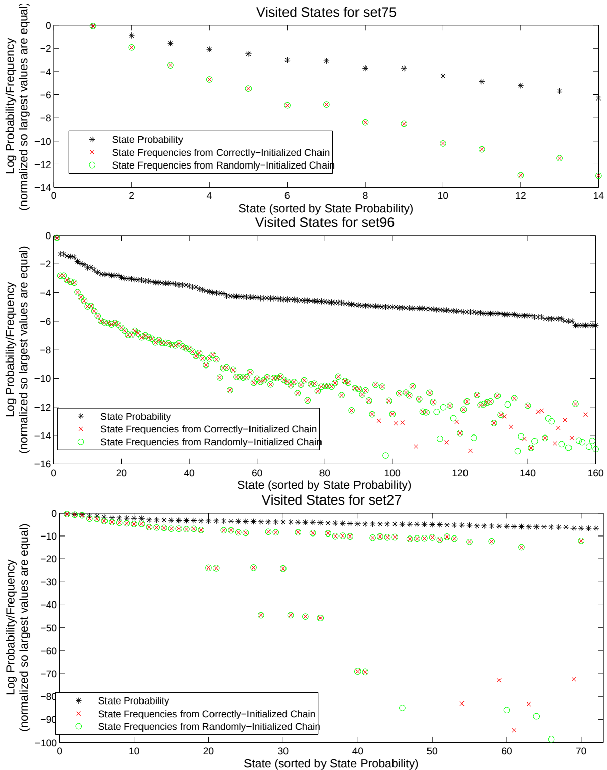
Figure 4.8: MCMC Convergence on Subproblems for 2X Strobes. MCMC convergence on a small subproblem (Top), an average-sized problem (Middle), and the largest subproblem (Bottom). The black asterisks denote the (unnormalized) probabilities of each state sampled in the 5 million iterations of the MCMC method. The red crosses and the green circles denote the relative sampling frequencies of each state for the correctly-initialized and randomly-initialized chains.
