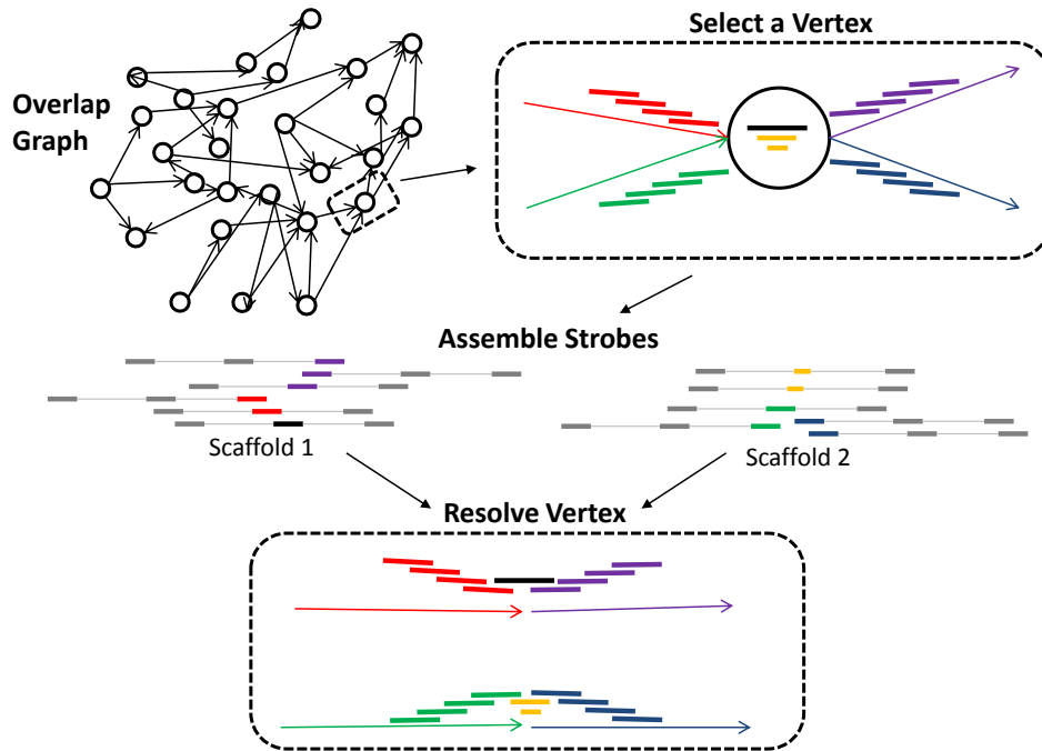
Figure 6.2: Resolving Vertices in the Overlap Graph. Assembling the strokes that are associated with subreads from a vertex could potentially resolve the ambiguities represented by the vertex.
