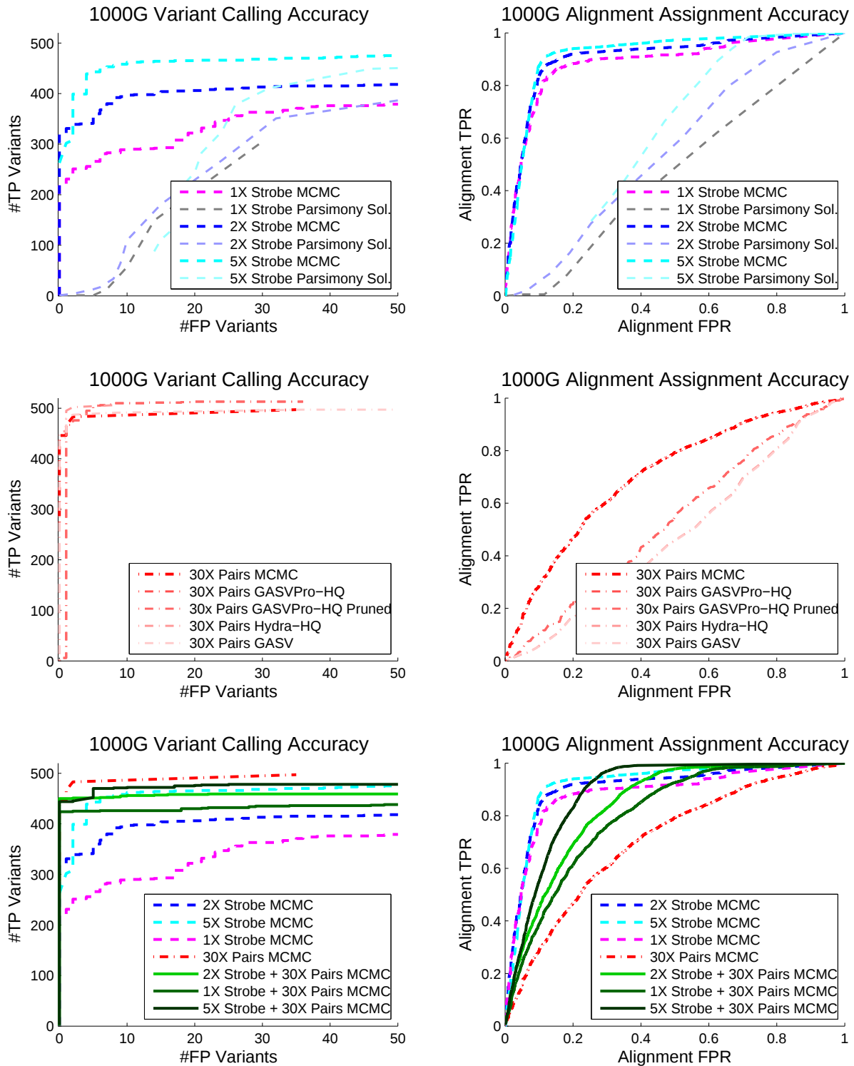
Figure 4.4: (Left) Variant calling accuracy and (Right) alignment assignment accuracy for datasets from the 1000 Genomes simulation. Dashed lines are strobe datasets, dot-dash lines are paired datasets, and solid lines are hybrid datasets. The plots are plotted as (top) MCMC vs. Parsimony Solution for 1X, 2X, and 5X strobos, (middle) the paired dataset run with a variety of methods, and (bottom) all the datasets run with the probabilistic method. Boldface lines are datasets run with our model: we compared the strobe datasets to a parsimony solution [124] and the paired datasets to Hydra [119], GASV [133], and GASVPro [134]. GASVPro-HQ is the original predictions output by GASVPro on unique alignments, and GASVPro-HQ Pruned removes overlapping variants from the predictions. Hydra-HQ is the Hydra method applied to unique alignments.
