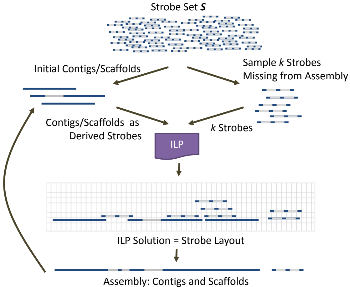
Figure 5.5: Overview of the Iterative ILP Assembler. A set of initial contigs are established from the set of strobes S . These contigs are formulated as derived strobes, combined with k strobes sampled from the remainder of the set, and run through the ILP. The resulting strobe layout defines a set of new contigs and scaffolds that are then passed as derived strobes in the next iteration. The method terminates when no ILP solution is found or all the strobes are in the assembly.
