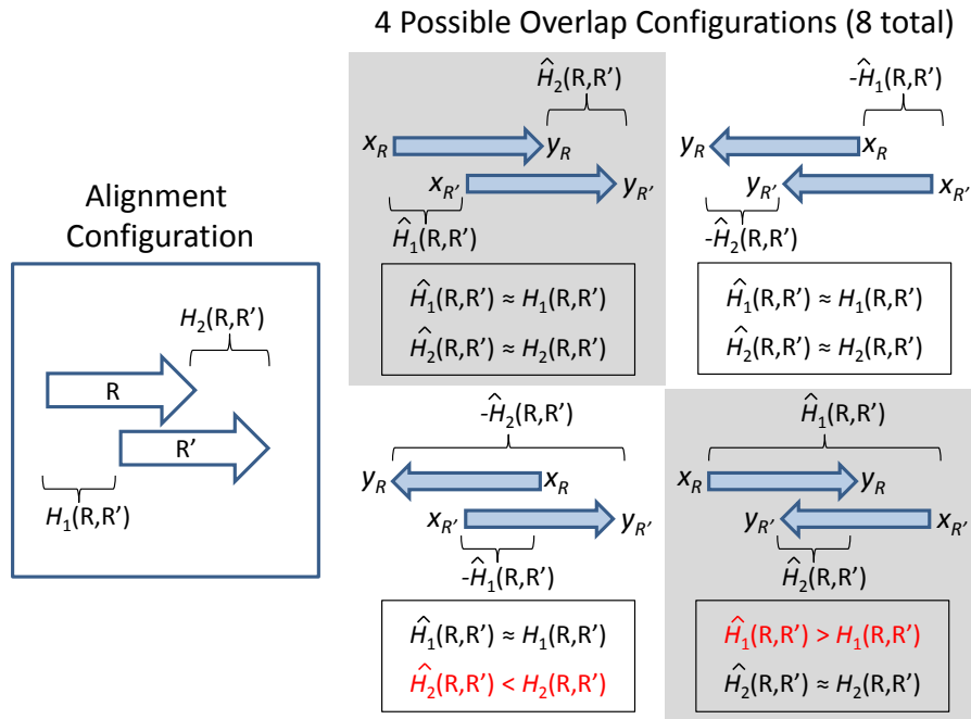
Figure 5.3: Four of eight possible overlap configurations. The inequalities in red are instances where \hat{\mathcal{H}}_1(R, R') is not near \mathcal{H}_1(R, R') or \hat{\mathcal{H}}_2(R, R') is not near \mathcal{H}_2(R, R') ; thus, R and R' cannot \delta -overlap according to these configurations. The other four overlap configurations include subread R being to the right of R' ; in those configurations, none of \hat{\mathcal{H}}_1(R, R') or \hat{\mathcal{H}}_2(R, R') are near \mathcal{H}_1(R, R') or \mathcal{H}_2(R, R') , respectively.
