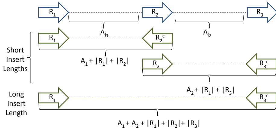
Figure 5.7: Converting Strobos to Pairs to Preserve Pairing Information. Two paired reads with “short” insert sizes and one paired read with a “long” insert size is created.
