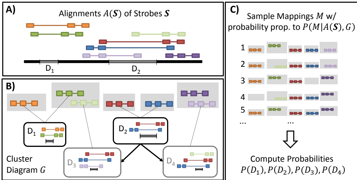
Figure 4.3: Overview of the Probabilistic Algorithm for SV Prediction. In this example, there are five strokes in the set S : orange, green, red, blue, and purple. A) There are two strobe alignments for the green and the purple strokes, and the rest of the strokes have a single strobe alignment. The correct strobe alignments (the orange, dark green, red, blue, and dark purple alignments) support two novel adjacencies ( D_1 and D_2 ). However, the light green and light purple alignments introduce two incorrect novel adjacency predictions. B) The space of all possible novel adjacencies is represented as a cluster diagram G , where the nodes are novel adjacencies and the directed edges represent overlapping novel adjacencies. The edges from the strokes to the nodes are not part of G , but are shown here for clarification. C) A solution to the t - Multiread Mapping Problem is a selection of at most one alignment for each strobe in S , called a mapping , which supports some subset of the deletions. We sample mappings from the solution space proportional to the mapping's posterior probability; from these sampled mappings, we finally compute the probabilities of the four deletions.
