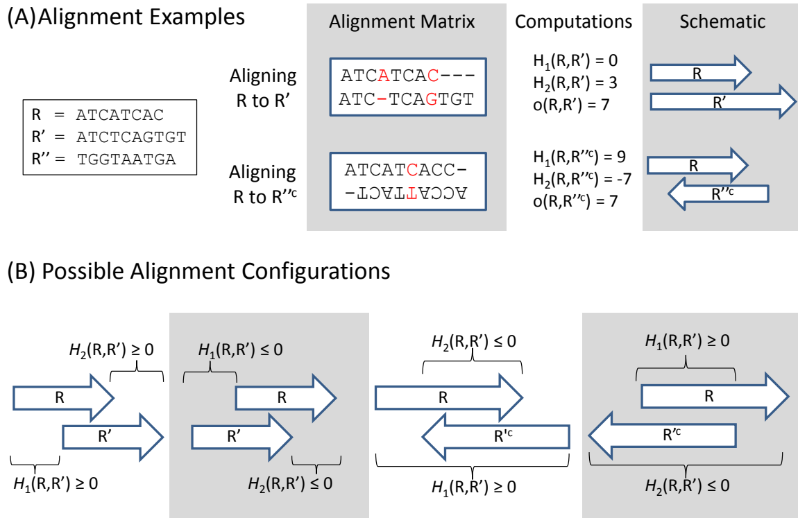
Figure 5.1: Alignment Examples and possible alignment configurations. (A) Two examples of end-space free alignments. The alignment of R and R' contains an indel and a substitution (in red in the alignment matrix). The alignment of R and R''^c contains a substitution. (B) \mathcal{H}_1(R, R') and \mathcal{H}_2(R, R') for possible alignment configurations of R and R' . Note that, if R and R' are in the same orientation, then the sign of \mathcal{H}_1(R, R') is the same as the sign of \mathcal{H}_2(R, R') (or they are both 0). If R' is in the reverse orientation, then one of \mathcal{H}_1(R, R') and \mathcal{H}_2(R, R') is non-negative and the other is negative.
