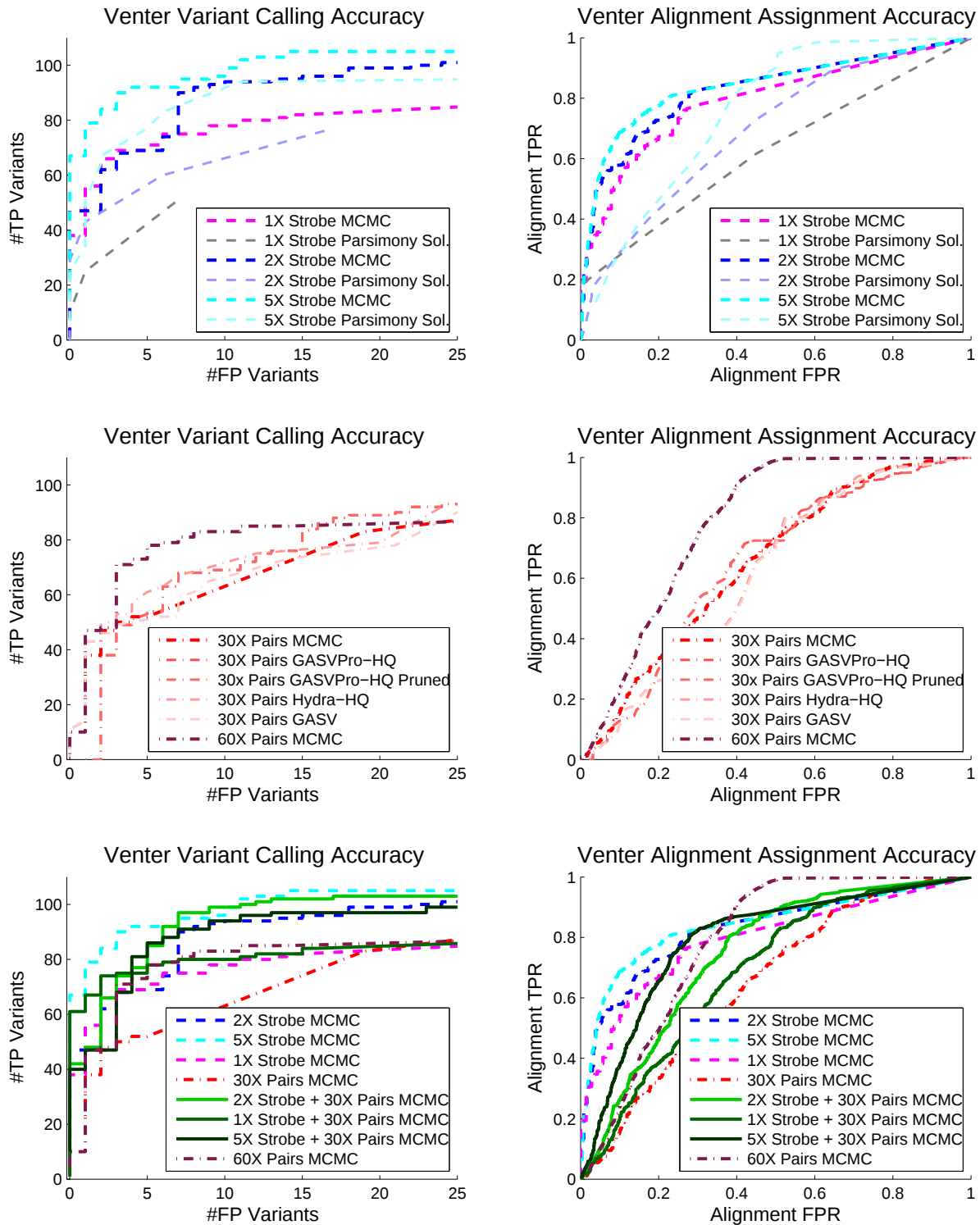
Figure 4.7: (Left) Variant calling accuracy and (Right) alignment assignment accuracy for datasets from the Venter simulation. Dashed lines are strobe datasets, dot-dash lines are paired datasets, and solid lines are hybrid datasets. The plots are plotted as (top) MCMC vs. Parsimony Solution for 1X, 2X, and 5X strobos, (middle) the paired dataset run with a variety of methods, and (bottom) all the datasets run with the probabilistic method. Boldface lines are datasets run with our model: we compared the strobe datasets to a parsimony solution [124] and the paired datasets to Hydra [119], GASV [133], and GASVPro [134]. GASVPro-HQ is the original predictions output by GASVPro on unique alignments, and GASVPro-HQ Pruned removes overlapping variants from the predictions. Hydra-HQ is the Hydra method applied to unique alignments.
