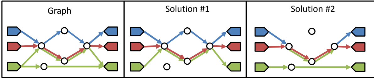
Figure 3.4: The graph G that is constructed is not an example of a fixed-charge network flow algorithm. Here we show an example graph G and potential solutions to the fixed-charge network-flow problem. The graph edges are colored by the three strobes (blue, red and green) that are allowed to travel that edge. Solution #1 shows a feasible solution to the fixed-charged network-flow problem uses four internal vertices. Solution #2 also contains with four internal vertices. However, solution #2 does not result in a path from source to sink for each individual strobe. Thus, solution #2 is not a feasible solution to the t -Strobe Minimum Breakpoints Problem.
