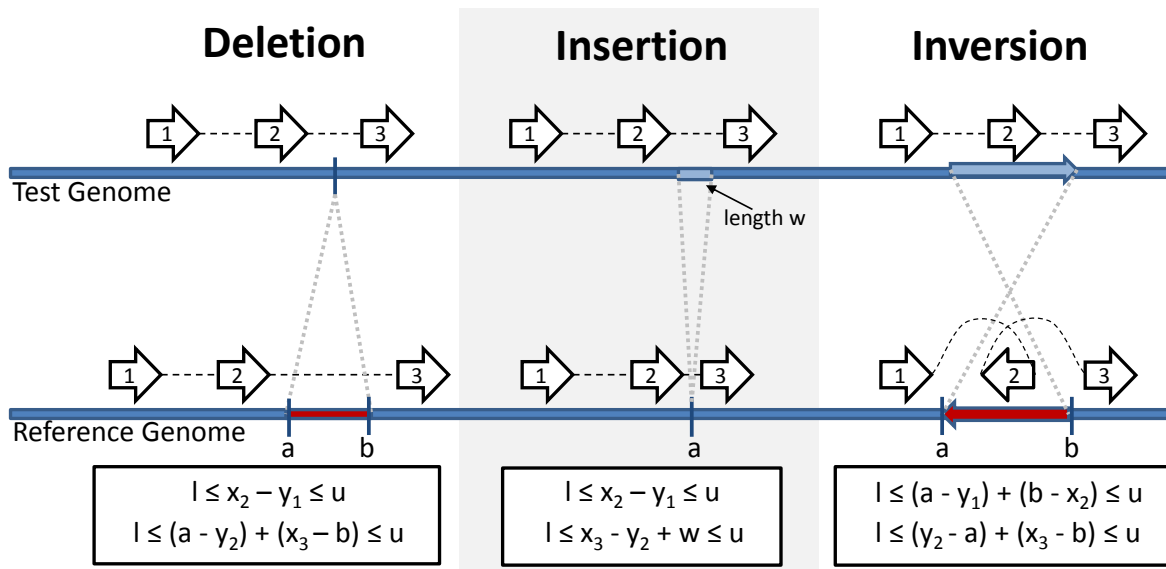
Figure 3.2: Discordant pairs that imply SVs and the constraints they pose on the type of variant. For simplicity, we label the subreads 1, 2 and 3, and the corresponding intervals as [x_1, y_1] , [x_2, y_2] , and [x_3, y_3] . SV coordinates are labeled as a and b in the reference genome. Each strobe corresponds to two inequalities due to two sets of adjacent subreads (1, 2) and (1, 3). In the deletion and insertion example, the set of adjacent subreads (1, 2) results in a concordant pair. All other inequalities represent discordant pairs. Note that insertions are a special case that includes the length of the inserted block rather than two cut points. The inequalities for an example translocation are not shown.
