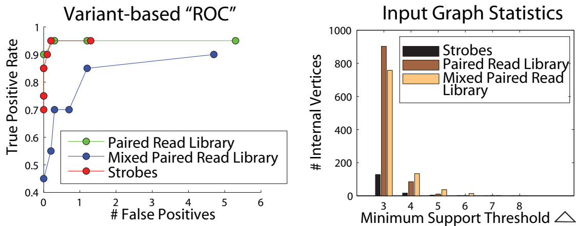
Figure 3.8: Statistics for ten 10x coverage simulations of a highly repetitive region. (Left) ROC curve of average number of false positives and average true positive rate, varying \Delta from 3 to 8. (Right) Distribution of the number of internal vertices in the generated graph.
