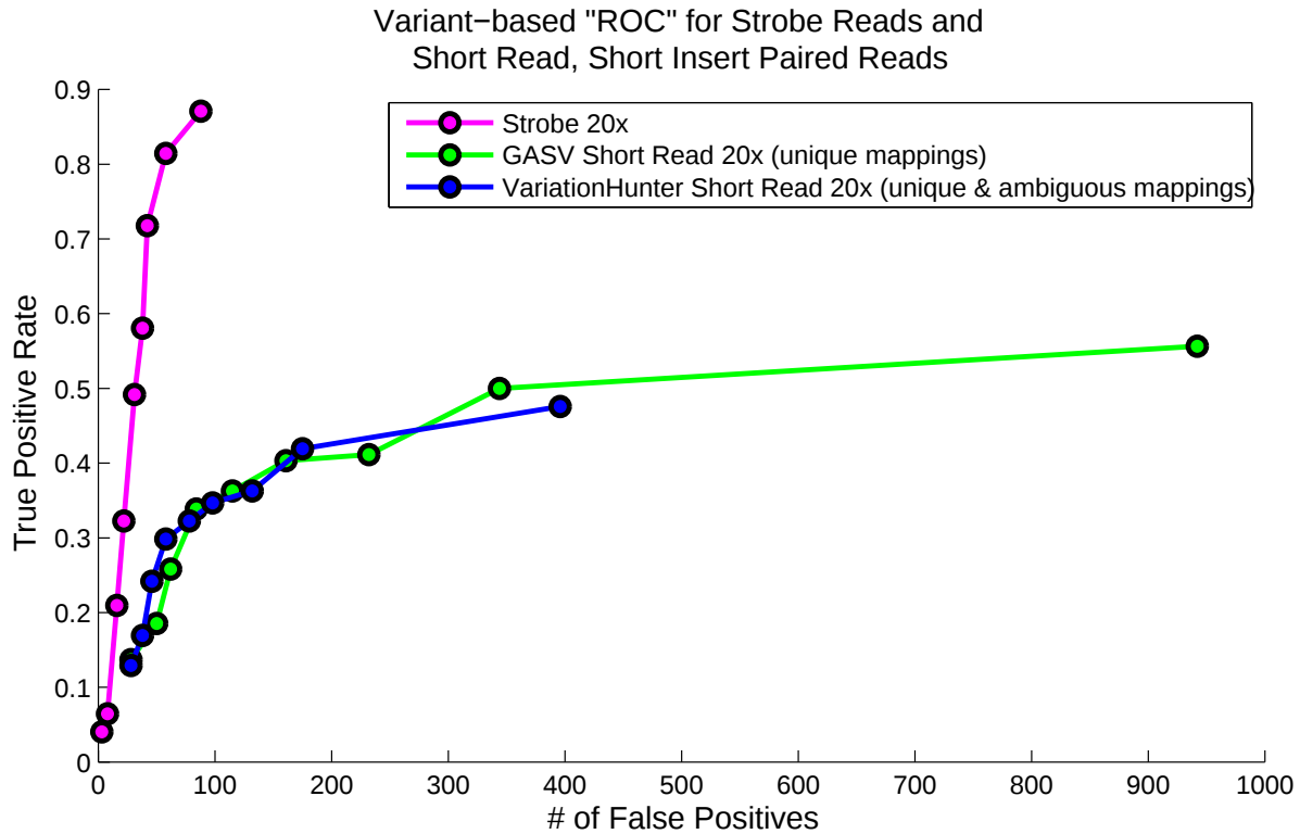
Figure 3.7: Strobe reads vs. paired-end reads on the Venter simulation. \Delta ranges from 4 to 20 in steps of 2 for all curves.
