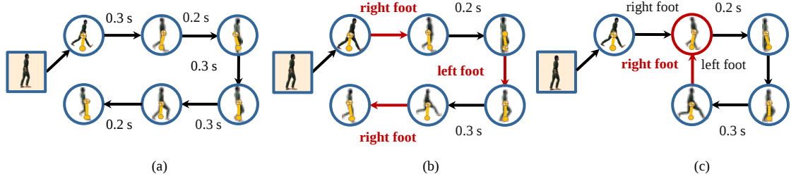
Figure 5.9: Refinement of Controller Structure. Illustration of the refinement of the controller structure for fast walk. The initial chain structure \mathcal{S}_M in (a) is first transformed in order to replace transitions based on time with those on contact, if an actual contact event happens close to the time of the transition. The obtained controller with the structure \mathbb{T}_\perp(\mathcal{S}_M) in (b) is more robust to external disturbances because the controller can react to explicitly to change of foot contact. This controller is further transformed in order to add a loop and remove duplicate states. The cyclic controller with the structure \mathbb{T}_\infty(\mathbb{T}_\perp(\mathcal{S}_M)) in (c) is now able to produce longer cyclic motions. See Figure 5.10 for the illustration of reconstruction results for the fast walk sequence with the cyclic controller obtained by the refinement.
