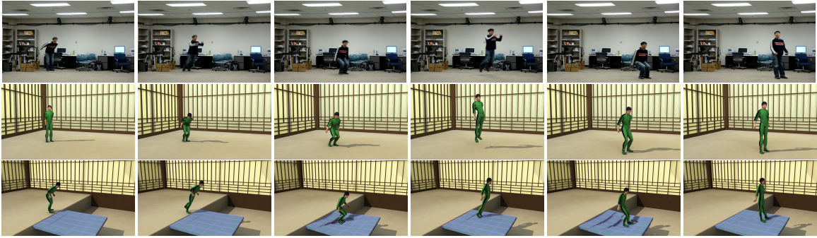
Figure 5.14: Video Result: Jump from VideoMocap. Input jump sequence from VideoMocap (top), reconstructed motion simulated by the controller estimated from the video (middle), new motion simulated in a modified environment (bottom).
