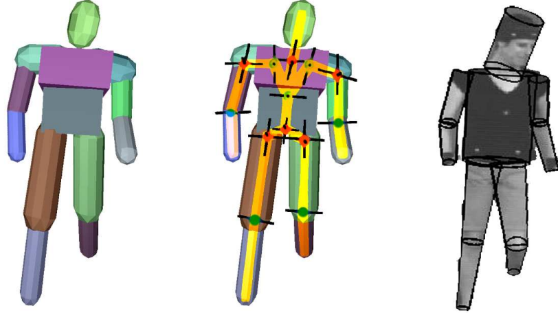
Figure 4.4: Body and Shape Model. 31 degree-of-freedom (DOF) character model with simulation shapes of the parts (left), the joints and skeletal structure (middle) and the image shapes in an image projection (right). Most joints have 3 DOFs, except for the knee and elbow joints (1 DOF), spine joint and the clavicle joints (2 DOFs) and the root joint (6 DOFs).
