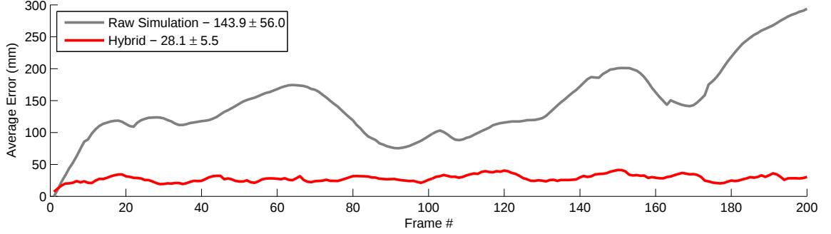
Figure 4.11: Raw Simulation Results (Tracking Errors, Multi-view L1 Walking). Pose reconstruction errors for results on the multi-view L1 walking sequence obtained with our physics-based motion estimation methods and an extended body model with extra parts to represent feet. See text in Section 4.2.4 for additional information on the methods.
