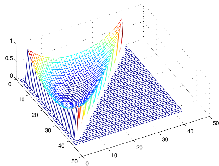
Figure 4.3: The graph of V^h for h = 1/40 of Example 4.5.1
