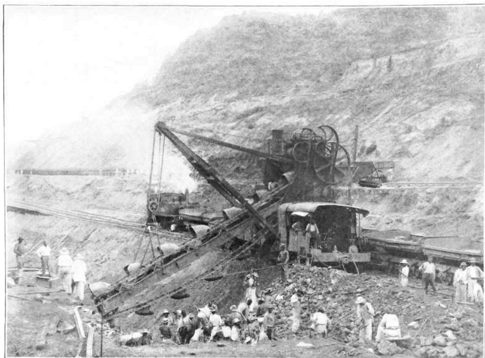
Showing the French system of excavation in the Culebra Cut.
