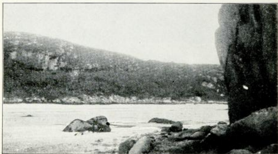
The channel between Earraid and Mull at low tide. The black band on the rocks shows mean high-water line, about six feet high.
