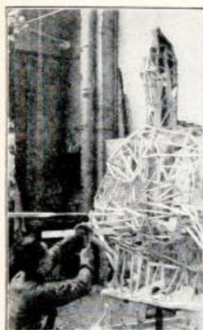
Left.—Armature of laths being made for enlargement of statue. Centre.—Armature partly filled in with plaster of paris, and showing the nails whose heads give the exact outline of the final statue. Right.—The plaster enlargement complete, showing also the original from which it was made.
