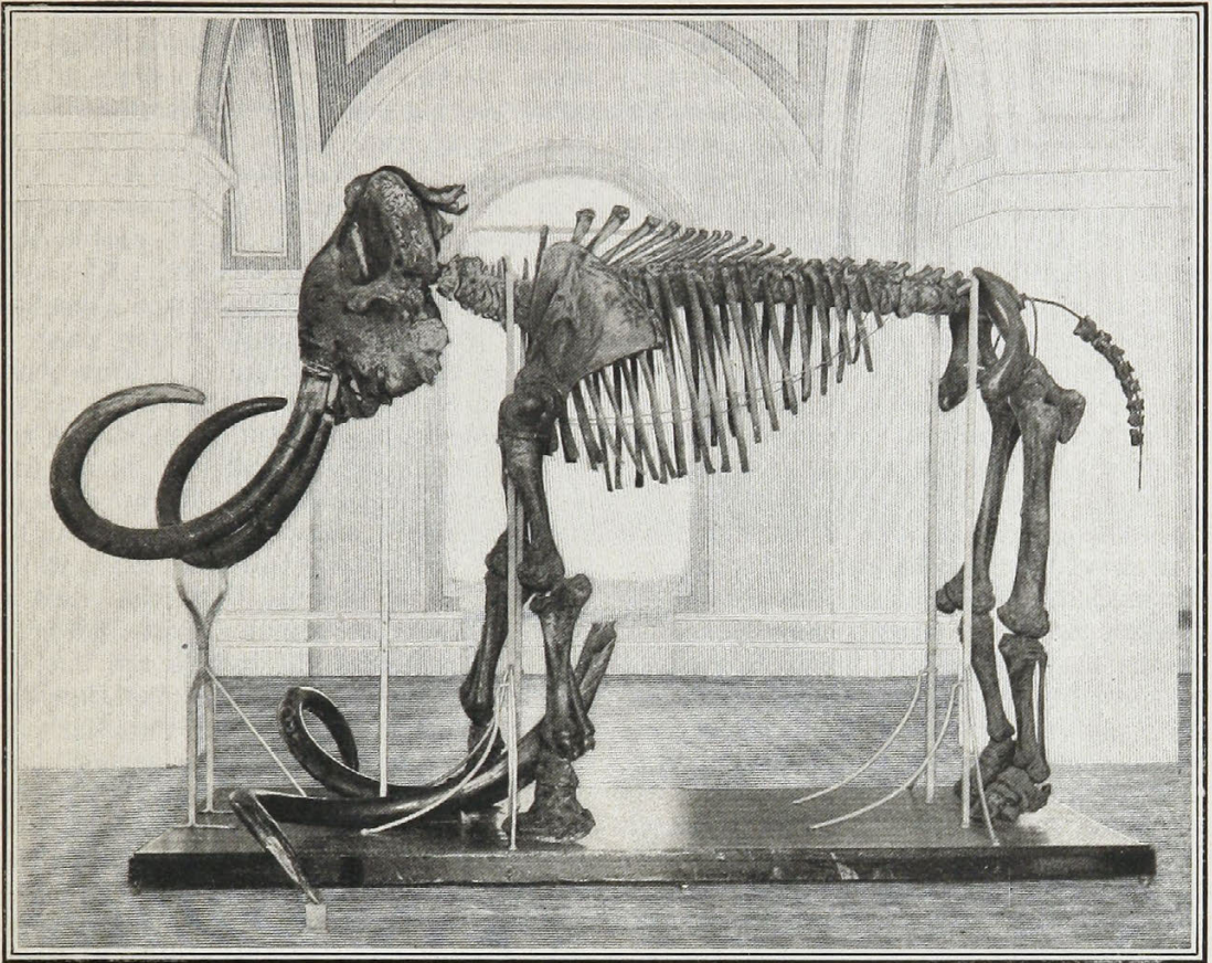
THE MAMMOTH IN THE ROYAL MUSEUM OF NATURAL HISTORY AT ST. PETERSBURG.
