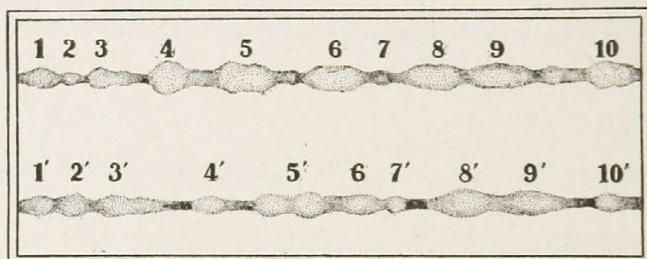
ENLARGEMENT OF PARTS OF THE ABOVE, SHOWING HOW THE ECHOES 1', 2', 3', ETC., TRAVELING OVER THE SURFACE, RESEMBLE IN SHAPE THE VIBRATIONS 1, 2, 3, ETC., WHICH TRAVELED THROUGH THE EARTH.
