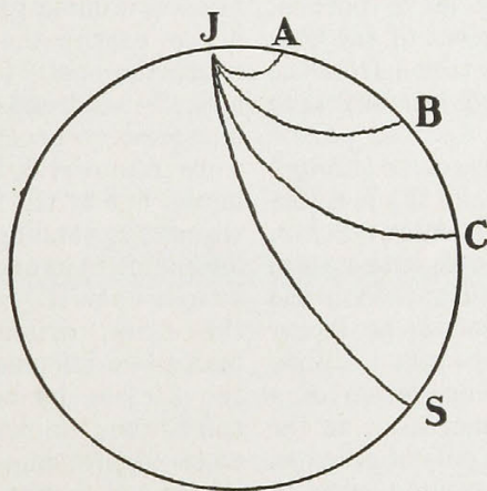
DIAGRAM SHOWING THE COURSES OF EARTHQUAKE TREMORS.
