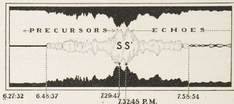
SEISMOGRAM OF THE EARTHQUAKE OF JUNE 29, 1898, IN THE SOUTH INDIAN OCEAN, AS RECORDED AT THE ISLE OF WIGHT.
