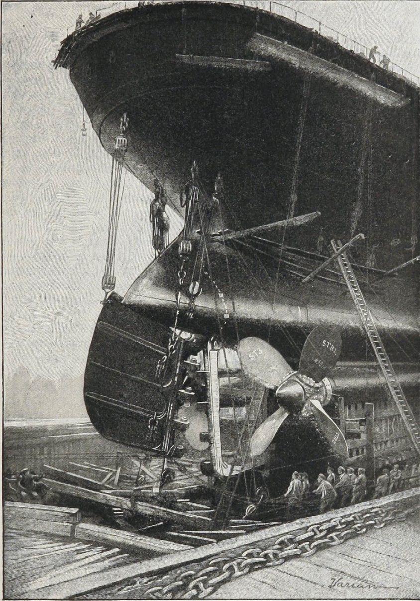
SHIPPING THE RUDDER.
