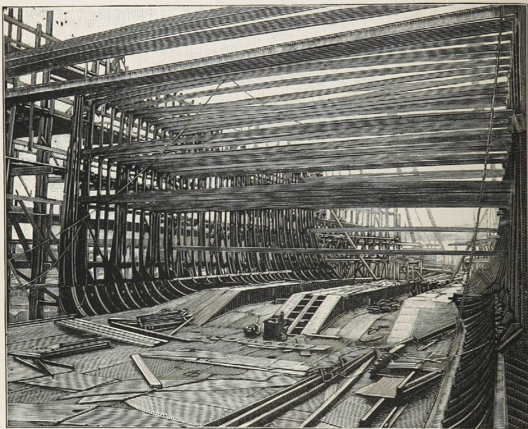
THE SKELETON OF THE "DEUTSCHLAND."
