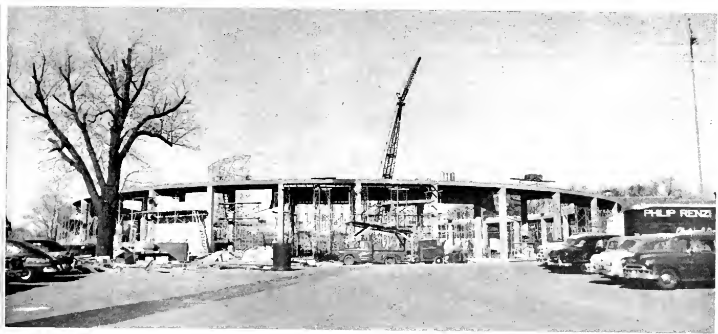
PROGRESS (below) on the Auditorium-Rink takes on meaning when compared with architect's drawing (above).
