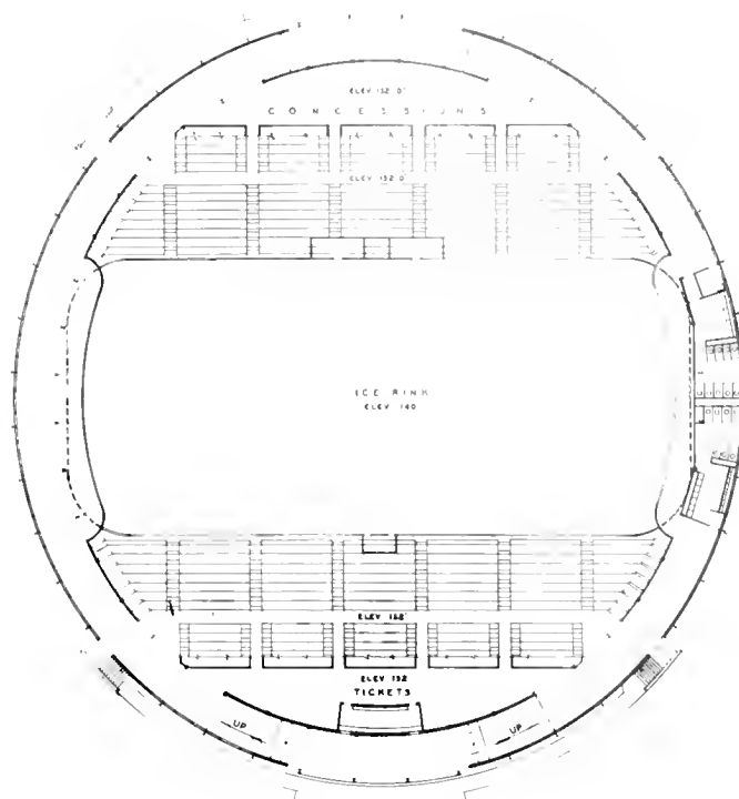
CHART shows how the ice surface and permanent seats for 2100 persons are accommodated in the oval of the Meehan Auditorium.
