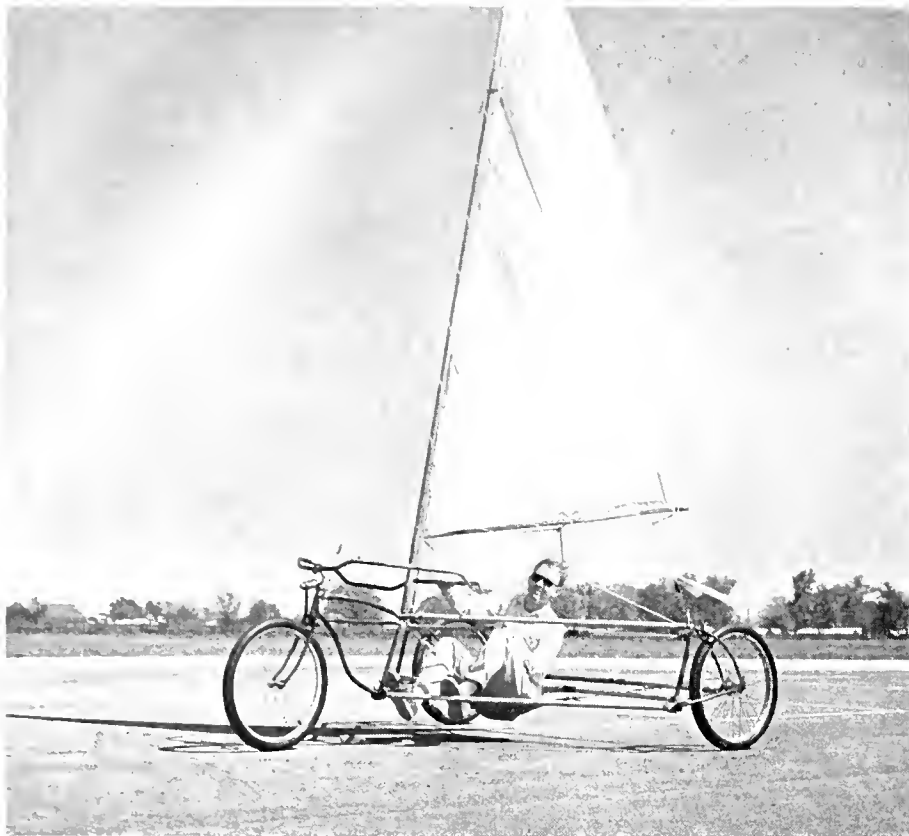
A DRY-LAND SAILOR, Robert A. Brown '60 of Lafayette, Ind., attracted considerable attention during the summer, with films on TV and this photo by Jesse McGreevy in the Indianapolis News. The latter called it "a weird-looking craft," but it proved landworthy. Brown, a mechanical engineer at Duncan Electric Manufacturing Co., built his sailmobile, using an old television antenna for the mast, bed-sheets for sail, and bicycle parts for the rest.
