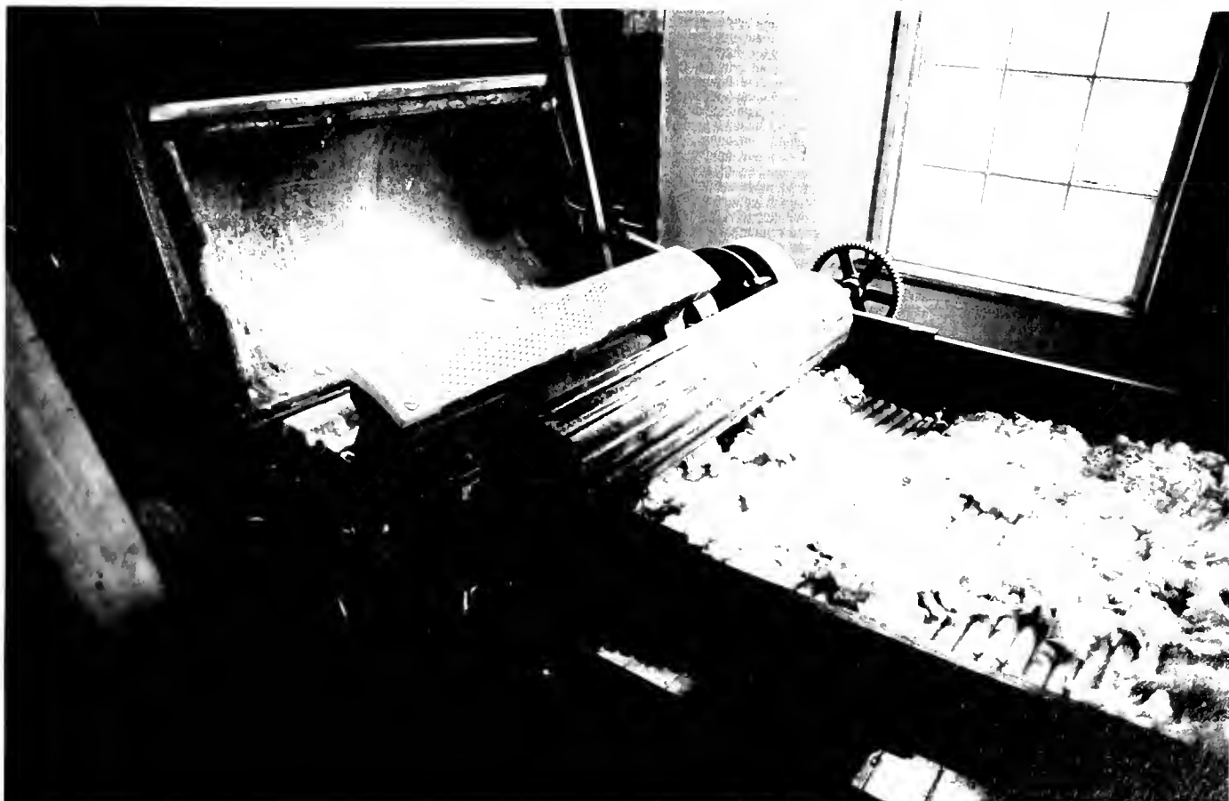
A breaker and picker on display in Slater Mill. This machine would break the cotton apart, and cull the seeds from the raw fiber.
