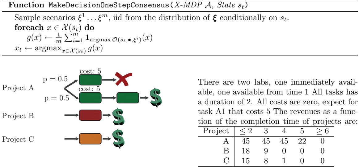
Figure 5.1: An instance of the S-RCPS on which 1s-AA is sub-optimal
