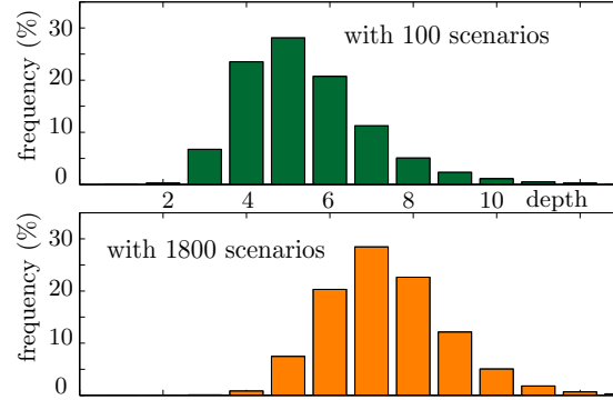
Figure 7.4: Distribution of the Depth of Explored Nodes by Amsaa for the Initial Decision.
