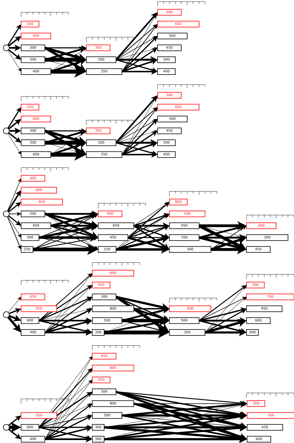
Figure 2.2: Stochastic model for instance Reg of the S-RCPPSP.
