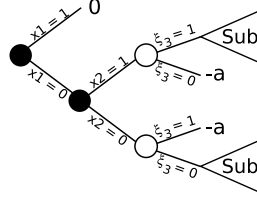
Figure 5.6: GAG higher than max of the EVPI s
