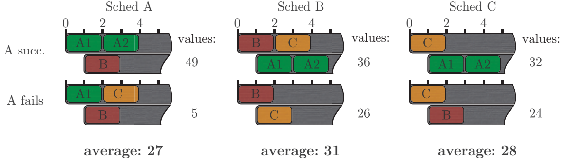
Figure 5.2: Offline optimal schedules and their values
