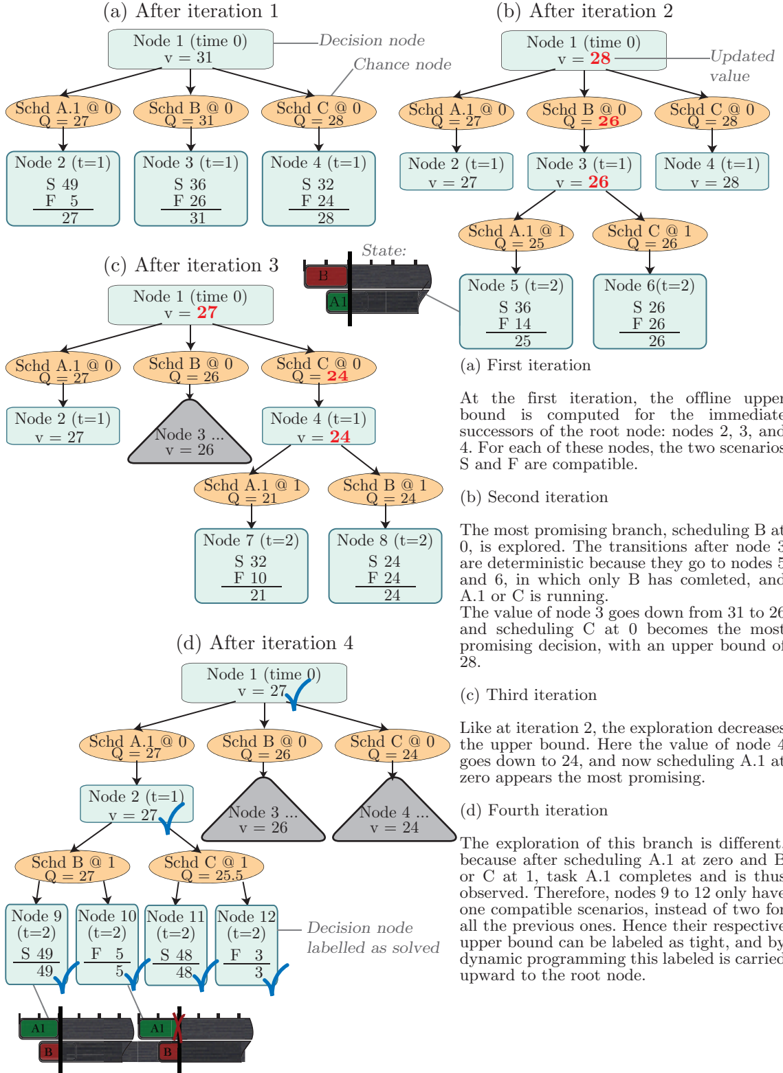
Figure 6.1: A run of Msaa
