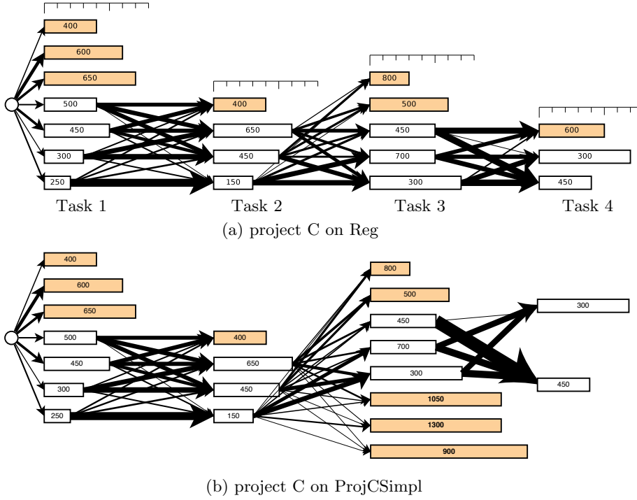
Figure 7.6: The project C in Reg and in a simplified instance
