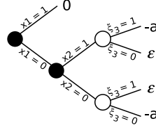
Figure 5.5: low EVPI but high Global Anticipatory Gap
