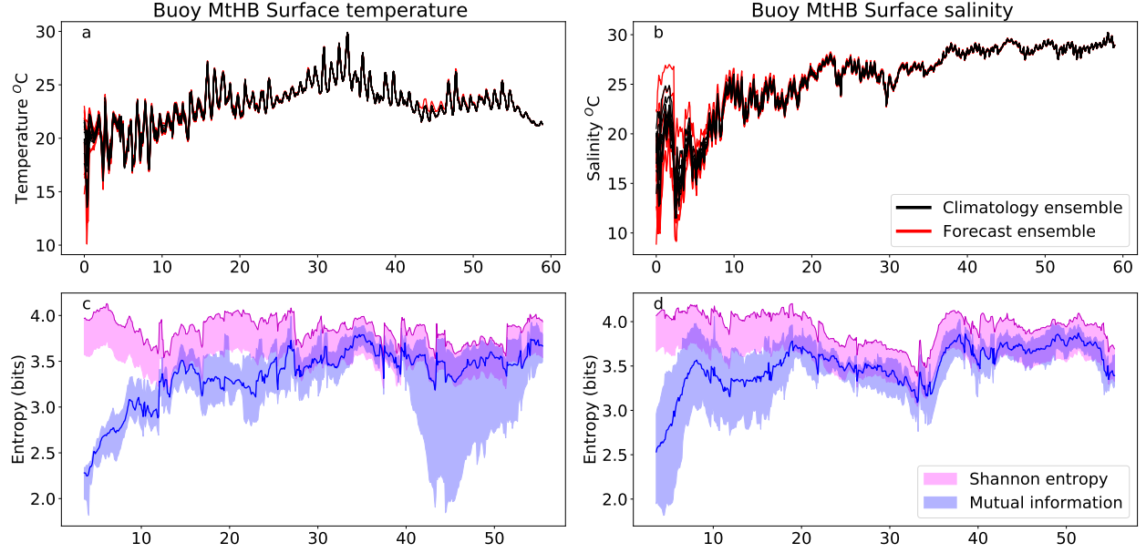
Figure 2.8: Surface temperature (a) and salinity (b) predictability metrics during July-August at one grid point closest to Mount Hope Bay (MtHB) buoy as shown in Figure 2.2. Information theory metrics for temperature and salinity are shown in c and d respectively. Surface temperature at this location is predictable for 27.4 [13.7 - 27.4] days and surface salinity is predictable for 18.5 [8.3 - 19.5] days. Figure S13 in the supporting information shows bottom temperature and salinity predictability.
