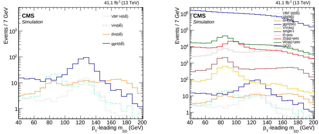
Figure 4.13: Corrected soft drop mass distribution for the p_T -leading jet. Left, simulated signal events normalized to their cross sections (Table 4.4). Right, background and signal events normalized to their cross sections.
