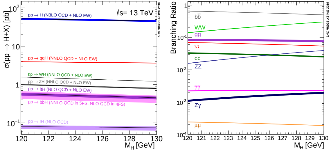
Figure 2.4: Minimal SM Higgs production and decay at the LHC [14]. Left: Production cross sections at \sqrt{s} = 13 TeV, for m_H = 120 –130 GeV. Right: Decay Branching Fractions for m_H = 120 –130 GeV.
