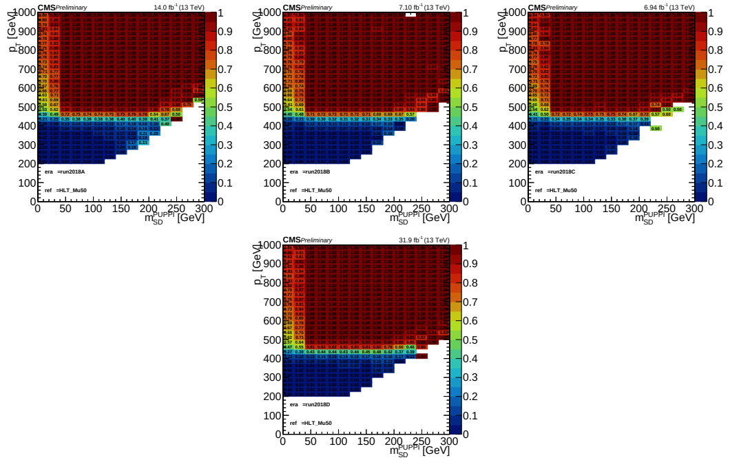
Figure 4.8: Measured trigger efficiency of the “OR” as function of jet p_T and jet m_{SD} is shown separately for each Run period in 2018.
