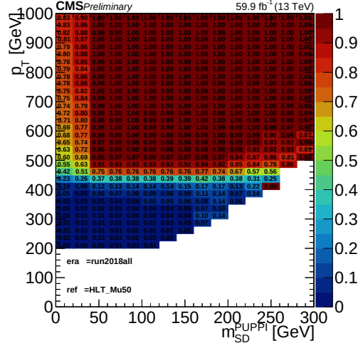
Figure 4.9: Measured trigger efficiency of the “OR” as function jet p_T and m_{SD} jet for Run 2018A-D.
