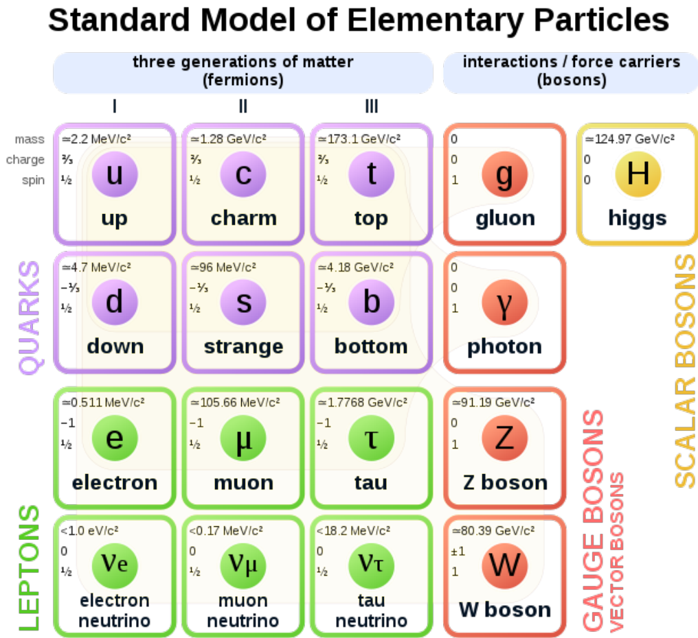
Figure 2.1: Particle content of the standard model.
