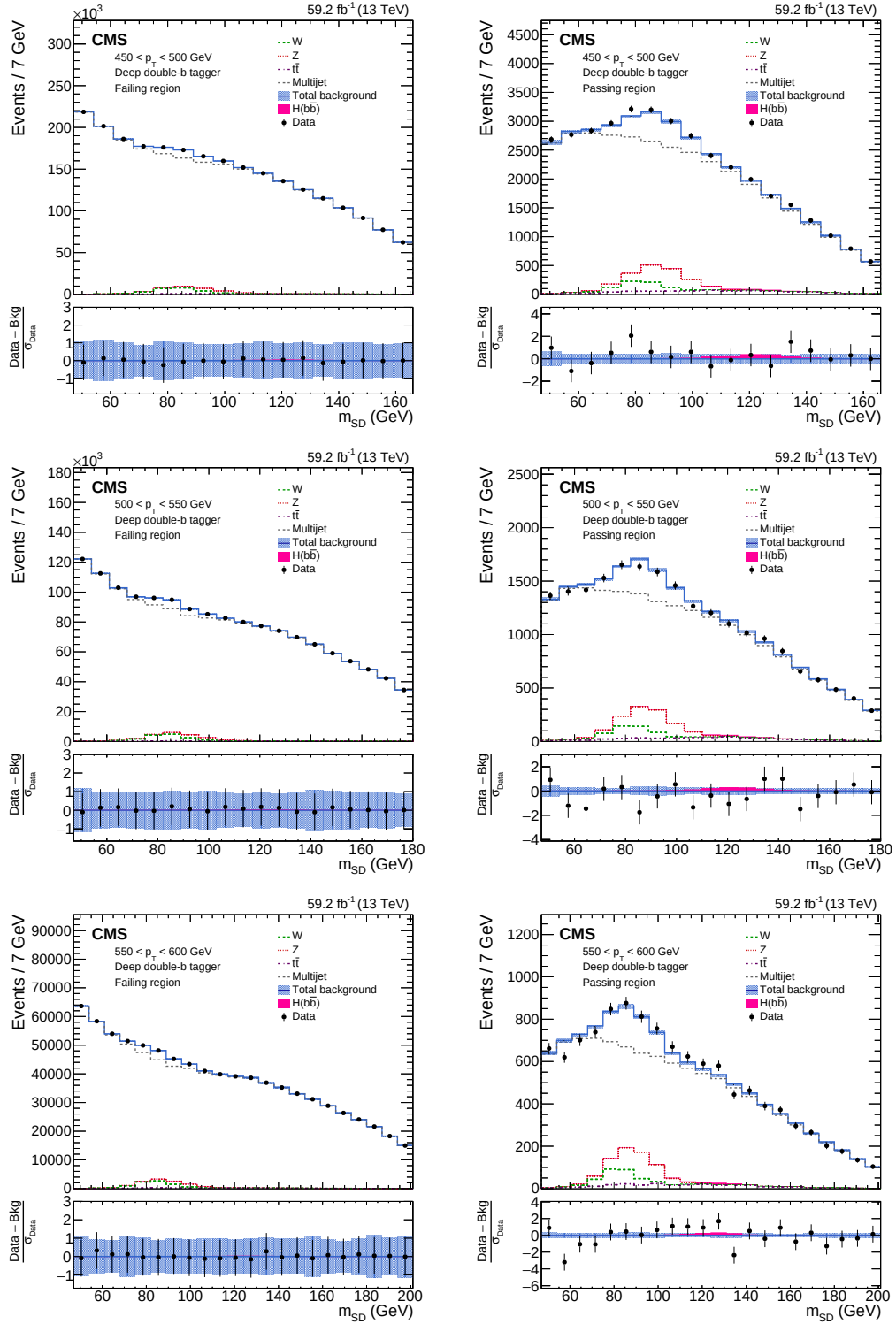
Figure B.5: Post-fit m_{SD} distributions in the full 2018 dataset for the pass and fail regions and the first three p_T categories (450-500, 500-550, 550-600 from top to bottom) by using a polynomial 1st order in \rho and 1st order in p_T . The EW and signal events are also shown separately.
