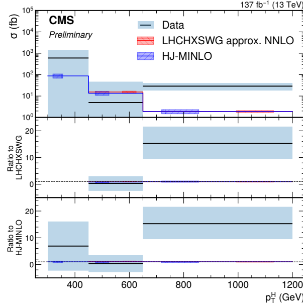
Figure 4.78: Measured differential fiducial cross section as a function of Higgs boson p_T , in comparison to the predictions of Ref. [86] and HJ-MINLO [105]. In the bottom two panels, the dotted line corresponds to a ratio of one. The measured cross section uncertainty in the first bin is larger because of limited acceptance. The cross section measurements in the first and second bins have a mild anti-correlation, primarily due to jet energy scale uncertainties, which inflates the corresponding uncertainties. The observed cross section in the third bin has a smaller relative uncertainty than that in the second bin because of the larger magnitude of the central value in that bin. The relative uncertainties in the predictions of Ref. [86] and HJ-MINLO are approximately 10% and 20%, respectively.
