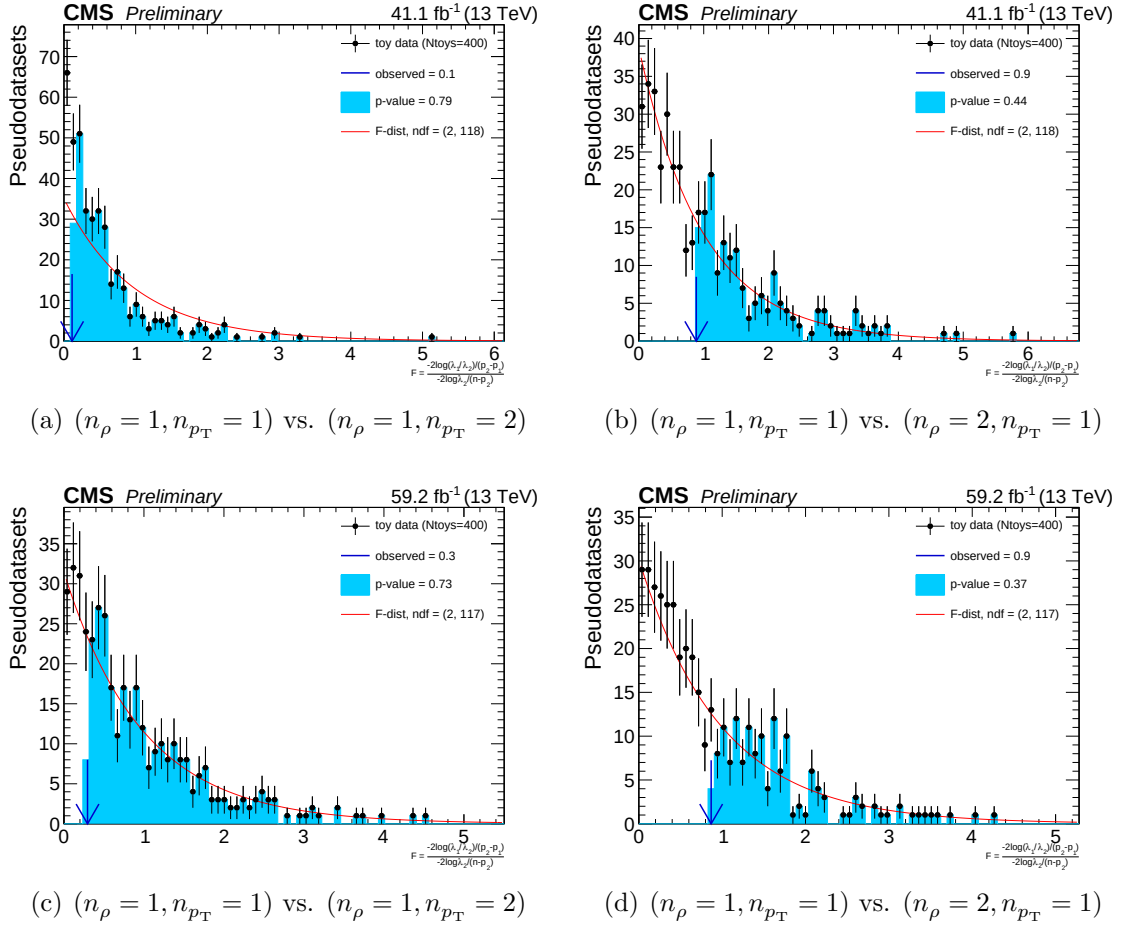
Figure 4.42: The F -test for different hypotheses on the 2017 (top) and 2018 (bottom) dataset.
