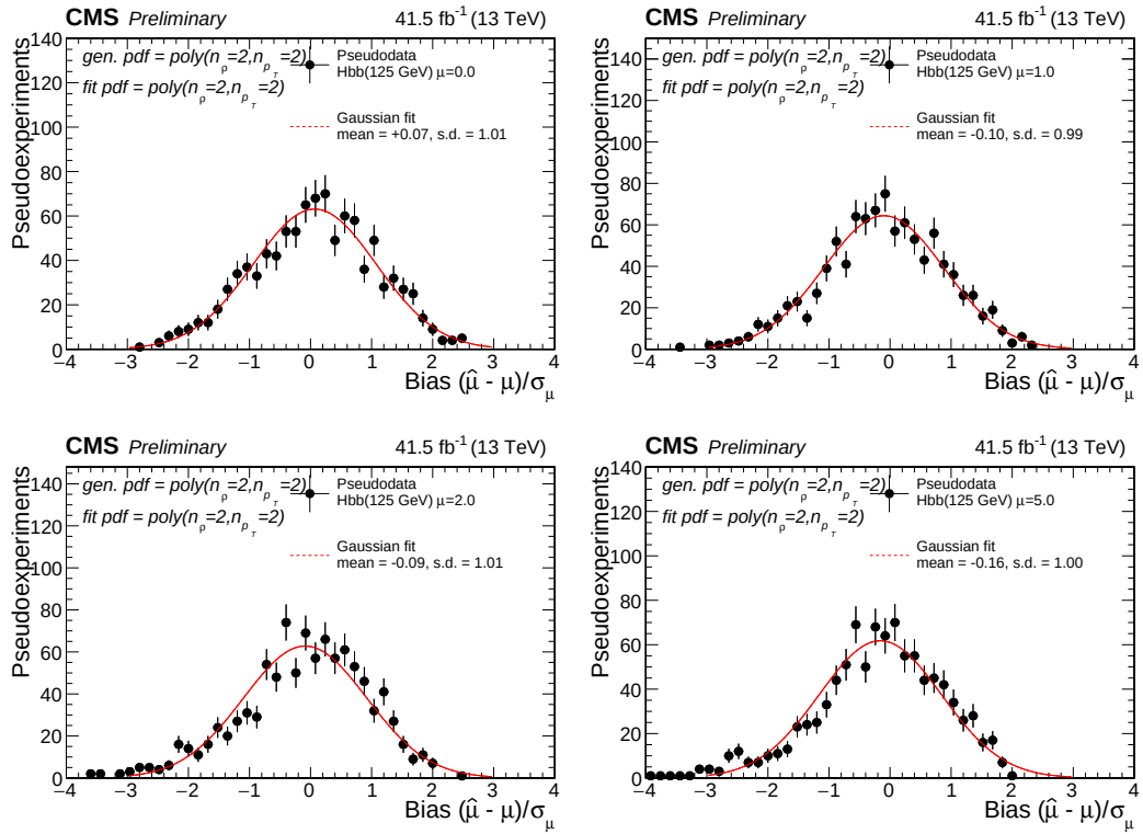
Figure 4.51: The pull distribution when generating and fitting with the nominal function. Plots are shown for different injected H(b\bar{b}) signal strengths: \mu_H = 0, 1, 2, 5 .
