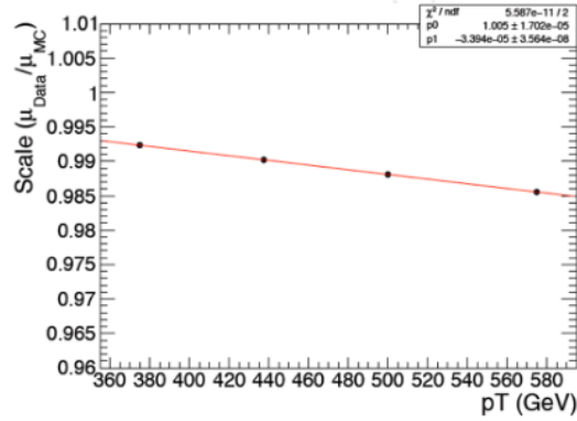
Figure 4.56: p_{\text{T}} dependence of the mass scale SF measured in the merged-W jet sample.
