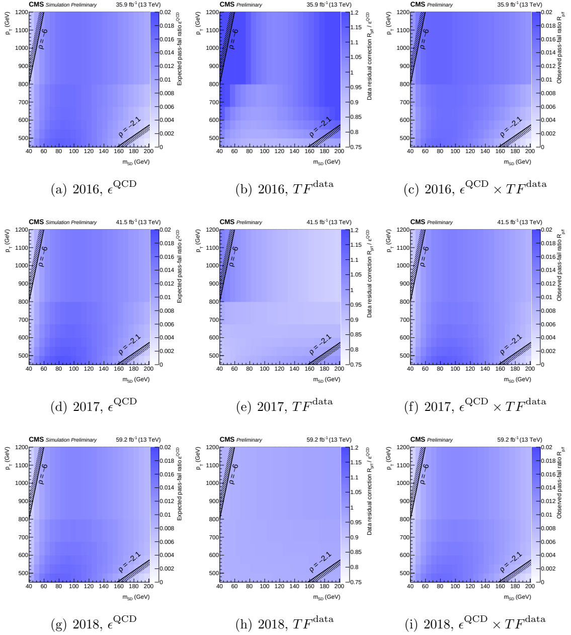
Figure C.1: The top(middle/bottom) rows correspond to quantities detailed below, corresponding to data collected in 2016(2017/2018) condition respectively. (Left) The expected pass-fail ratio \epsilon^{\text{QCD}} as a function of jet p_T and m_{\text{SD}} for QCD multijet simulation. (Middle) The correction TF^{\text{data}} for residual differences between data and simulation as a function of jet p_T and m_{\text{SD}} (Right) The fitted pass-fail ratio R_{\text{p/f}} as a function of jet p_T and m_{\text{SD}} . The ratio relates the QCD multijet event yield in the passing region to that of the failing region. The pass-fail ratio is the product of the previous two components.
