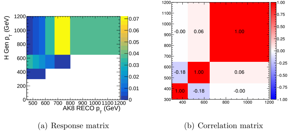
Figure 4.79: (a) Response matrix corresponding to the STXS binning of the generated Higgs p_T . Reconstructed p_T binning is fixed to the p_T categories defined in the analysis. The z -axis value quantifies the fraction of events in a given reconstructed p_T bin for the given generated p_T bin, normalized to the total production rate in the generated p_T bin. (b) Correlation between per- p_T -bin signal strength parameters corresponding to the STXS binning of the generated Higgs p_T .
