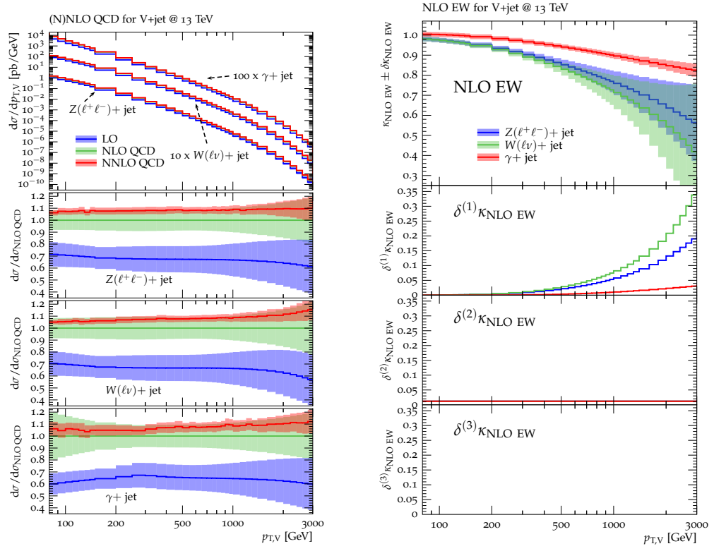
Figure 4.1: NLO QCD (left) and EW (right) corrections and the corresponding uncertainties. Ref [79]
