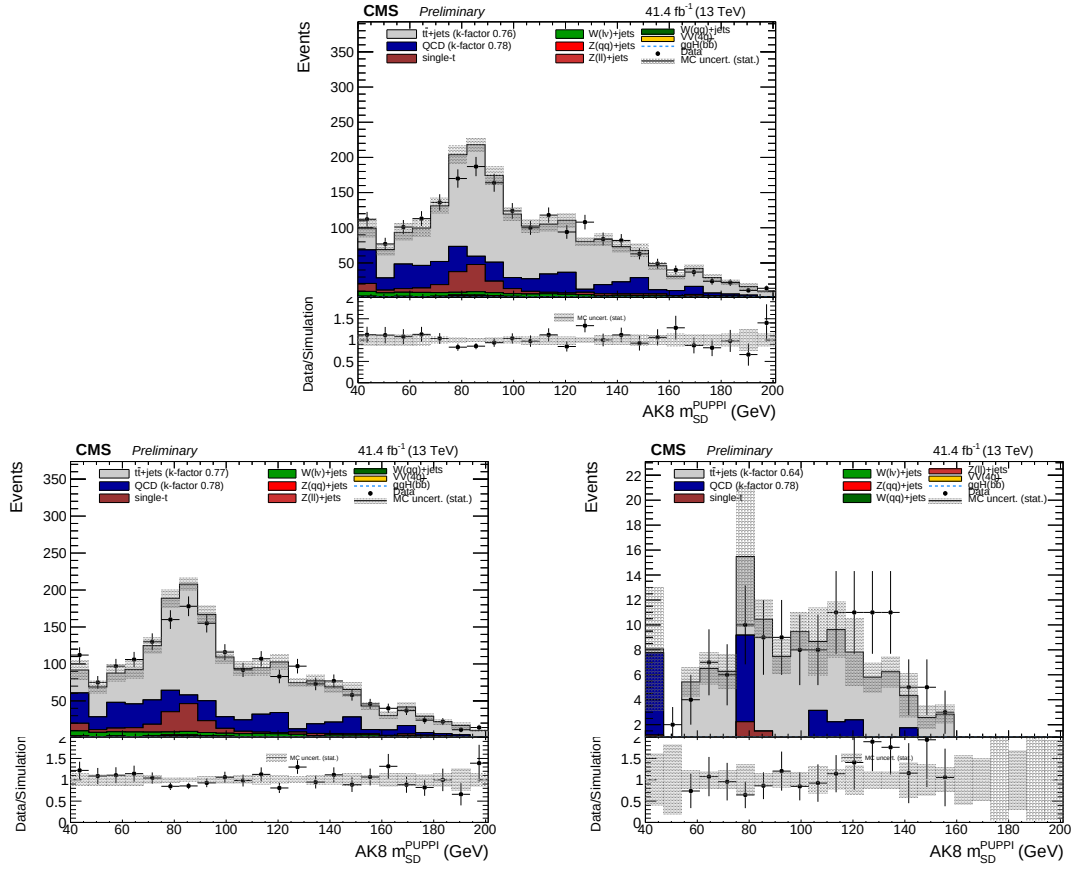
Figure 4.37: Single muon control region for t\bar{t} background in 2017 data. (Top) Inclusive in deep double-b tag. (Bottom left) Failing region with deep double-b tag < 0.89 . (Bottom right) Passing region with deep double-b tag > 0.89 . QCD is scaled down by a k-factor of 0.78 and t\bar{t} is scaled to same integral as data.
