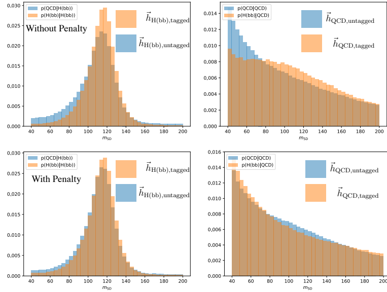
Figure 3.25: The weighted, normalized mass distributions for the "tagged" and "untagged" background and signal before adding the KL divergence penalty terms to the training (top) and after adding the KL divergence penalty terms to the training (bottom).
