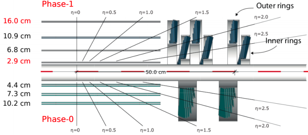
Figure 3.6: Comparison of the layouts of the Phase-1 pixel detector (top) and the original pixel detector before the year-end technical stop between 2016 and 2017 (bottom) [37].
