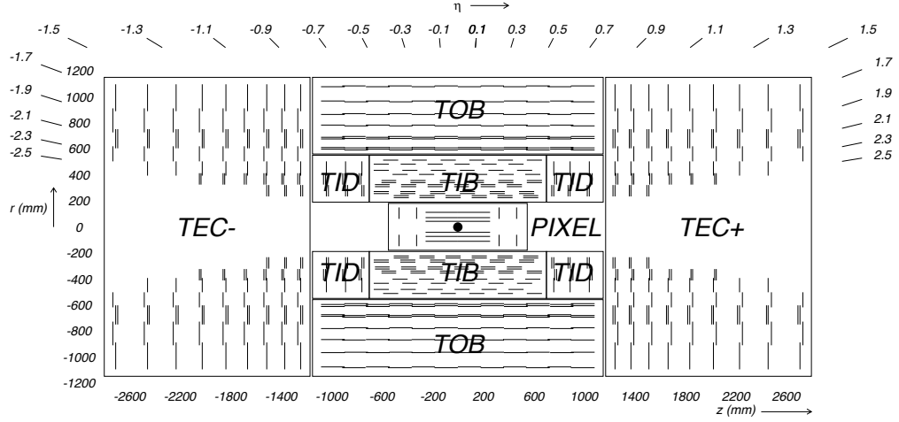
Figure 3.7: Schematic diagram the CMS tracker [34].
