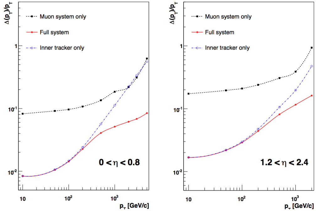
Figure 3.20: Muon transverse momentum resolution as a function of muon transverse momentum [37].
