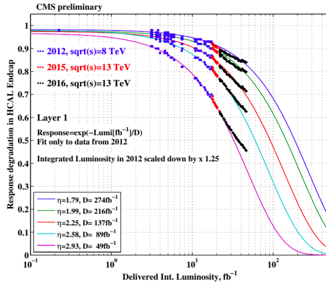
Figure 3.10: Response of the HE scintillators tiles as a function of the delivered integrated luminosity for several pseudorapidity values. The blue, red and black dots represent response measurements performed during 2012, 2015, and 2016, respectively. The colored lines are fits to the 2012 measurements for different \eta values [42].
