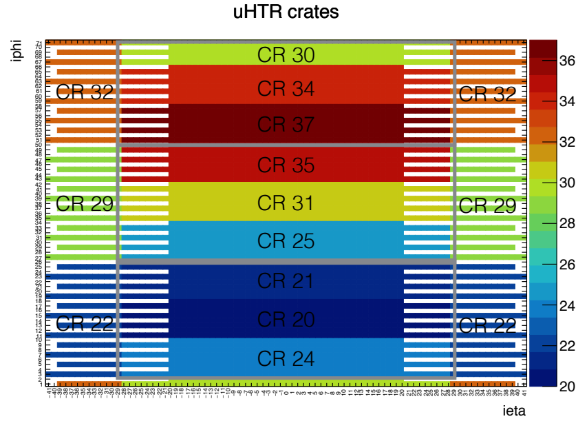
Figure 3.13: Map of HCAL (HB, HE and HF only) backend electronics structure, called uHTR crates, in the \eta - \phi plane segmented in HCAL granularity. Each grid corresponds to one read-out channel. The gray boxes covers the crates corresponding to the partition HBHEa, HBHEb and HBHEc, whereas the crates in the large \eta regions belongs to HF.
