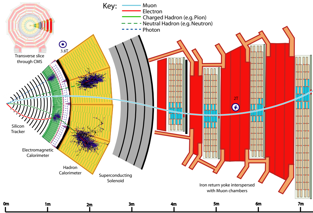
Figure 3.18: Diagram of how different particles traverse different detector components in the CMS detector [37].
