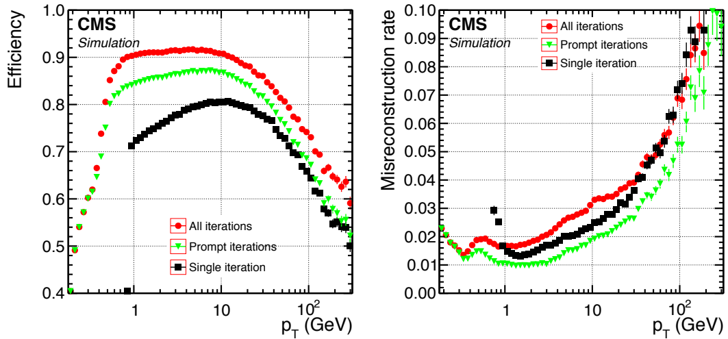
Figure 3.19: Efficiency (left) and misreconstruction rate (right) of global combinatorial track finder at different iterations as a function of track p_T [44].
