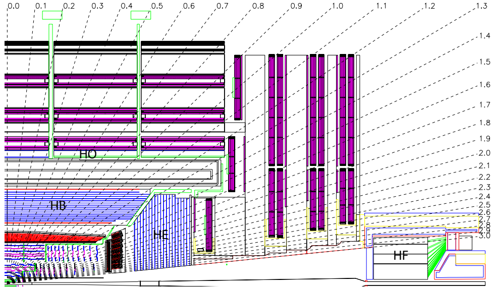
Figure 3.9: Layout of the CMS hadronic calorimeter [37].
