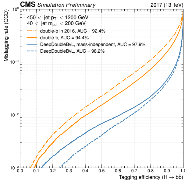
Figure 4.19: ROC curve for double-b evaluated on 2017 MC (orange), double-b evaluated on 2016 MC (orange dashed) and deep double-b (decorrelated) taggers, evaluated on 2017 MC.
