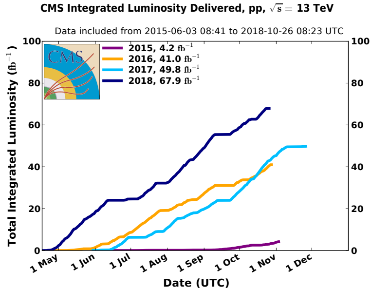
Figure 3.4: Cumulative luminosity versus day delivered to CMS during stable beams for pp collisions in LHC Run II.
