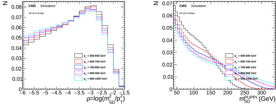
Figure 3.22: Distribution of \rho (left) and m_{\text{SD}} (right), shown for QCD MC for different p_T bins.
