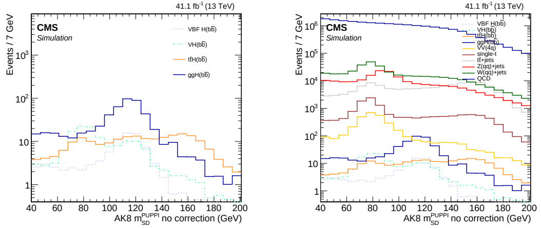
Figure 4.12: Uncorrected soft drop mass distribution for the p_T -leading jet. Left, simulated signal events normalized to their cross sections (Table 4.4). Right, background and signal events normalized to their cross sections.
