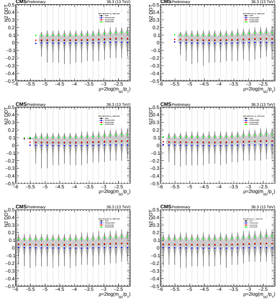
Figure 4.16: N_2^{1,DDT} kinematic dependence as a function of \rho in different p_T bins: p_T :450-500 GeV (top-left), p_T :500-550 GeV (top-right), p_T :550-600 GeV (middle-left), p_T :600-675 GeV (middle-right), p_T :675-800 GeV (bottom-left), p_T :800-1000 GeV (bottom-right). The blue points represent again the 26% quantile value of N_2^{1,DDT} , which by construction is flat as function of \rho .
