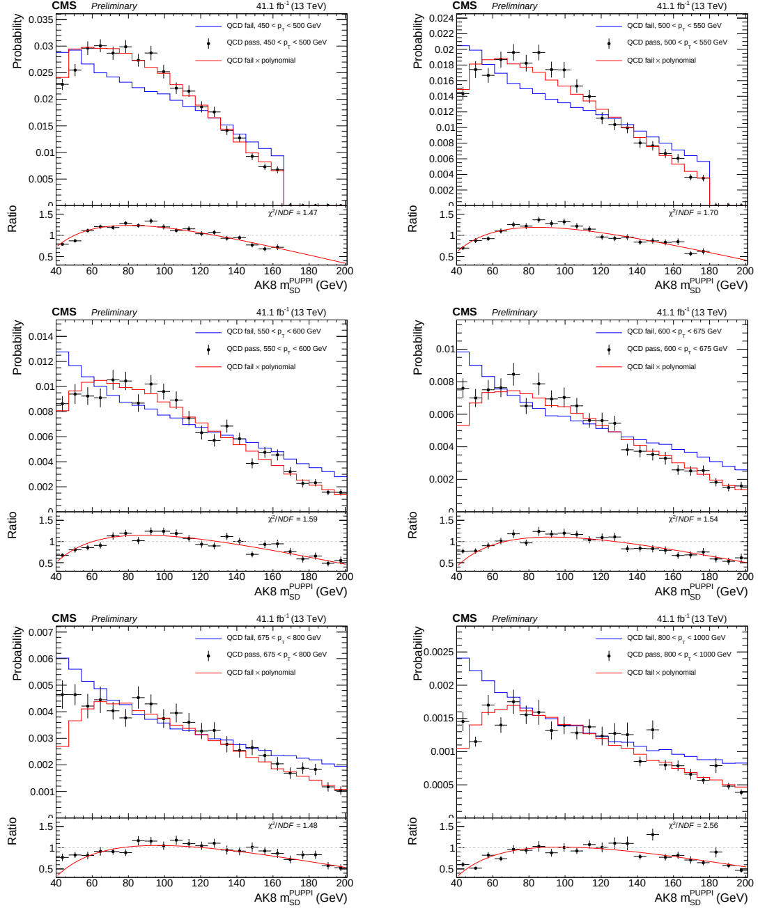
Figure 4.39: m_{SD} distributions of the QCD MC in the pass and fail regions (top panel) and their ratio (bottom panel) in each p_T category. This polynomial TF is used to derive the QCD prediction (shown in red) for the pass region (defined as the fail region distribution times the polynomial). The \chi^2 reported here refers to the compatibility between shapes in the pass and fail regions.
