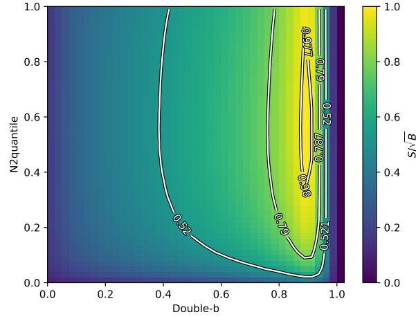
Figure 4.26: Scan of relative S/\sqrt{B} for the deep double-b tagger and N_2^{\text{1,DDT}} substructure cuts, using simulated multijet QCD and ggF H(b\bar{b}) signal events. The white contours show the value of S/\sqrt{B} . The maximum occurs near deep double-b values of 0.86 – 0.90 and N_2^{\text{1,DDT}} quantiles of 0.38 – 1
