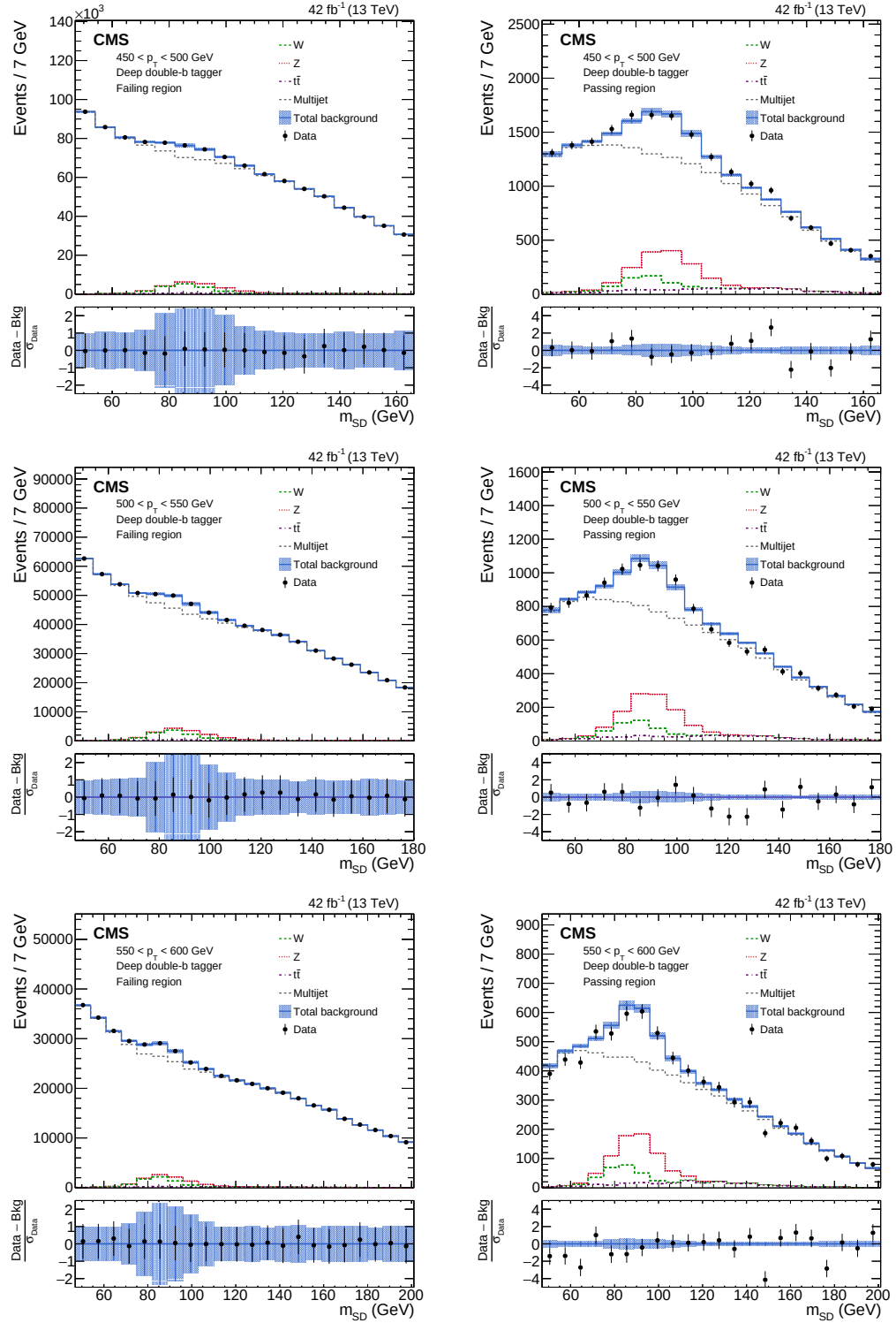
Figure 4.46: Post-fit m_{SD} distributions in simulated MC events corresponding to 2017 conditions for the pass and fail regions and the first three p_T categories (450-500, 500-550, 550-600 from top to bottom) by using a polynomial 2nd order in \rho and 2nd order in p_T . The EW and signal events are also shown separately.
