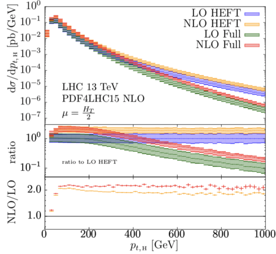
Figure 4.3: Transverse momentum distribution of the Higgs boson at the LHC with \sqrt{s} = 13 TeV computed in Ref. [84]. The upper panel shows absolute predictions at LO and NLO in the full SM and in the infinite top-mass approximation (EFT). The lower panel shows respective NLO/LO correction factors. The bands indicates theoretical errors of the full SM result due to scale variation.
