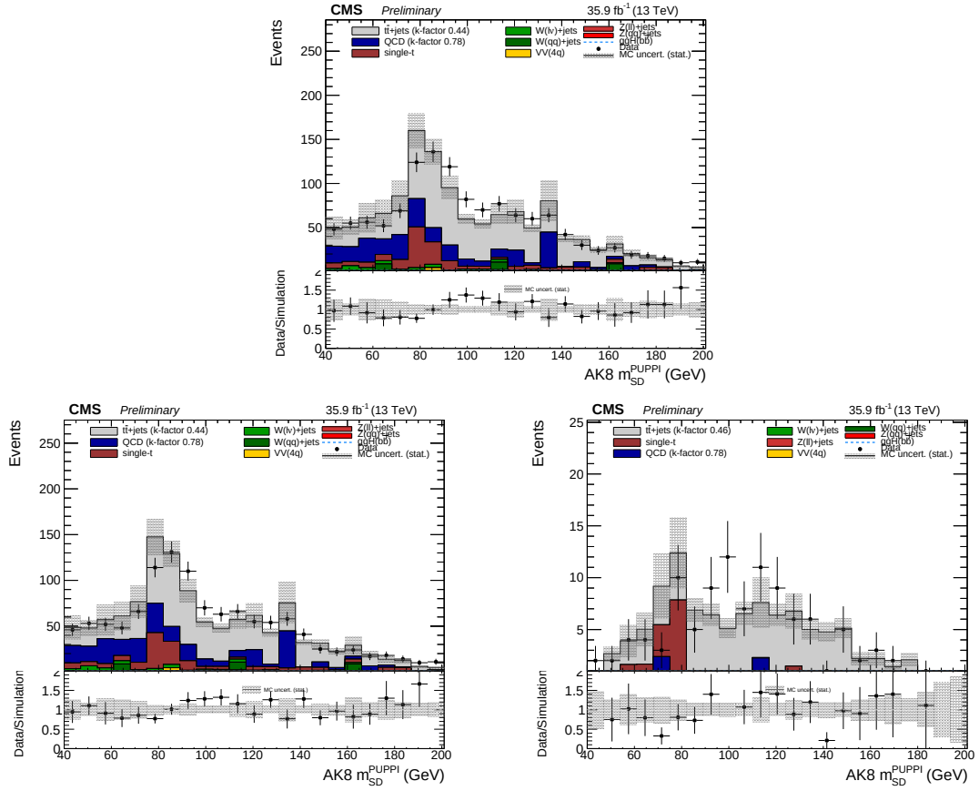
Figure 4.36: Single muon control region for t\bar{t} background in 2016 data. (Top) Inclusive in deep double-b tag. (Bottom left) Failing region with deep double-b tag < 0.89 . (Bottom right) Passing region with deep double-b tag > 0.89 . QCD is scaled down by a k-factor of 0.78 and t\bar{t} is scaled to same integral as data.
