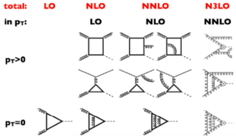
Figure 2.6: Part of the Feynman diagrams involved in predicting Higgs production cross section at different orders.
