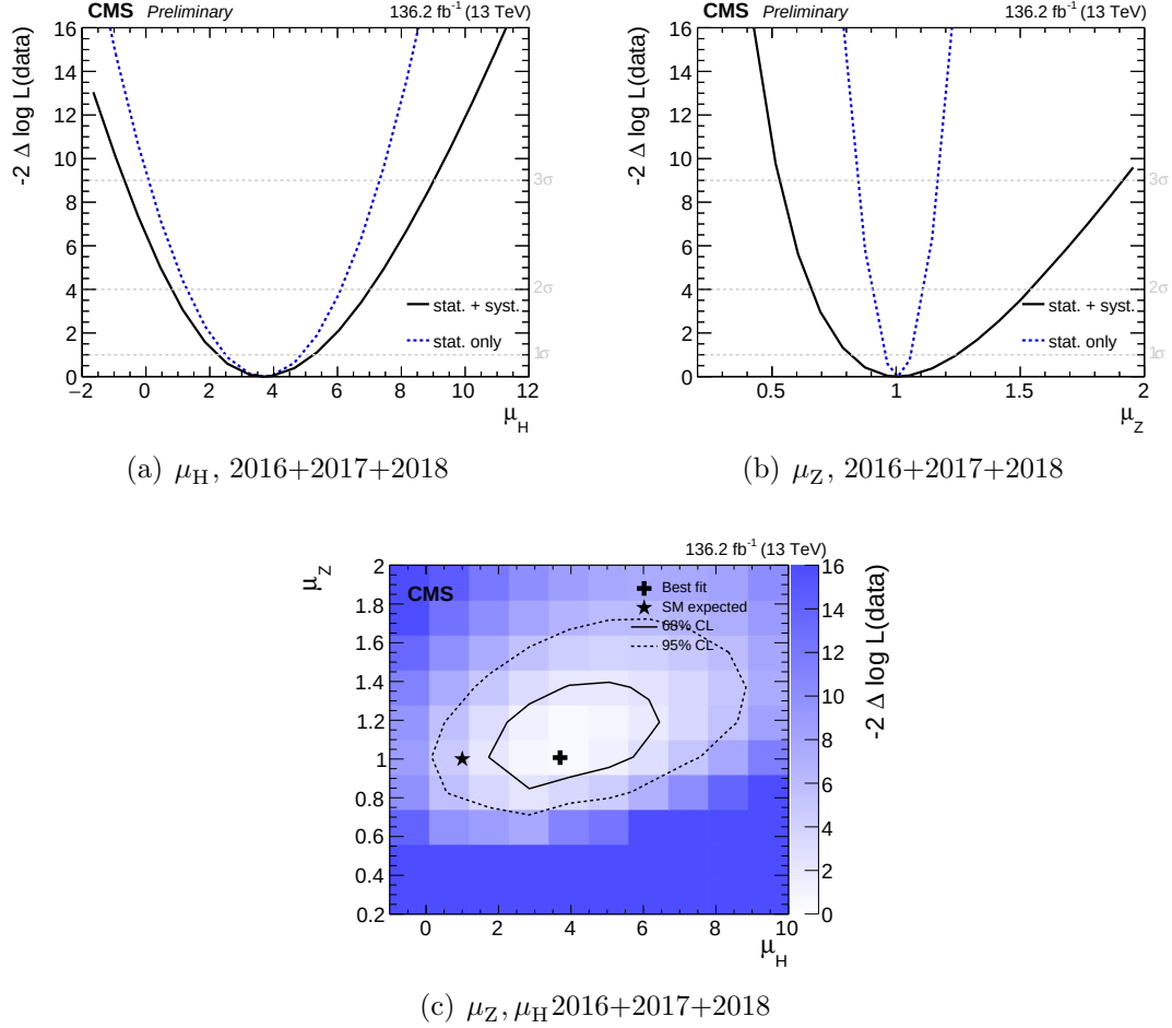
Figure 4.72: 1D profile and 2D likelihood test statistic -2\Delta \log(\mathcal{L}) scans as a function of the signal strengths \mu_H and \mu_Z on data for 2016+2017+2018. In the 1D profile, the solid black curve, labeled “stat+syst,” corresponds to the scan when profiling all nuisance parameters and the dotted blue curve, labeled “stat only,” corresponds to only profiling the unconstrained nuisance parameters, such as the QCD transfer factor parameters.
