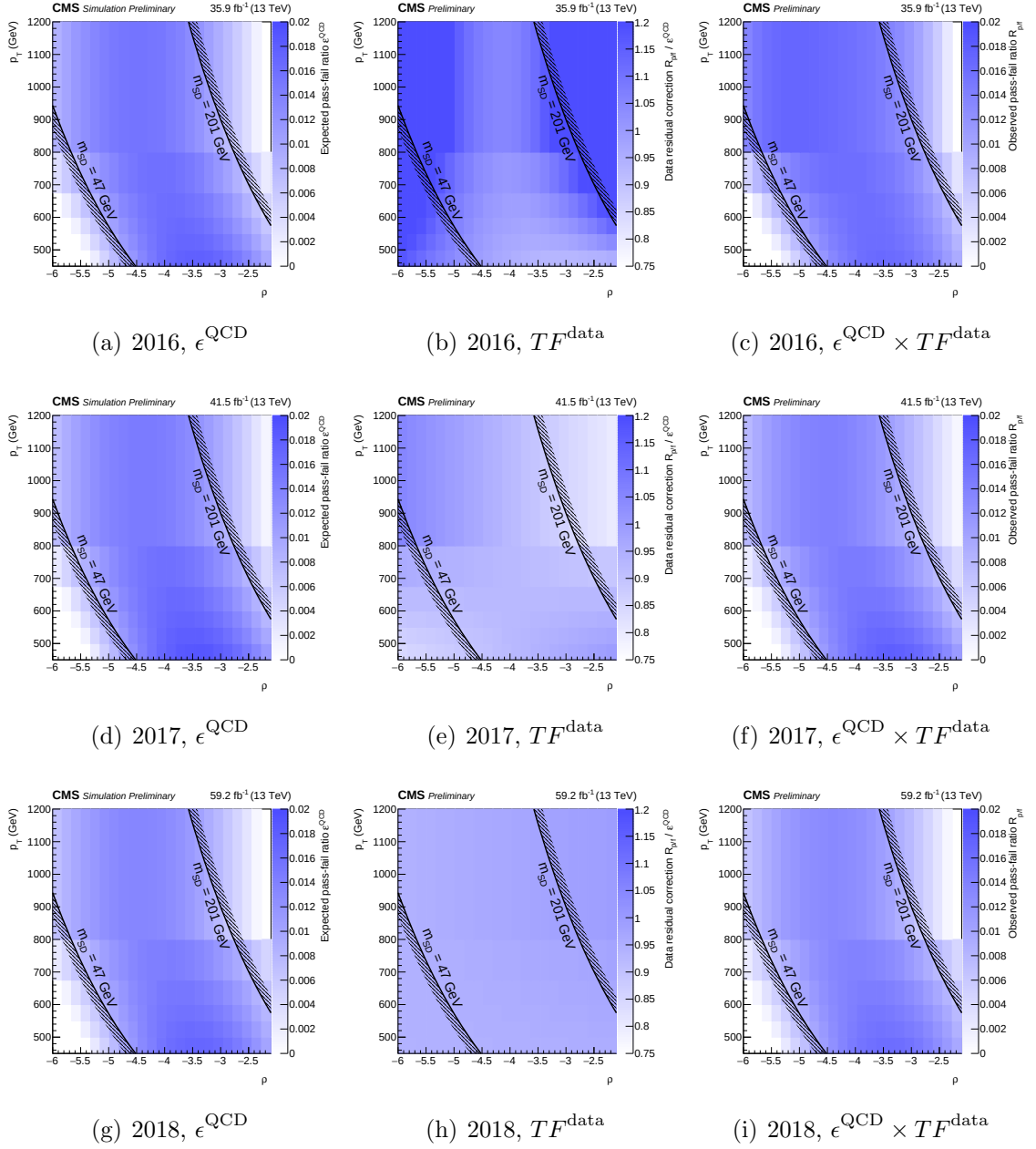
Figure C.2: The top(middle/bottom) rows corresponds to quantities detailed below, corresponding to data collected in 2016(2017/2018) condition respectively. (Left) The expected pass-fail ratio \epsilon^{\text{QCD}} as a function of jet p_T and \rho for QCD multijet simulation. (Middle) The correction TF^{\text{data}} for residual differences between data and simulation as a function of jet p_T and \rho (Right) The fitted pass-fail ratio R_{p/f} as a function of jet p_T and \rho . The ratio relates the QCD multijet event yield in the passing region to that of the failing region. The pass-fail ratio is the product of the previous two components.
