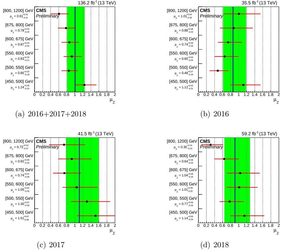
Figure 4.74: The best-fit Z signal strength \mu_Z and uncertainty per p_T category extracted from a simultaneous fit of all channels, performed on different data taking periods. The H signal strength \mu_H is also floating in these fits.
