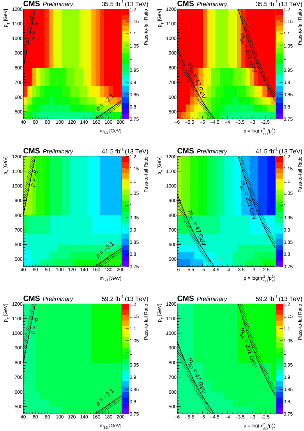
Figure 4.68: The fitted data-mc transfer function TF^{\text{data}} as a function of p_T and m_{SD} (left) or p_T and \rho (right) for 2016 (top), 2017 (middle), and 2018 (bottom) data. The polynomial orders of used these functions are 1st order in p_T and 1st order in \rho for 2017 and 2018, while the order in p_T and \rho are 2nd order and 1st order for 2016 respectively.
