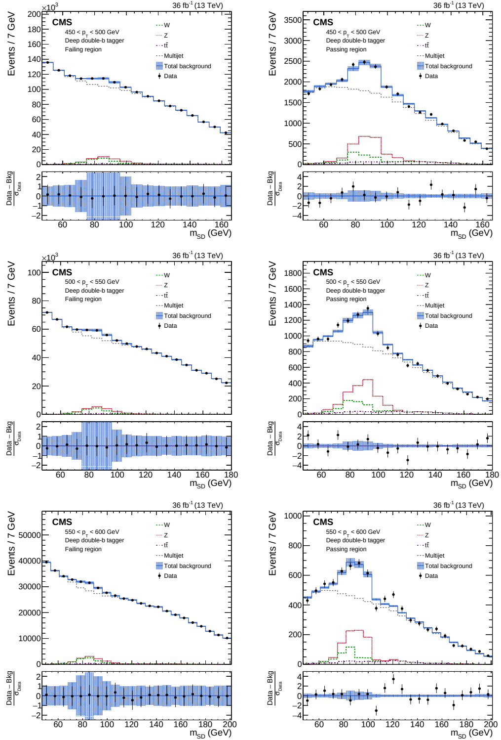
Figure 4.44: Post-fit m_{SD} distributions in simulated MC events corresponding to 2016 conditions for the pass and fail regions and the first three p_T categories (450-500, 500-550, 550-600 from top to bottom) by using a polynomial 2nd order in \rho and 2nd order in p_T . The EW and signal events are also shown separately.
