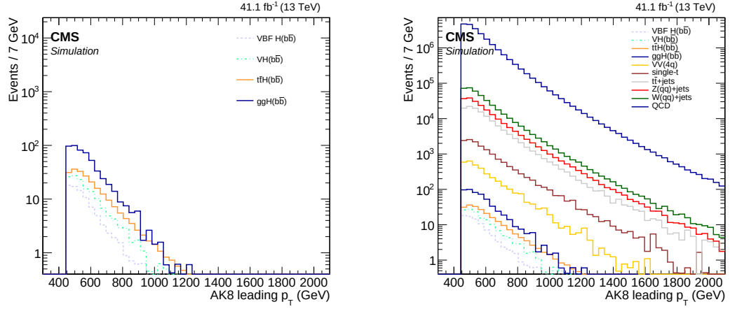
Figure 4.11: AK8 jet p_T distribution. Left, simulated signal events normalized to their cross sections (Table 4.4). Right, background and signal events normalized to their cross section.
