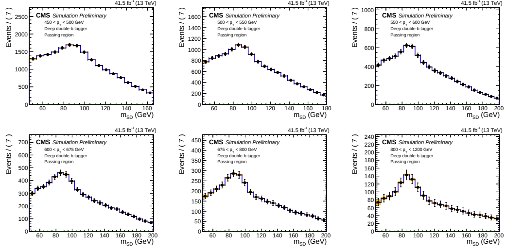
Figure 4.53: R_{p/f} TF function signal+background fit to the pass category directly with the 2017 MC.
