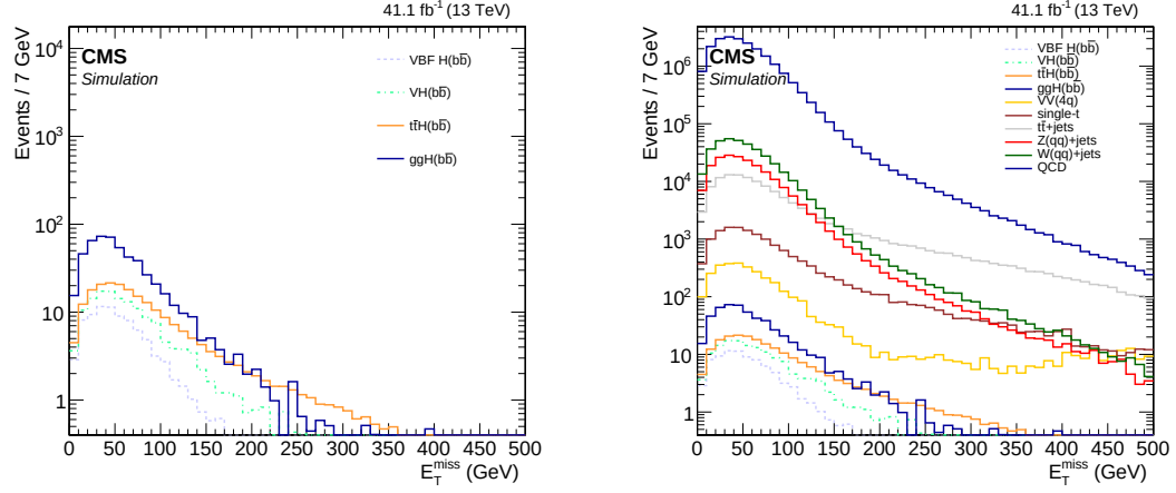
Figure 4.24: E_T^{\text{miss}} distributions. Left, simulated signal events normalized to their cross sections (Table 4.4). Right, background and signal events normalized to their cross sections.
