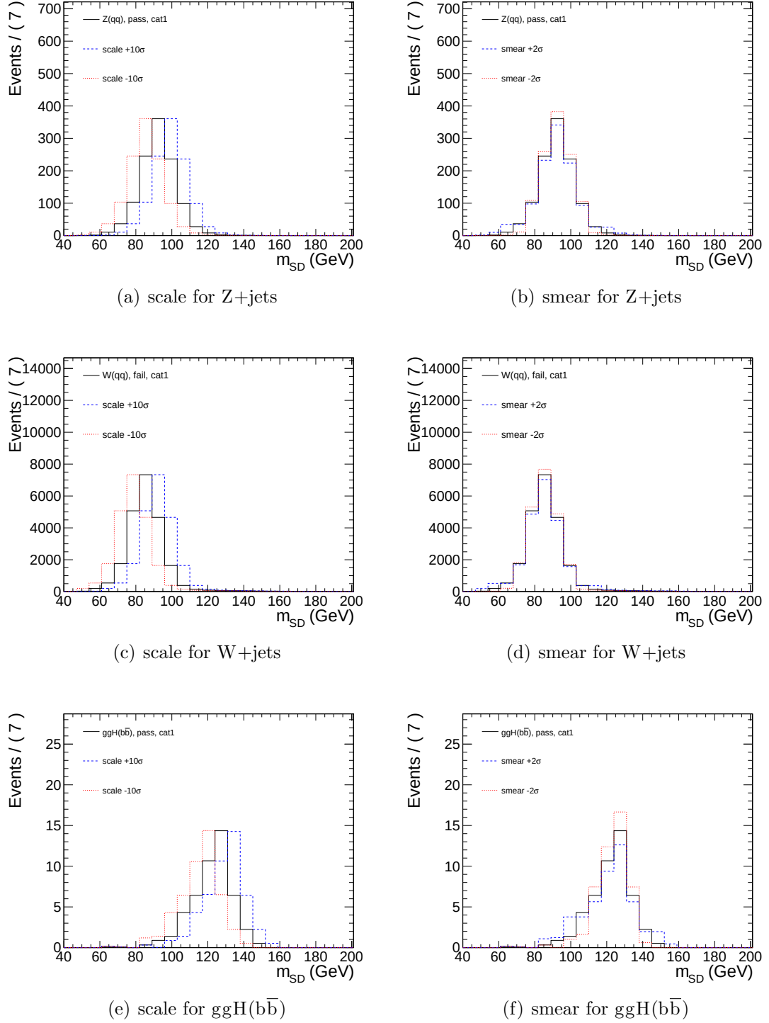
Figure 4.55: Effect of varying the jet mass scale by \pm 10\sigma and the jet mass resolution by \pm 2\sigma for W/Z+jets and the signal ggH(b\bar{b}) in p_T category 1 ( 450 < p_T < 500 GeV).
