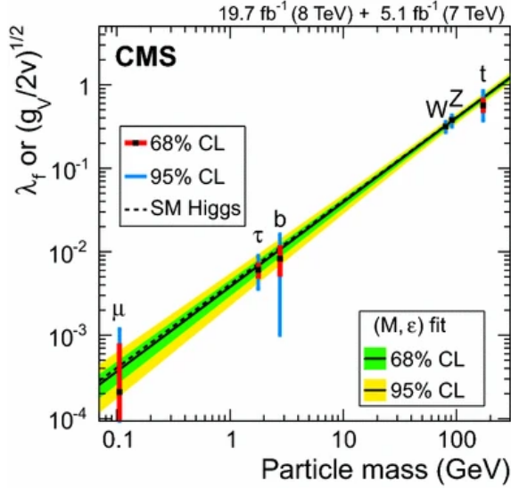
Figure 2.5: Coupling strengths of Higgs boson as a function of particle masses, extracted using LHC run 1 data [25]. Note that the uncertainties on fermionic couplings are significantly larger than the ones in W and Z.
