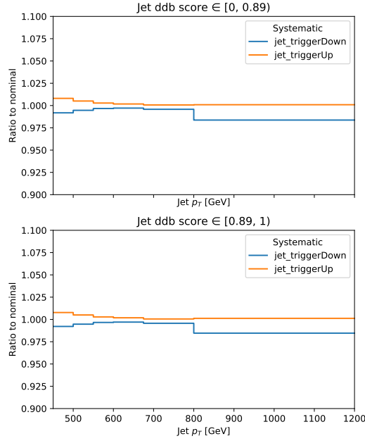
Figure 4.61: Relative effect of the jet trigger systematic uncertainty on the expected event yield, per jet p_T bin in the signal region. The effect is shown separately for events in the AK8 deep double-b passing (bottom) and failing (top) regions. The effect is as measured in a sample of Z+jets events simulated with 2017 data-taking conditions and corrected by the 2017 jet trigger efficiency as measured in an independent control sample.
