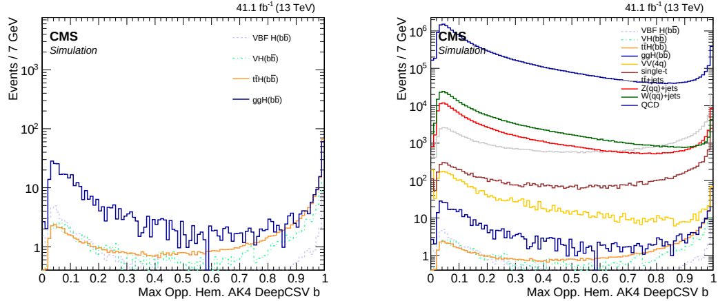
Figure 4.23: Distribution of the maximum DeepCSV discriminator value for the four leading- p_T AK4 jets in the opposite hemisphere from the leading- p_T AK8 jet. Note, the medium working point discriminator cut value is 0.4941 for 2017 data. Left, simulated signal events normalized to their cross sections (Table 4.4). Right, background and signal events normalized to their cross sections.
