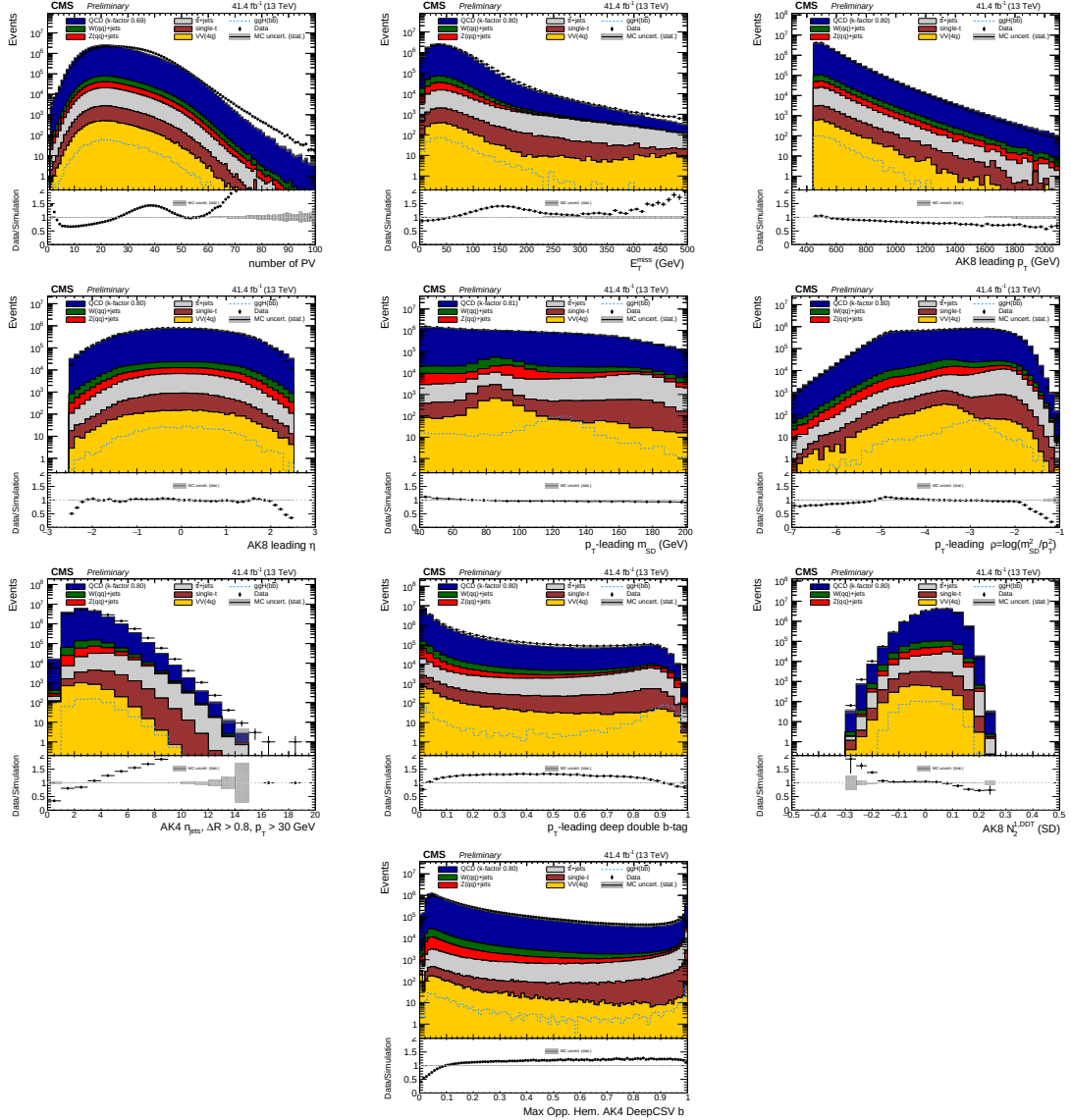
Figure 4.31: Distributions of variables in 2017 data and simulated samples after the kinematic preselection. From top to bottom: number of primary vertices, E_T^{\text{miss}} , p_T , \eta , m_{\text{SD}} , deep double-b tagger, N_2^{\text{DDT}} , and the t\bar{t} rejection variable. The VV(4q) category is mislabeled, and represents instead inclusive diboson production. The background processes, QCD(blue), W+jets(green), Z+jets(red), t\bar{t} (grey), single-top(brown) and diboson(yellow), are shown as stacked distributions.
