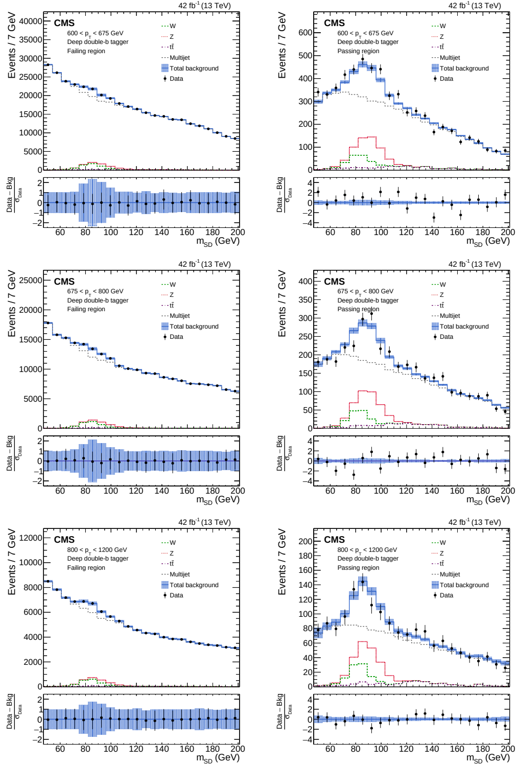
Figure 4.47: Post-fit m_{SD} distributions in simulated MC events corresponding to 2017 conditions for the pass and fail regions and the second three p_T categories (600-675, 675-800, 800-1200 from top to bottom) by using a polynomial 2nd order in \rho and 2nd order in p_T . The EW and signal events are also shown separately.
