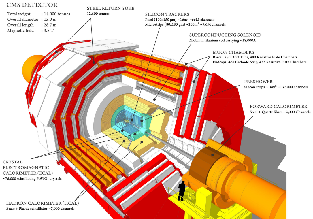
Figure 3.5: Cut-out diagram of the CMS detector [34].
