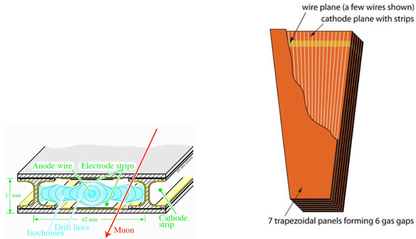
Figure 3.16: Diagram of basic unit of DT and CSC system, showing the drift cell (left) and cathode stripe chamber (right) [37].
