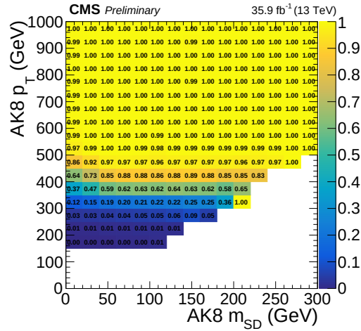
Figure 4.5: Measured trigger efficiency of the “OR” as function of jet p_T and jet m_{SD} is shown for 2016.
