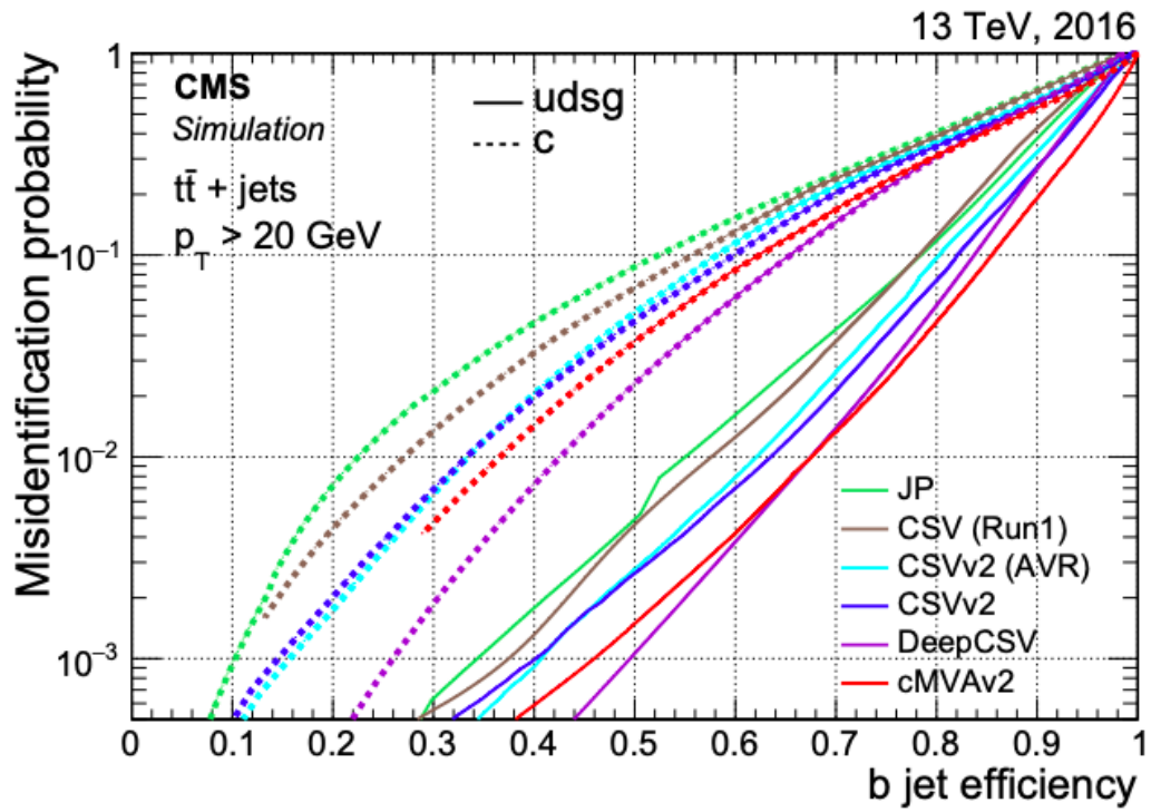
Figure 3.24: Receiver operating characteristic (ROC) curve comparing the performance of different b-tagging algorithms in CMS [65].
