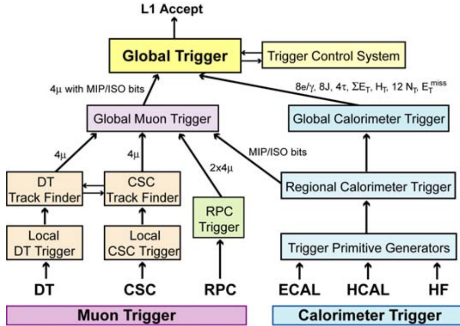
Figure 3.17: Level-1 Trigger system architecture [37].
