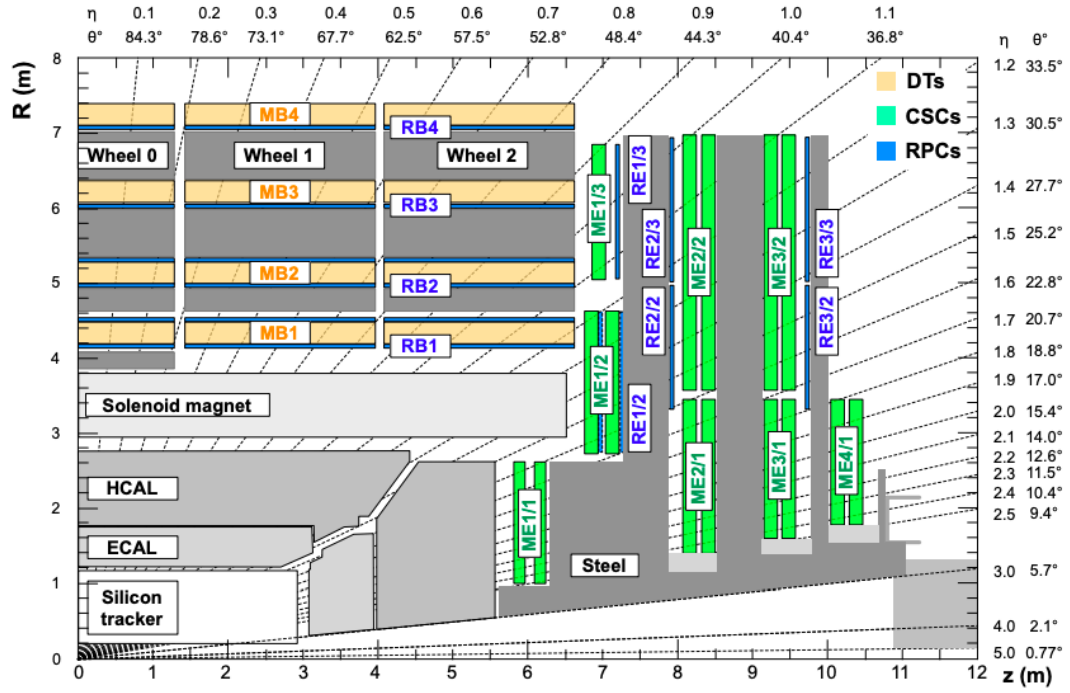
Figure 3.15: Layout of the CMS muon system [37].
