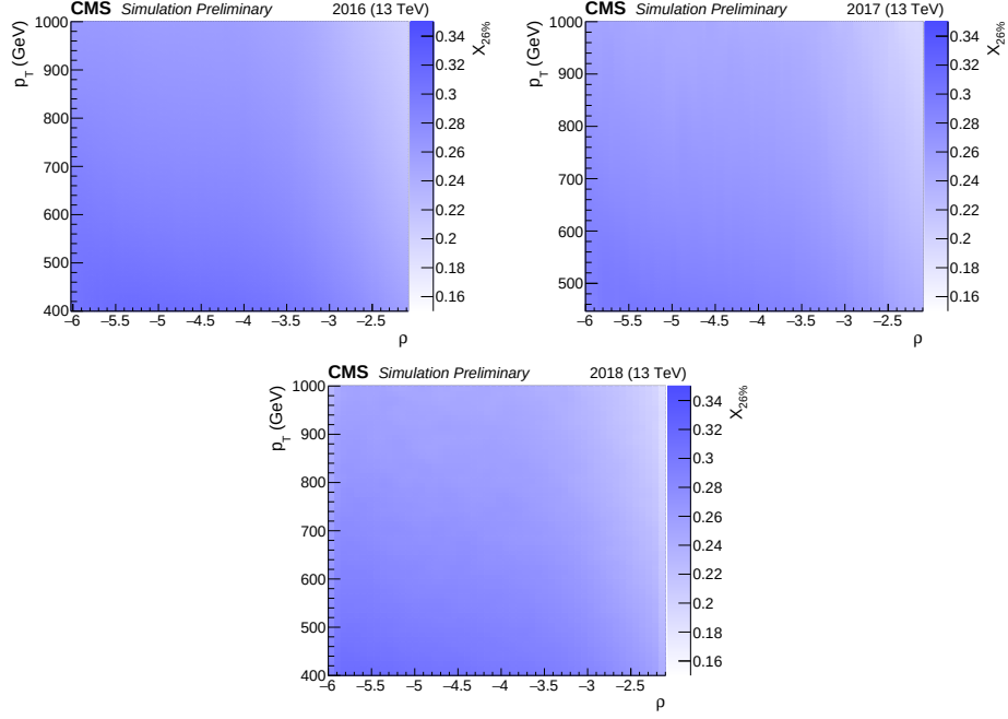
Figure 4.17: Transformation maps of N_2^1 \rightarrow N_2^{1,DDT} for different data-taking years (top left: 2016, top right: 2017, bottom: 2018) corresponding to the N_2^1 quantile value of 26% (i.e. for \epsilon_{QCD} = 26\% ), as a function of \rho and p_T .
