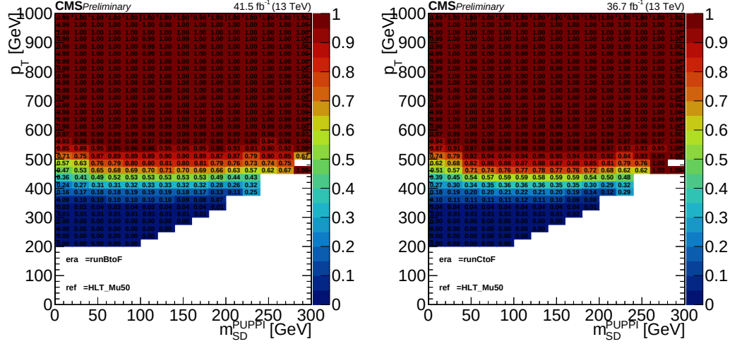
Figure 4.7: Measured trigger efficiency of the “OR” as function jet p_T and m_{SD} jet for Run 2017B-F and Run 2017C-F.
