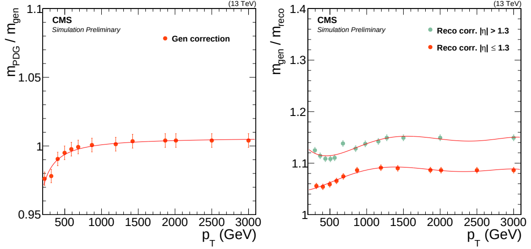
Figure 3.21: Fit to (left) M_{\text{PDG}}/M_{\text{GEN}} as a function of jet p_T , where M_{\text{PDG}} = 80.4 GeV and M_{\text{GEN}} is the fitted mean of the generator level mass and (right) M_{\text{GEN}}/M_{\text{RECO}} , where M_{\text{RECO}} is the reconstructed softdrop mass, as a function of jet p_T in two \eta bins. [58]
