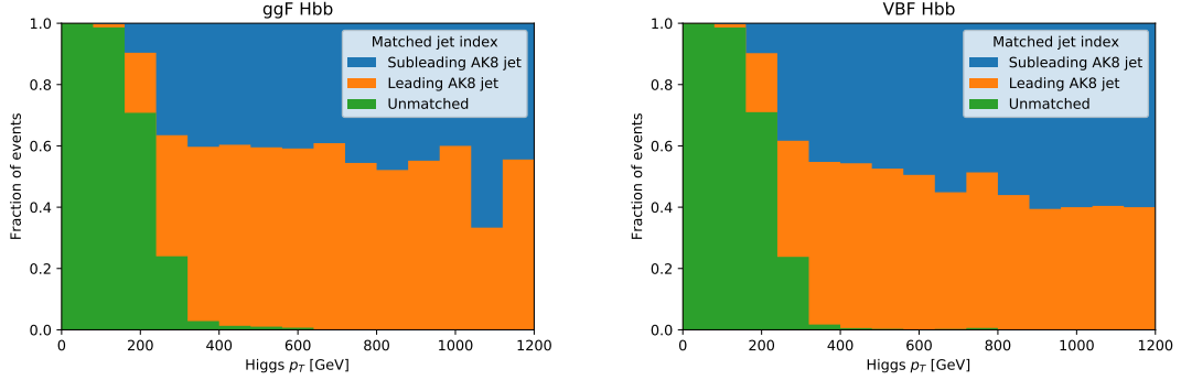
Figure 4.25: Fraction of H \rightarrow b\bar{b} events where the generated Higgs boson was found within \Delta R < 0.8 of either the leading reconstructed AK8 jet, the subleading jet, or not matched to any AK8 jet in the event, as a function of generated Higgs boson p_T . The fractions are shown separately for gluon fusion H production with the MINLO generator (left) and for VBF H production (right). Gluon fusion is the dominant production mode in the p_T > 450 GeV region, followed by VBF production.
