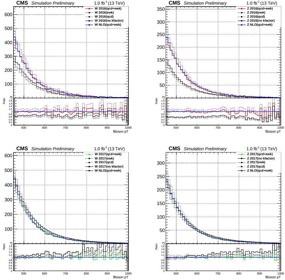
Figure 4.2: Boson p_T distributions at the generator level for W (left) and Z (right) in 2016 (upper) and 2017/18 (lower) generation configurations, showing the uncorrected spectrum, as well as the successive corrections to arrive at NLO QCD+EW. Also included is the target sample, generated as described in the text (“V NLO”), with NLO EW corrections applied. The ratio is shown with respect to the target sample.
