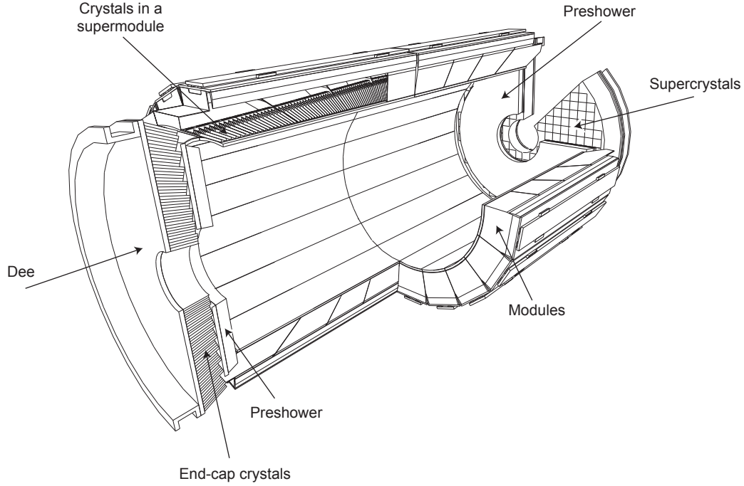
Figure 3.8: Layout of the CMS electromagnetic calorimeter [37].
