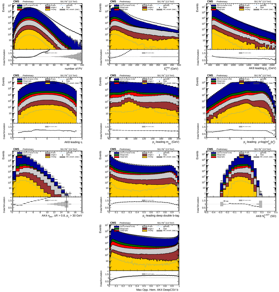
Figure 4.32: Distributions of variables in 2018 data and simulated samples after the kinematic preselection. From top to bottom: number of primary vertices, E_T^{\text{miss}} , p_T , \eta , m_{\text{SD}} , deep double-b tagger, N_2^{1,\text{DDT}} , and the t\bar{t} rejection variable. The VV(4q) category is mislabeled, and represents instead inclusive diboson production. The background processes, QCD(blue), W+jets(green), Z+jets(red), t\bar{t} (grey), single-top(brown) and diboson(yellow), are shown as stacked distributions.
