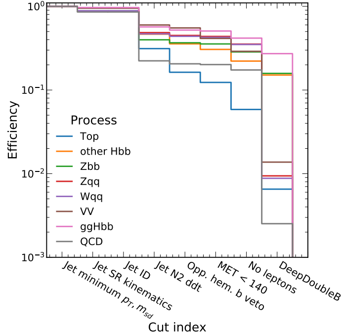
Figure 4.27: Efficiency of each of the requirement of the kinematic and top rejection selections, for simulated signal and background events.
