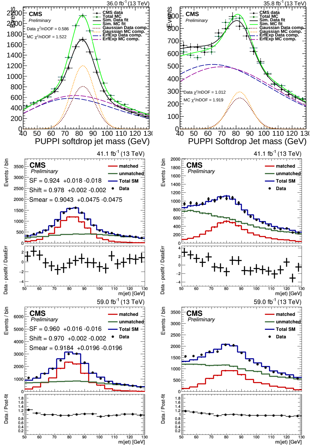
Figure 4.54: N_2^{\text{1,DDT}} Passing and failing region fits in the semileptonic t\bar{t} sample for 2016 (top), 2017 (middle) and 2018 (bottom). Note for 2016, pre-fit and post-fit models are shown, while only post-fit is shown for 2017 and 2018. In addition, the ratio panels for 2017 and 2018 correspond to different quantities.
