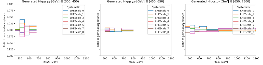
Figure 4.59: The envelope of the relative effect on signal acceptance of the 6 combinations (ignoring 0.5, 2 and 2, 0.5) about the nominal ggHbb yield, as a function of reconstructed Higgs boson p_T , for three regions in generated Higgs boson p_T . The yields are as predicted by the HJ-MINLO generator, with 2017 detector conditions.
