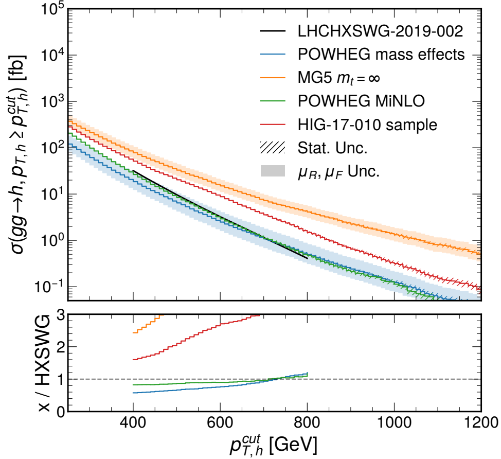
Figure 4.4: Comparison between the LHC Higgs cross section working group prescription [86] for the p_T^H spectrum and the spectrum found in several CMS datasets. The factorization and renormalization scale uncertainties were evaluated as the envelope of the 7 scale variations stored as weights in the samples. For MINLO, the weights were not available due to technical issues, and for the HIG-17-010 sample they are the same as found in the POWHEG mass effects sample. In the lower panel, the ratio of each described p_T spectrum relative to the LHCHXSWG spectrum is shown. See text for further details on the various samples.
