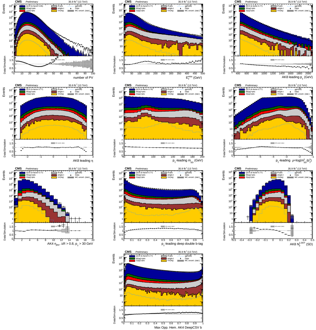
Figure 4.30: Distributions of variables in 2016 data and simulated samples after the kinematic preselection. From top to bottom: number of primary vertices, E_T^{\text{miss}} , p_T , \eta , m_{\text{SD}} , deep double-b tagger, N_2^{\text{DDT}} , and the t\bar{t} rejection variable. The VV(4q) category is mislabeled, and represents instead inclusive diboson production (yellow). The background processes, QCD(blue), W+jets(green), Z+jets(red), t\bar{t} (grey), single-top(brown) and diboson(yellow), are shown as stacked distributions.
