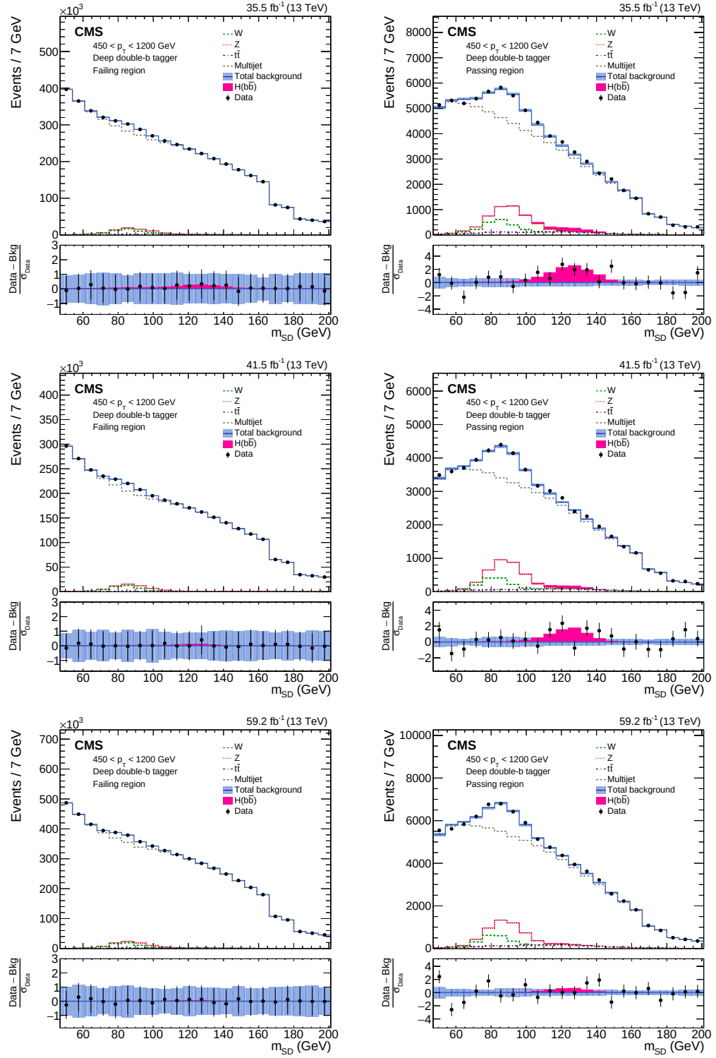
Figure B.7: Post-fit m_{SD} distributions in the full 2016, 2017, and 2018 dataset for the pass and fail regions. The EW and signal events are also shown separately.
