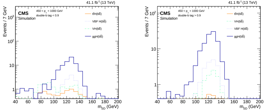
Figure 4.28: m_{SD} distribution for simulated signal events after all the selection criteria in both the failing (left) and passing (right) b-tagging categories. Each process is normalized to its cross section as shown in Table 4.4
