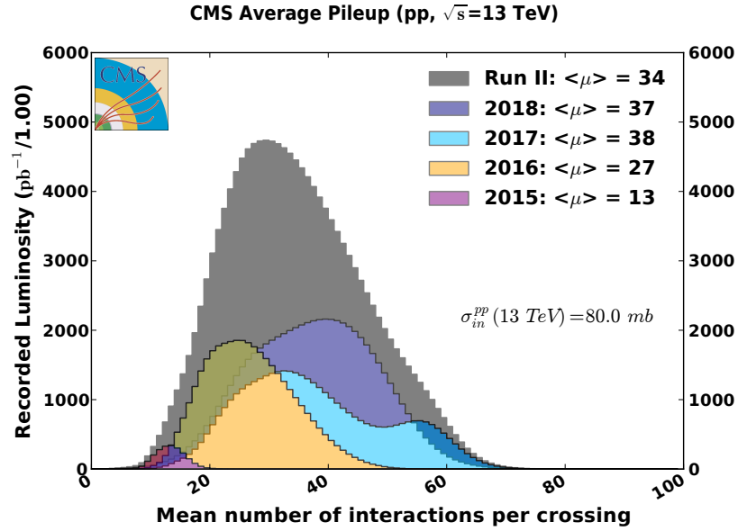
Figure 3.2: Distribution of the average number of interactions per crossing (pileup) for pp collisions in different data-taking years in the LHC Run II. The overall mean values and the minimum bias cross sections, which is pp collision cross section measured with minimum experimental selections, are also shown.
