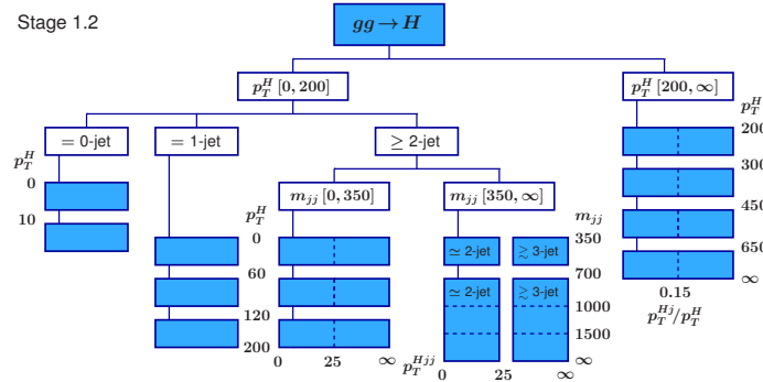
Figure 4.77: STXS Stage 1.2 binning.
