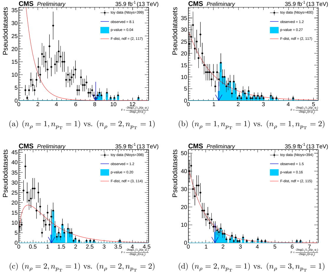
Figure 4.41: The F -test for different hypotheses on the 2016 dataset.
