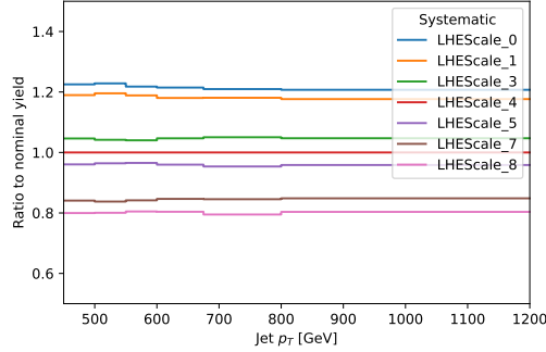
Figure 4.58: The envelope of the relative effect of the 6 combinations (ignoring 0.5, 2 and 2, 0.5) about the nominal ggHbb yield, as a function of reconstructed Higgs boson p_T . The yields are as predicted by the HJ-MINLO generator, with 2017 detector conditions.
