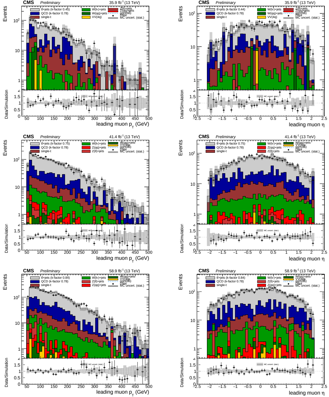
Figure 4.34: Muon p_T (left) and \eta (right) in the single muon control region for t\bar{t} background in 2016 data (top), 2017 data (middle), and 2018 data (bottom) respectively. QCD is scaled down by a k-factor of 0.78 and t\bar{t} is scaled to achieve the same overall background integral as data.
