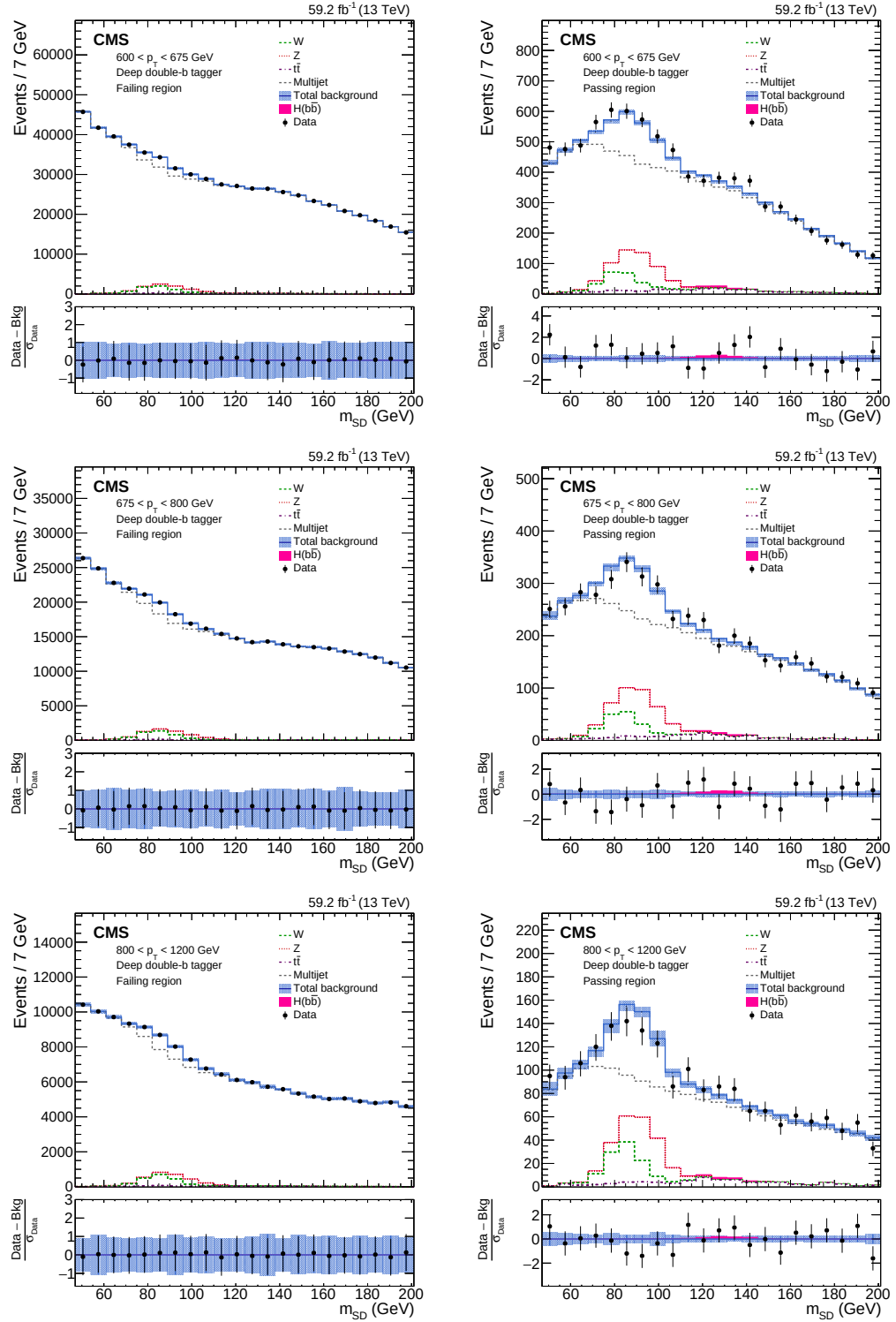
Figure B.6: Post-fit m_{SD} distributions in the full 2018 dataset for the pass and fail regions and the second three p_T categories (600-675, 675-800, 800-1200 from top to bottom) by using a polynomial 1st order in \rho and 1st order in p_T . The EW and signal events are also shown separately.
