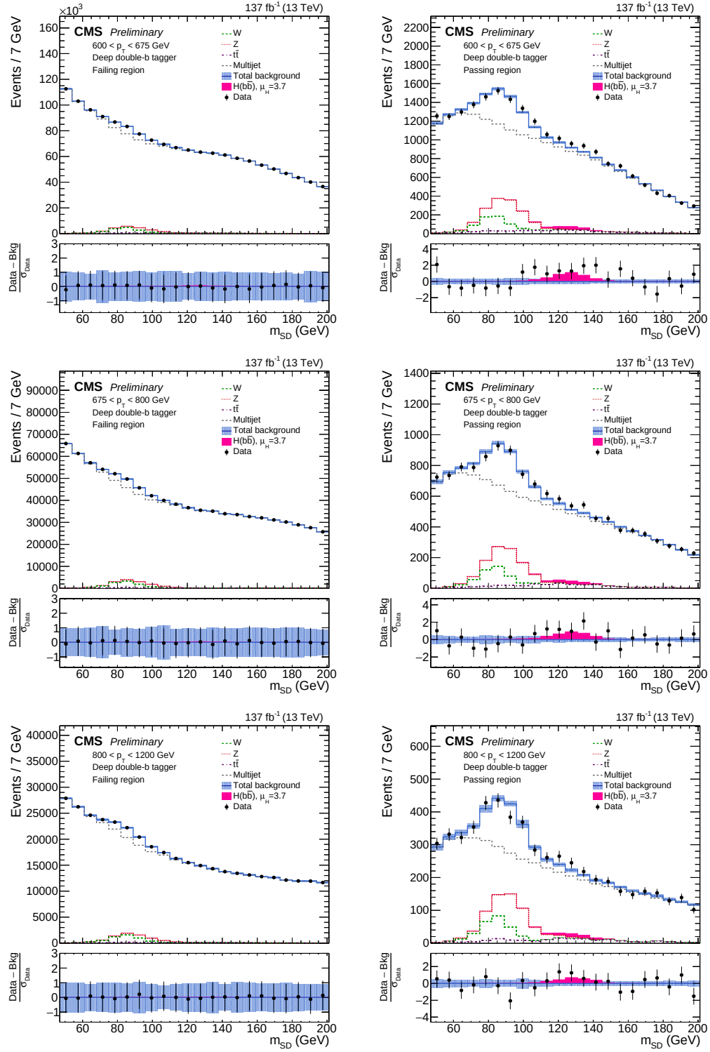
Figure 4.66: Post-fit m_{SD} distributions in the full 2016, 2017, and 2018 data set for the pass and fail regions and the second three p_T categories (600-675, 675-800, 800-1200 from top to bottom) summed over all three years. The EW and signal events are also shown separately.
