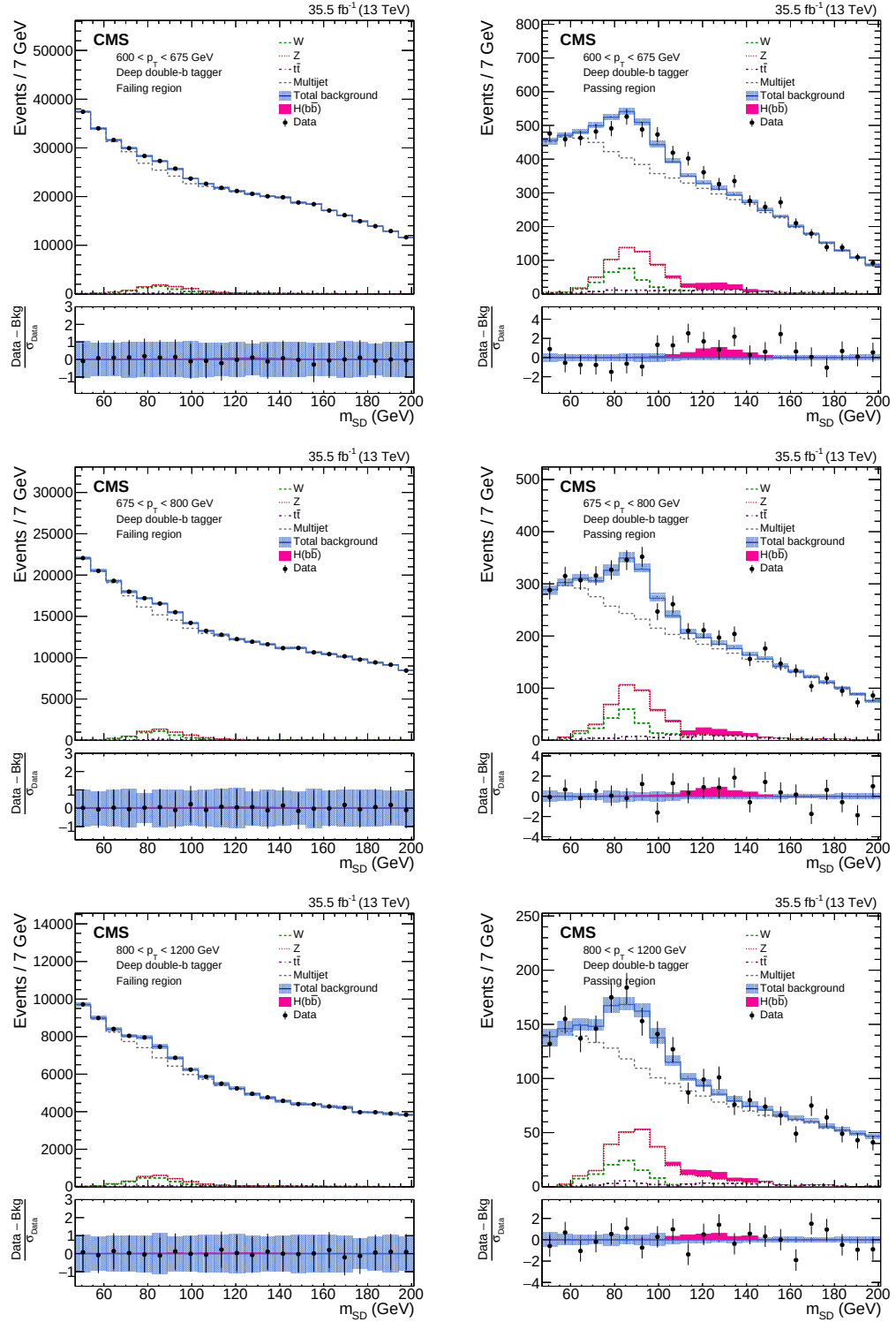
Figure B.2: Post-fit m_{SD} distributions in the full 2016 dataset for the pass and fail regions and the second three p_T categories (600-675, 675-800, 800-1200 from top to bottom) by using a polynomial 2nd order in \rho and 1st order in p_T . The EW and signal events are also shown separately.
