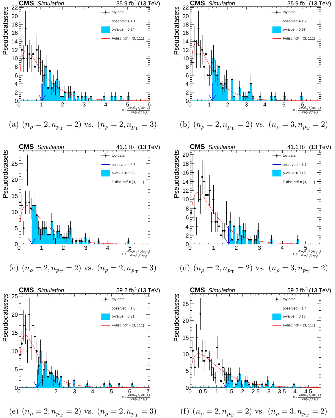
Figure 4.40: The F -test for different hypotheses on the MC (with \mu = 1 ), corresponding to the 2016(top), 2017(middle), 2018(bottom) dataset.
