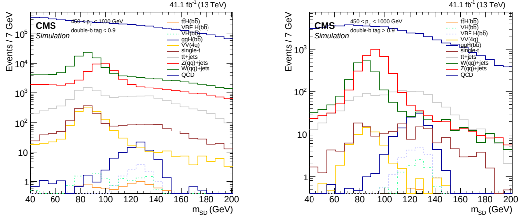
Figure 4.29: Signal region m_{SD} distribution for simulated signal and background events after all the selection criteria in both the failing (left) and passing (right) deep double-b tagging categories.
