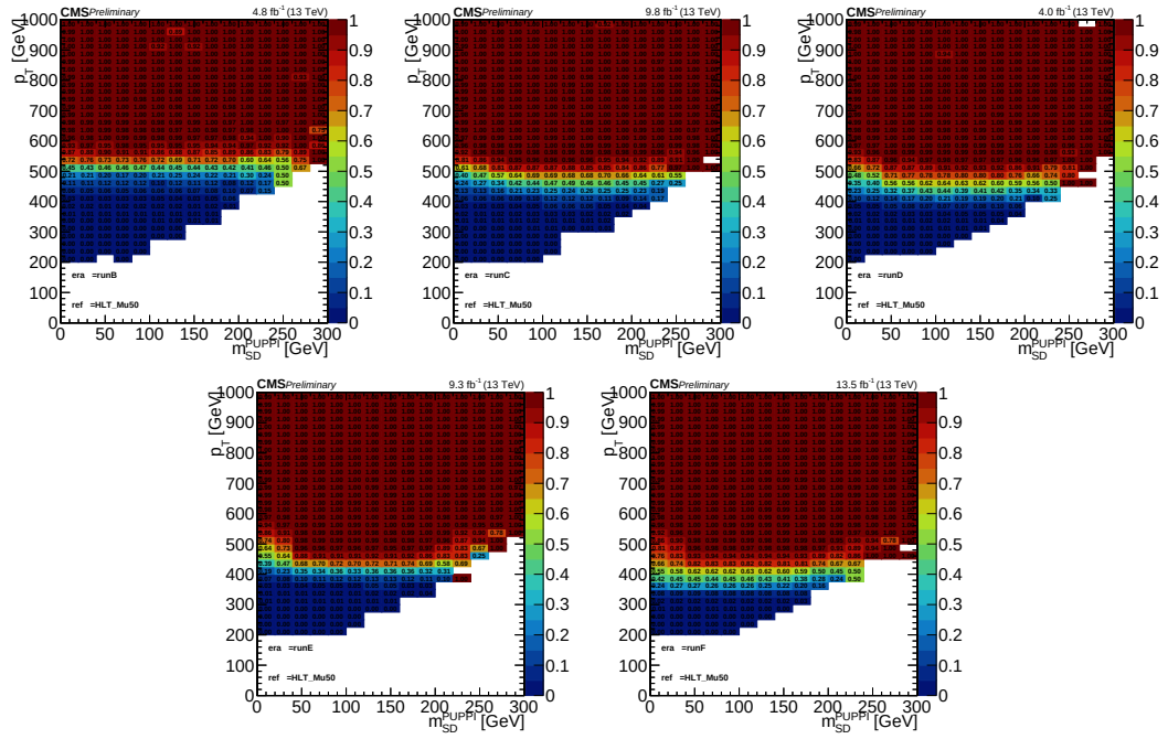
Figure 4.6: Measured trigger efficiency of the “OR” as function of jet p_T and jet m_{SD} is shown separately for each Run period in 2017.
