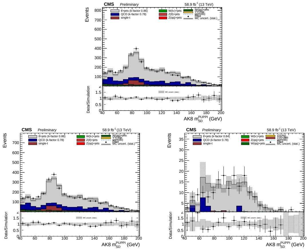
Figure 4.38: Single muon control region for t\bar{t} background in 2018 data. (Top) Inclusive in deep double-b tag. (Bottom left) Failing region with deep double-b tag < 0.89 . (Bottom right) Passing region with deep double-b tag > 0.89 . QCD is scaled down by a k-factor of 0.78 and t\bar{t} is scaled to same integral as data.
