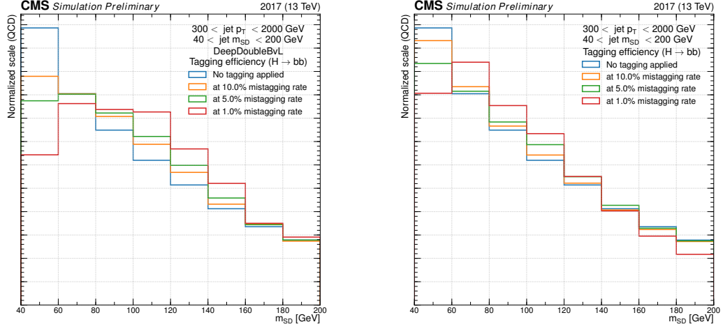
Figure 4.20: Mass sculpting for deep double-b without (left) and with (right) mass decorrelation.
