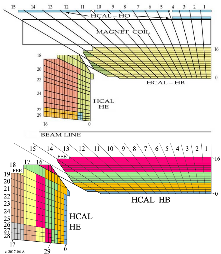
Figure 3.11: Depth segmentation of CMS HCAL before (top) and after (bottom) Phase-1 upgrade [37, 41].
