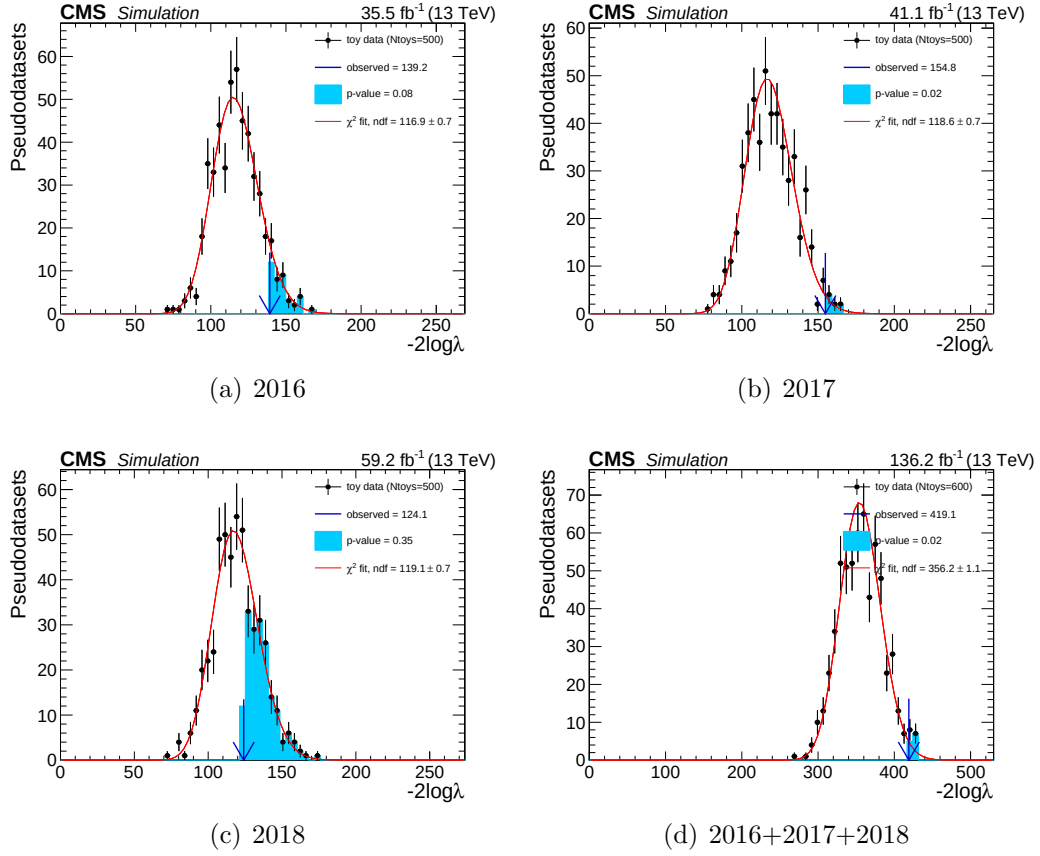
Figure 4.70: Results of the goodness-of-fit test for the full (a) 2016 data set, (b) 2017 data set, (c) 2018 data set and (d) full Run 2 data set using the saturated test statistic. The order of polynomial used are second(first) order in \rho and first(first) order in p_T for all 2016(2017,2018) data sets.
