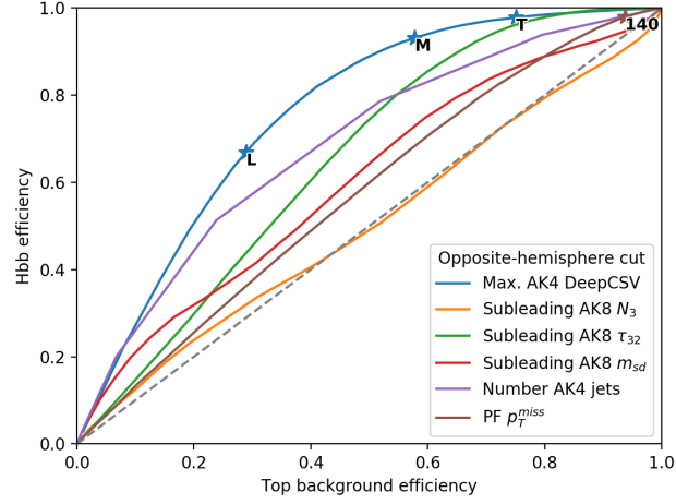
Figure 4.22: ROC curves for different t\bar{t} sensitive variables.
