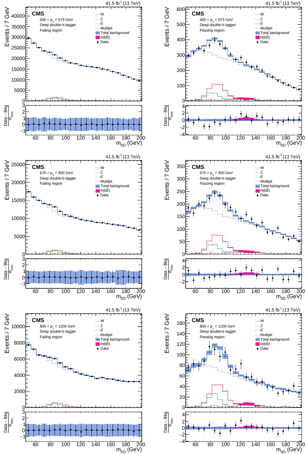
Figure B.4: Post-fit m_{SD} distributions in the full 2017 dataset for the pass and fail regions and the second three p_T categories (600-675, 675-800, 800-1200 from top to bottom) by using a polynomial 1st order in \rho and 1st order in p_T . The EW and signal events are also shown separately.
