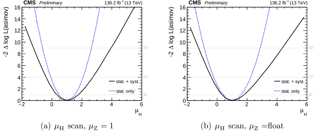
Figure 4.71: 1D profile test statistic -2\Delta\log(\mathcal{L}) scans as a function of the signal strengths \mu_H , fixing \mu_Z = 1 (left) and floating \mu_Z (right), with Asimov data set for 2016+2017+2018. The solid black curve, labeled “stat+syst,” corresponds to the scan when profiling all nuisance parameters and the dotted blue curve, labeled “stat only,” corresponds to only profiling the unconstrained nuisance parameters, such as the QCD transfer factor parameters.
