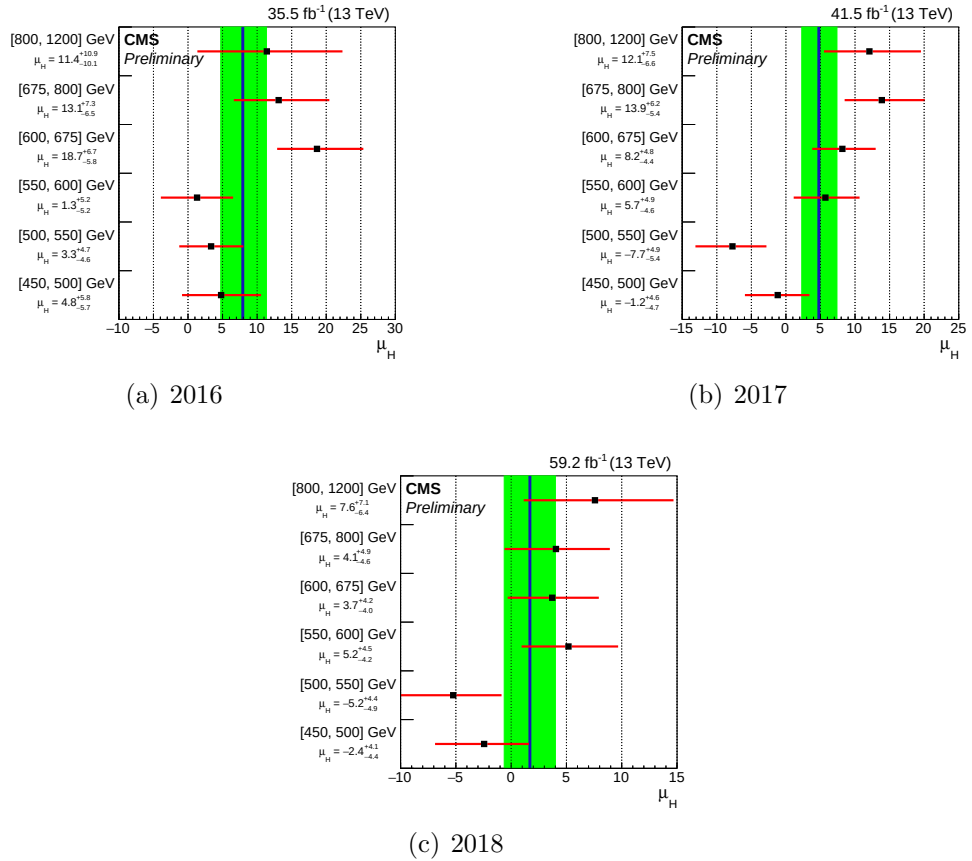
Figure 4.73: The best-fit H signal strength \mu_H and uncertainty per p_T category extracted from a simultaneous fit of all channels, performed on different data taking periods.
