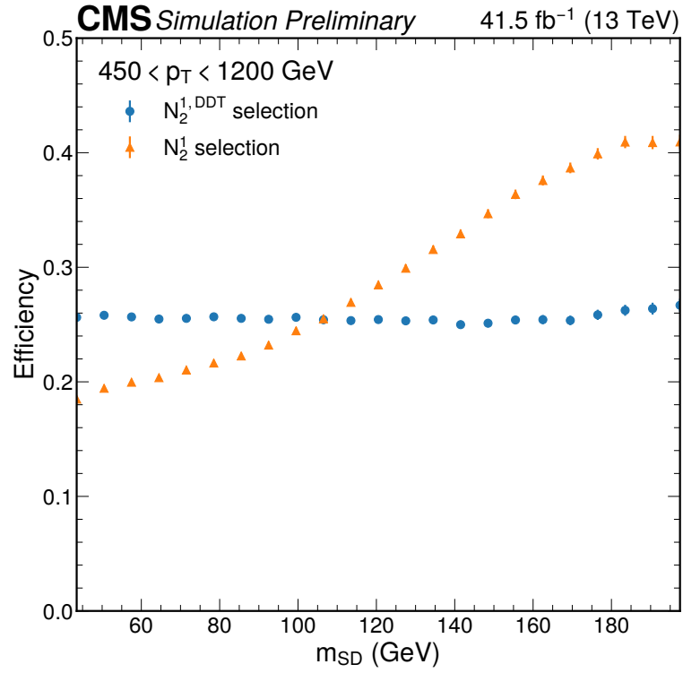
Figure 4.15: Comparison between N_2^{1,DDT} and N_2^1 efficiency as a function of m_{SD} with QCD simulation. The cut on N_2^1 corresponds to same overall efficiency of 26% in the analysis phase space.
