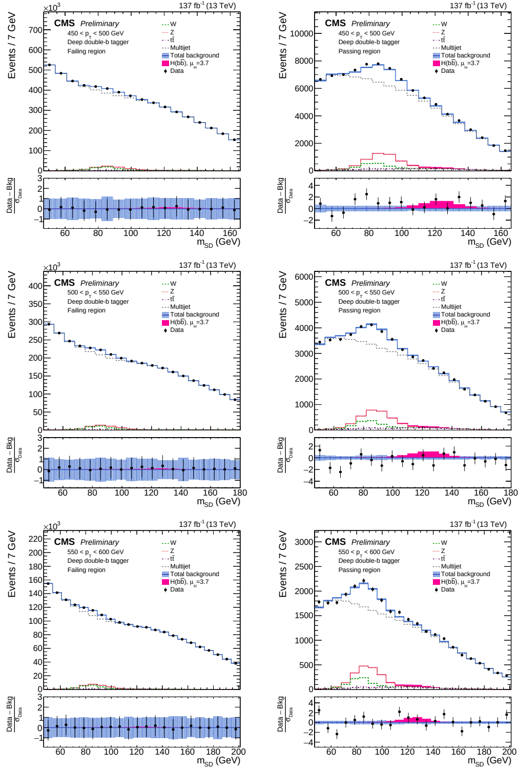
Figure 4.65: Post-fit m_{SD} distributions in the full 2016, 2017, and 2018 data set for the pass and fail regions and the first three p_T categories (450-500, 500-550, 550-600 from top to bottom) summed over all three years. The EW and signal events are also shown separately.
