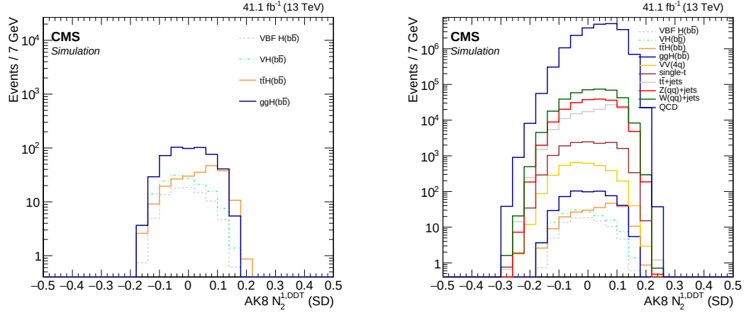
Figure 4.18: N_2^{1,DDT} distribution for the p_T -leading jet. Left, simulated signal events normalized to their cross sections (Table 4.4). Right, background and signal events normalized to their cross sections.
