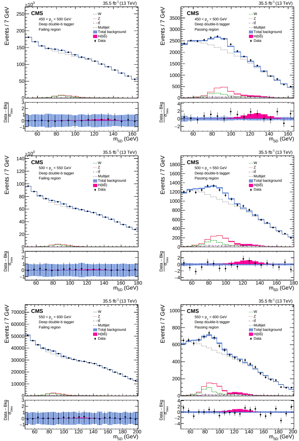
Figure B.1: Post-fit m_{SD} distributions in the full 2016 dataset for the pass and fail regions and the first three p_T categories (450-500, 500-550, 550-600 from top to bottom) by using a polynomial 2nd order in \rho and 1st order in p_T . The EW and signal events are also shown separately.
