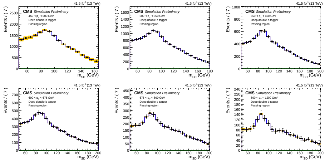
Figure 4.52: Empirical function signal+background fit to the pass category directly with the 2017 MC.
