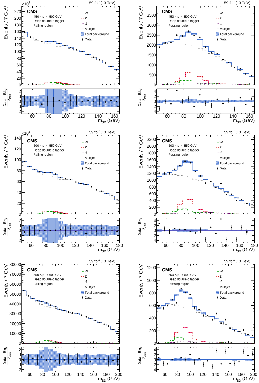
Figure 4.48: Post-fit m_{SD} distributions in simulated MC events corresponding to 2018 conditions for the pass and fail regions and the first three p_T categories (450-500, 500-550, 550-600 from top to bottom) by using a polynomial 2nd order in \rho and 2nd order in p_T . The EW and signal events are also shown separately.
