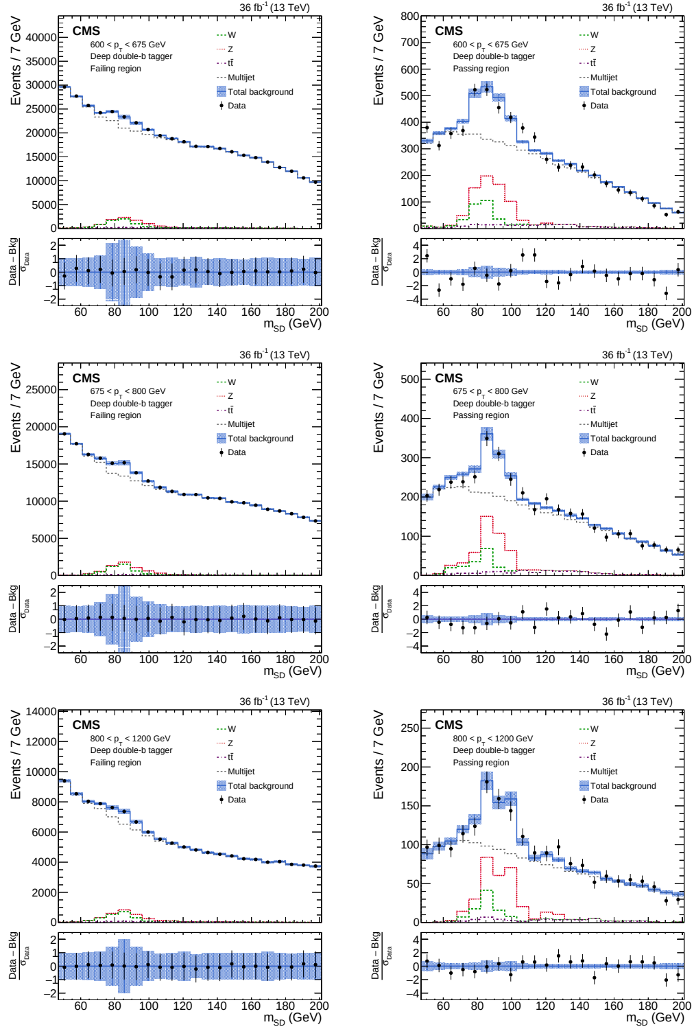
Figure 4.45: Post-fit m_{SD} distributions in simulated MC events corresponding to 2016 conditions for the pass and fail regions and the second three p_T categories (600-675, 675-800, 800-1200 from top to bottom) by using a polynomial 2nd order in \rho and 2nd order in p_T . The EW and signal events are also shown separately.
