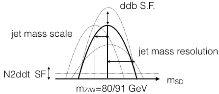
Figure 4.33: Schematic drawing of the effect of data-MC corrections factors applied on W/Z+jets backgrounds.
