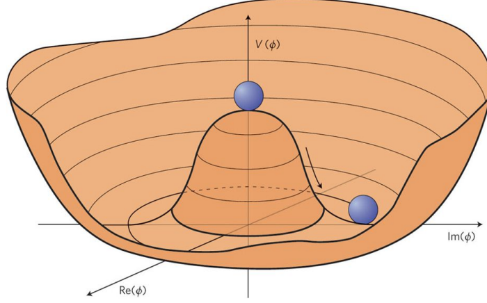
Figure 2.2: Sketch of the Higgs potential V(\phi) [10].
