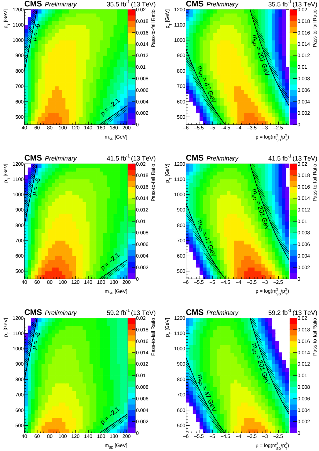
Figure 4.43: The fitted pass-fail ratio \epsilon^{\text{QCDMC}} as a function of p_T and m_{SD} (left) or p_T and \rho (right) for QCD MC corresponding to conditions in 2016 (top), 2017 (middle), and 2018 (bottom).
