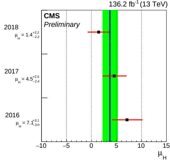
Figure 4.75: The best-fit signal strength \mu_H and uncertainty per year, extracted from a simultaneous fit of all channels.
