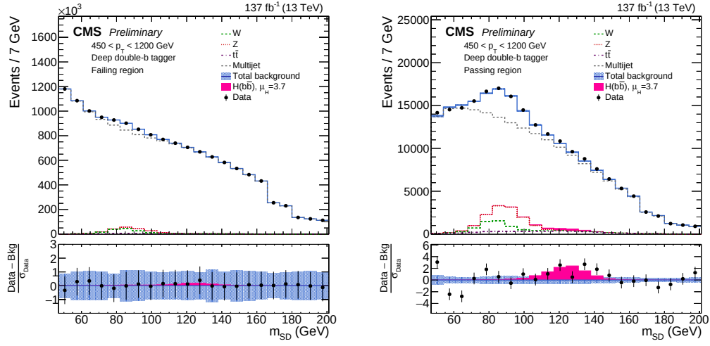
Figure 4.67: Post-fit m_{SD} distributions in the full Run II data set for the pass and fail regions. The EW and signal events are also shown separately.
