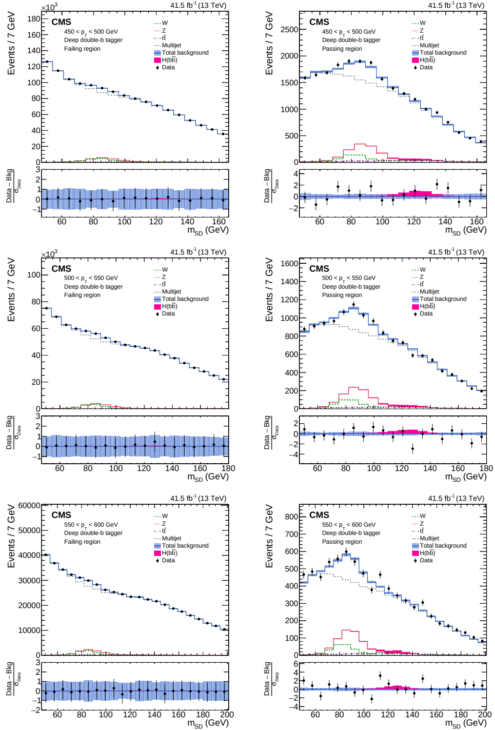
Figure B.3: Post-fit m_{SD} distributions in the full 2017 dataset for the pass and fail regions and the first three p_T categories (450-500, 500-550, 550-600 from top to bottom) by using a polynomial 1st order in \rho and 1st order in p_T . The EW and signal events are also shown separately.
